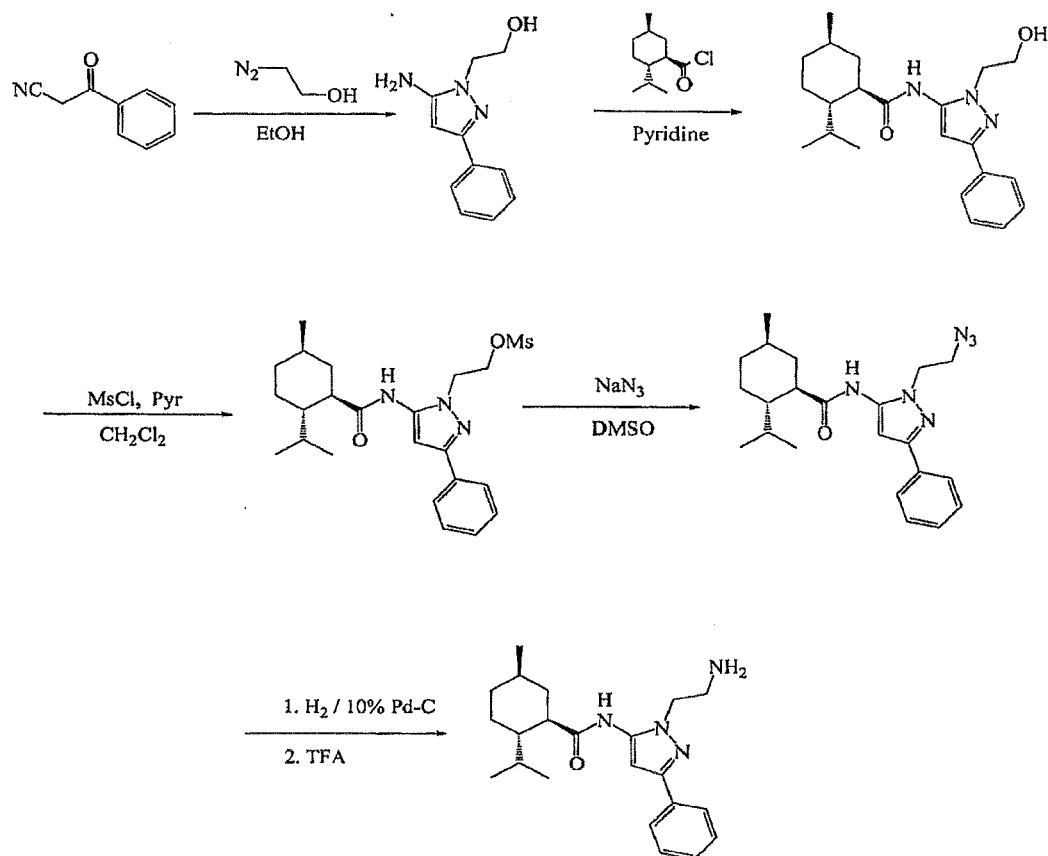
Scheme 5.
