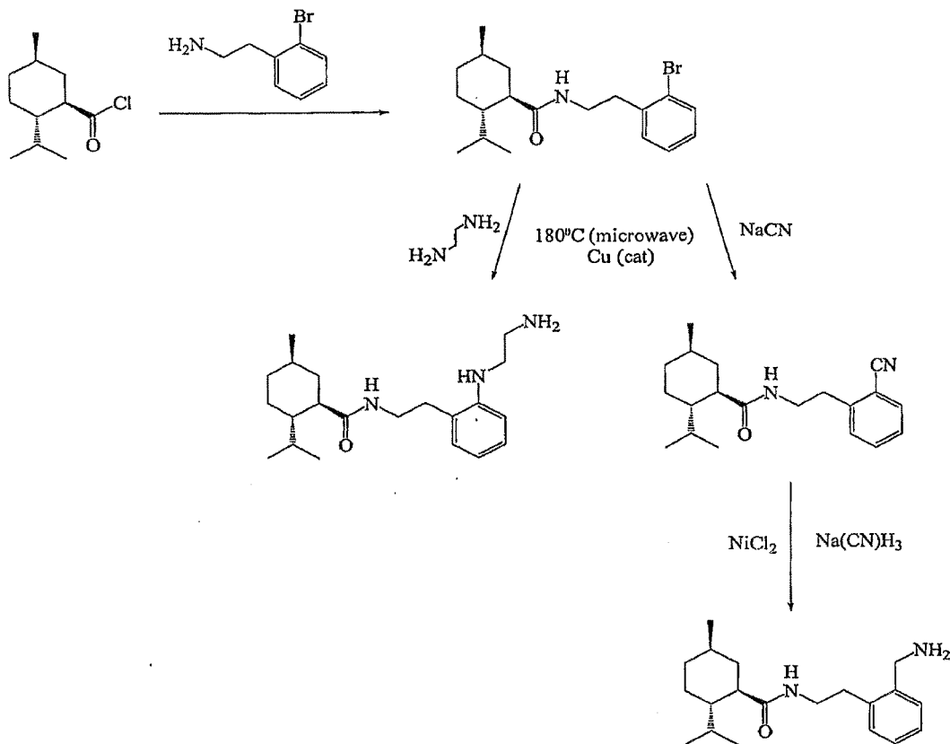
Scheme 7.
