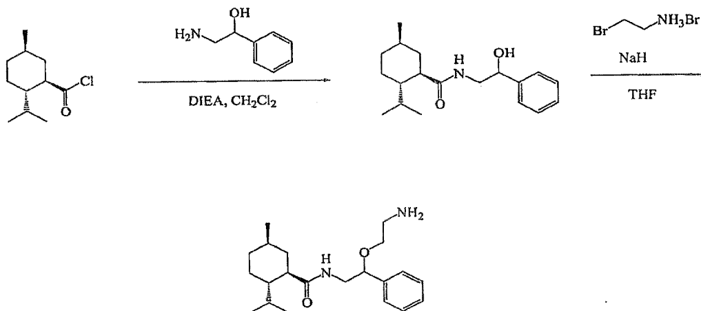
Scheme 6.
