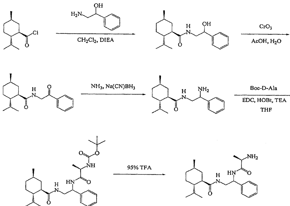
Scheme 7.
