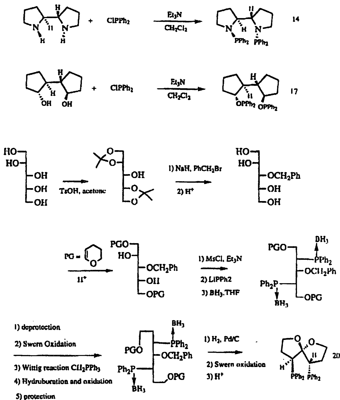
Figure 9. Synthesis of new chiral ligands 14-23.
