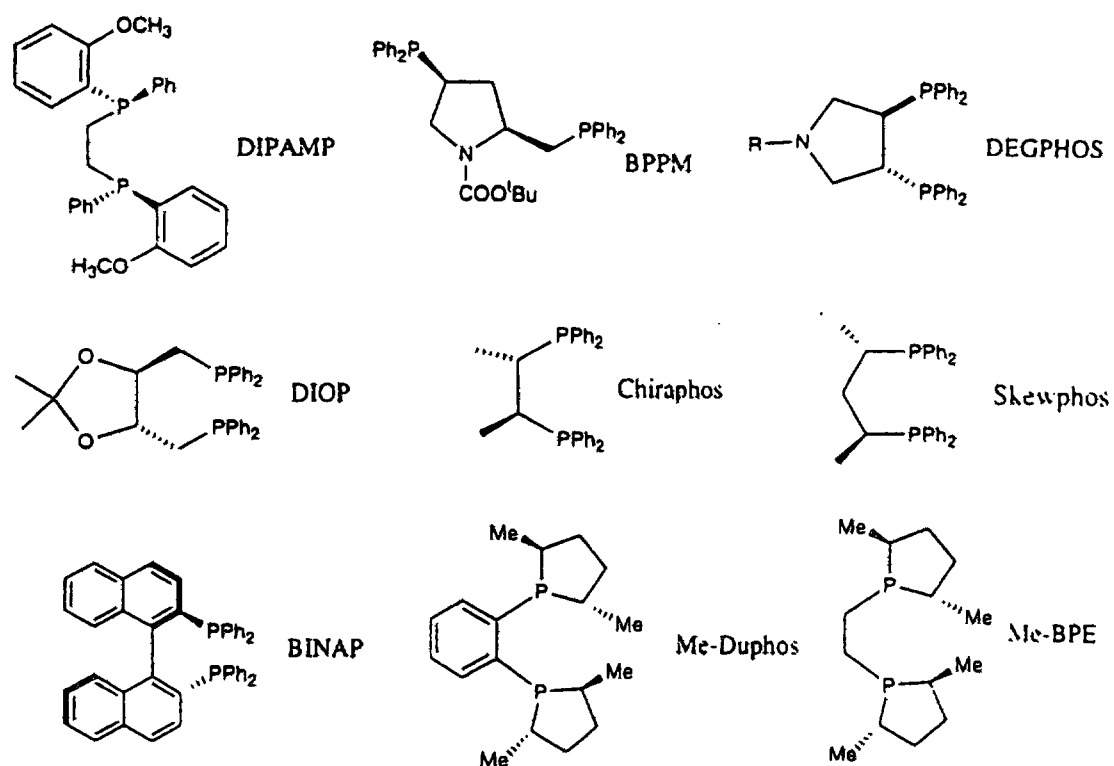
Figure 1. Chiral bidentate phosphine ligands
