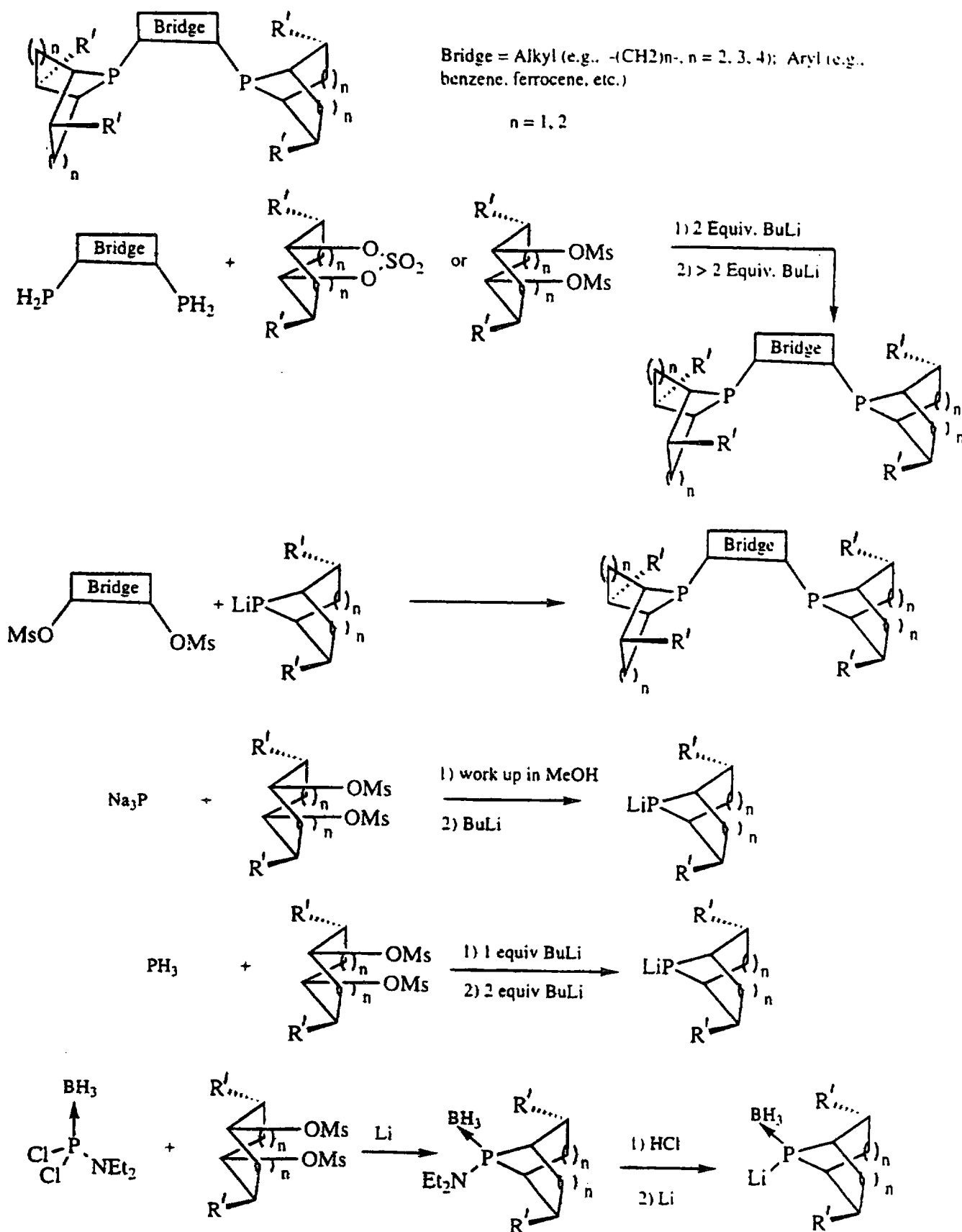
Figure 11 Synthesis of Bidentate Cyclic Phosphines (ligands 35-39)
