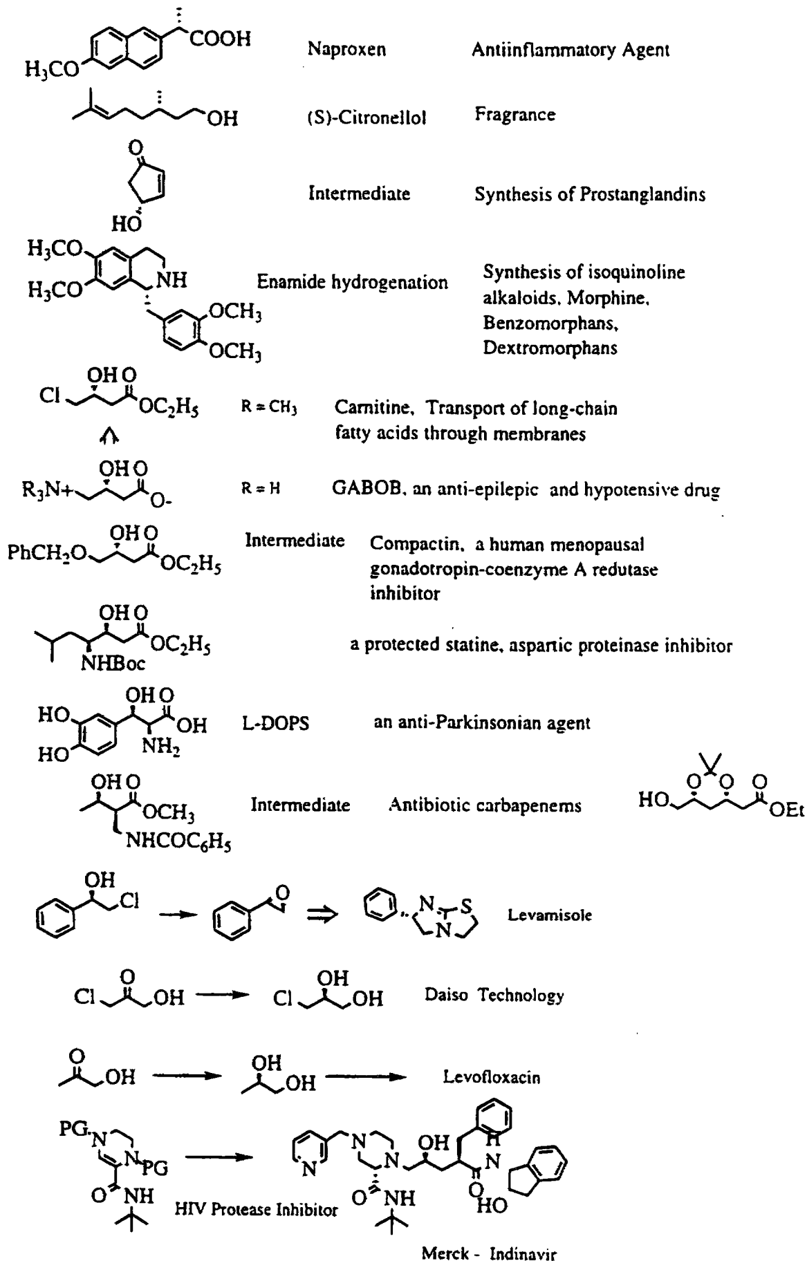
Figure 1 Some Applications of Asymmetric Catalytic Reactions
