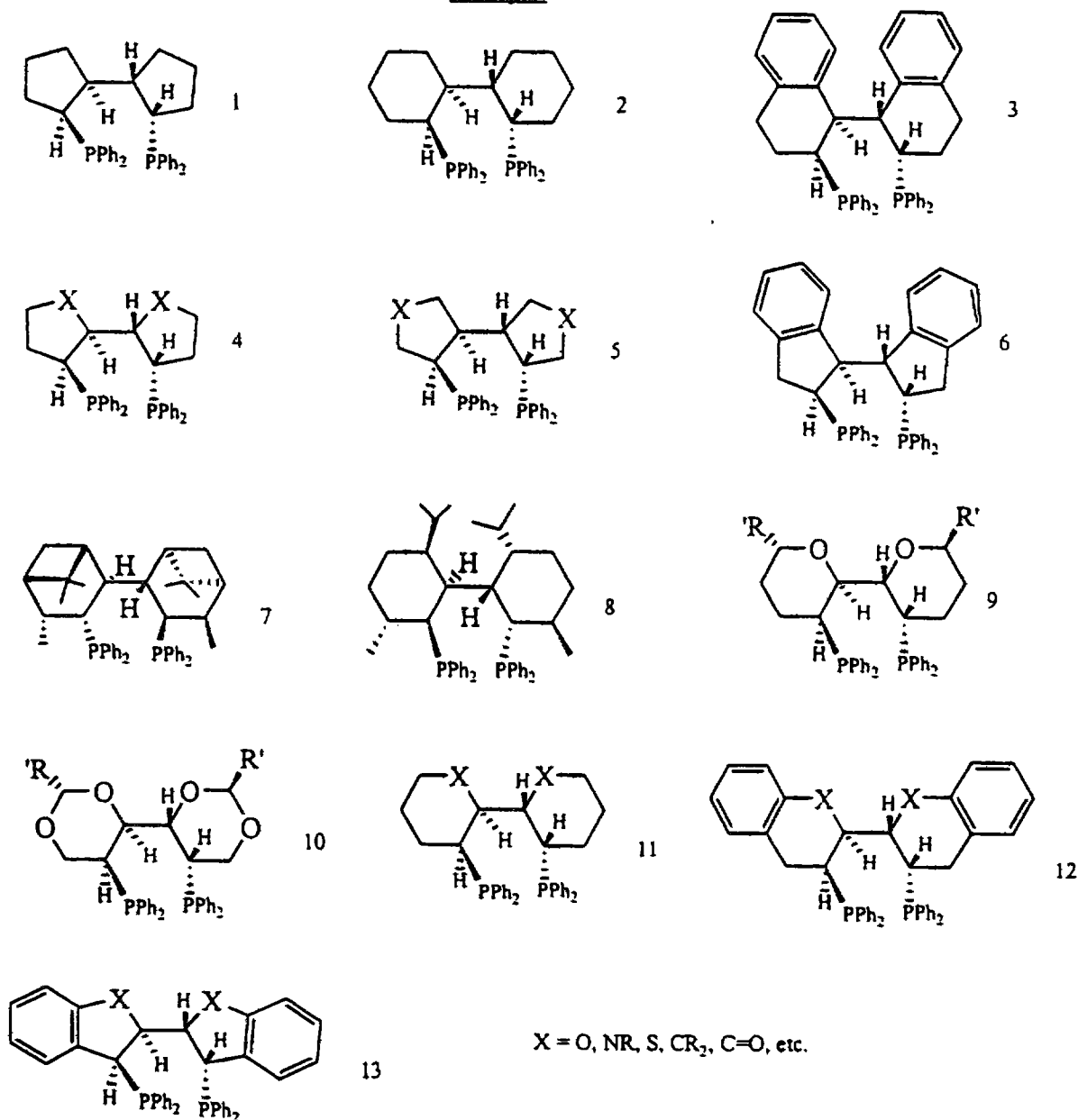
Figure 2. Selected New phosphine ligands with ring structures
