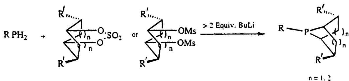
Figure 12 Synthesis of Bidentate Cyclic Phosphines (ligands 40-44)
