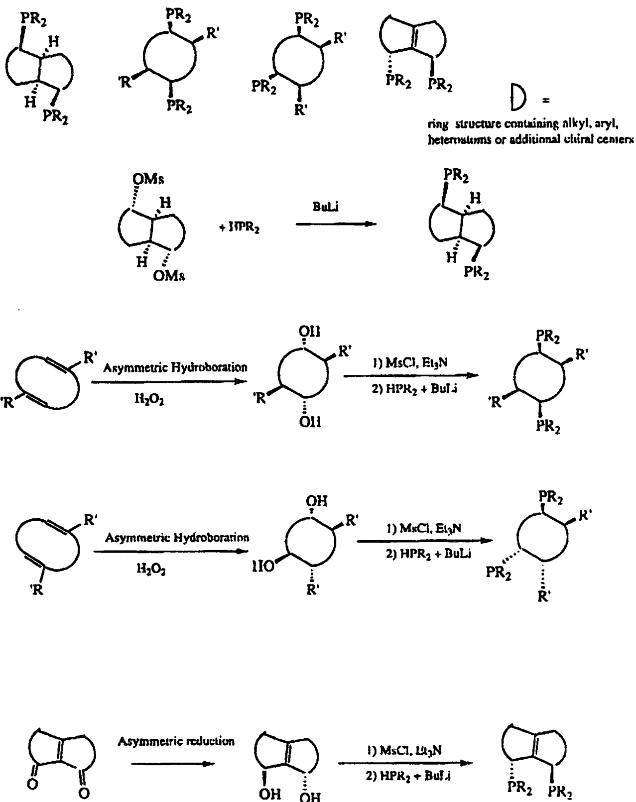
Figure 13. Synthesis of Bidentate Cyclic Phosphines (Ligands 45-49)
