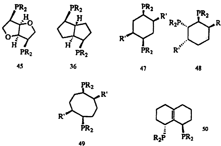
Figure 7. Selected new phosphine ligands with ring structures
