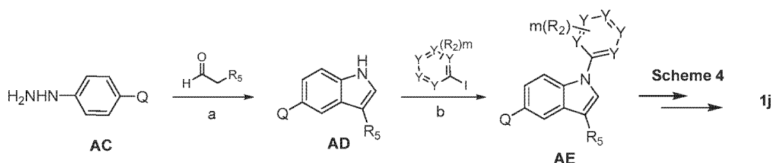
Scheme 6. Reagents and conditions: a) AcOH, 120 °C; b) Cu(I)Br, Cu(OAc) 2 , K 2 CO 3 , NaOH, 140 °C.
