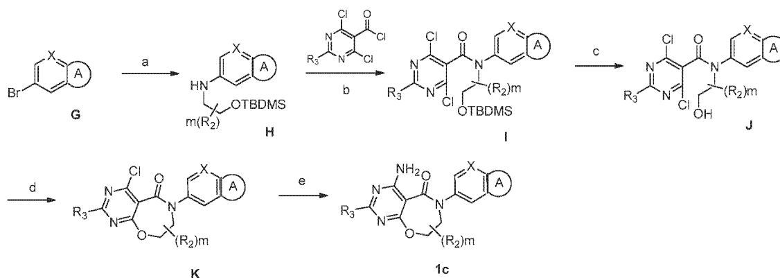
Scheme 2. Reagents and conditions: a) \text{NH}_2(\text{CH}_2)_2\text{OTBDMS} , \text{Pd}(\text{OAc})_2 , \text{Cs}_2\text{CO}_3 , X-PHOS, Toluene, 120 °C; b) THF, \text{Et}_3\text{N} , RT; c) 3% HCl-MeOH, RT; d) \text{CH}_3\text{CN} , \text{Et}_3\text{N} , 80 °C; e) \text{NH}_3 , Dioxane, RT.
