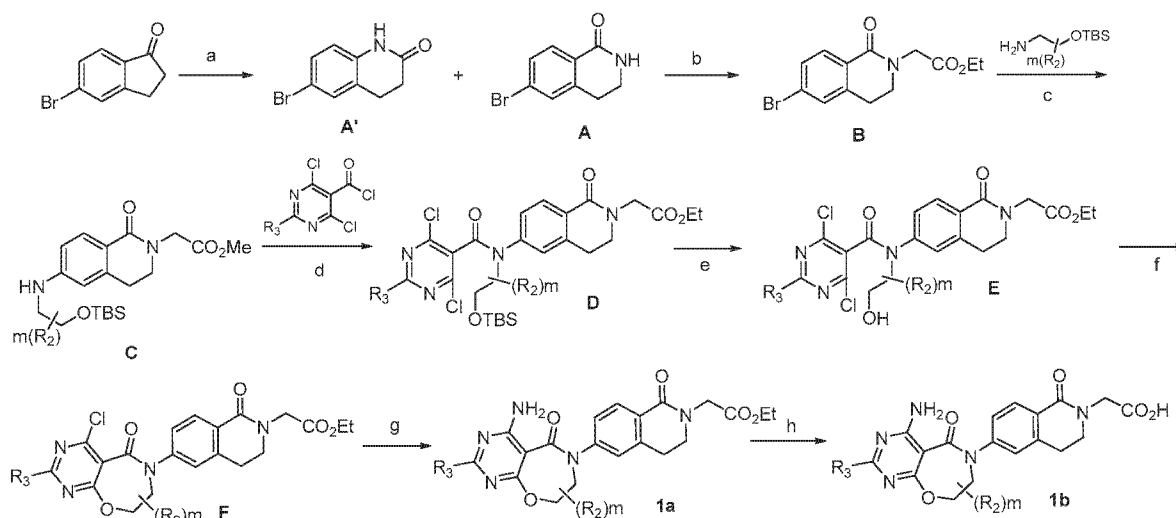
Scheme 1. Reagents and conditions: a) \text{NaN}_3 , \text{MeSO}_3\text{H} , \text{CH}_2\text{Cl}_2 , RT; b) \text{NaH} , \text{BrCH}_2\text{CO}_2\text{Et} , THF, RT; c) \text{Pd}(\text{OAc})_2 , \text{Cs}_2\text{CO}_3 , X-Phos, Toluene, 120^\circ\text{C} ; d) THF, \text{Et}_3\text{N} , RT; e) 3% \text{HCl} -MeOH, RT; f) \text{CH}_3\text{CN} , \text{Et}_3\text{N} , 80^\circ\text{C} ; g) \text{NH}_3 , Dioxane, RT; h) \text{LiOH} , Dioxane- \text{H}_2\text{O} , RT
