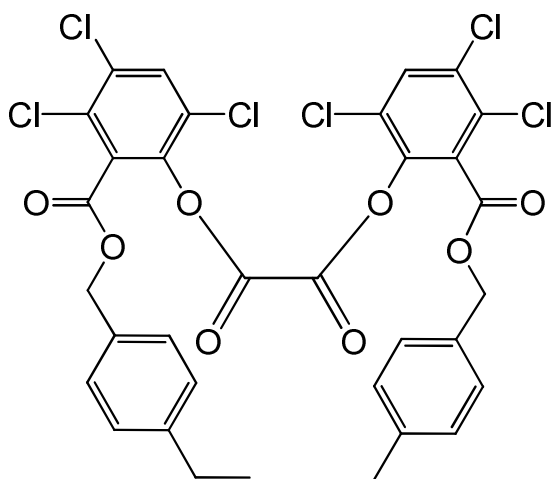
bis(3,4,6-trichloro-2-[[4-ethylphenyl)methoxy]carbonyl}phenyl) oxalate
