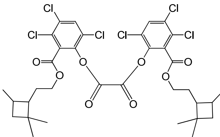
bis(3,4,6-trichloro-2-([2-(2,2,4-trimethylcyclobutylethoxy)carbonyl]phenyl) oxalate
