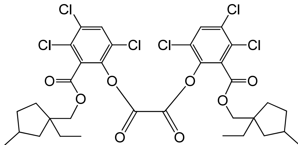
bis(3,4,6-trichloro-2-[(1-ethyl-3-methylcyclopentyl)methoxy]carbonyl)phenyl oxalate
