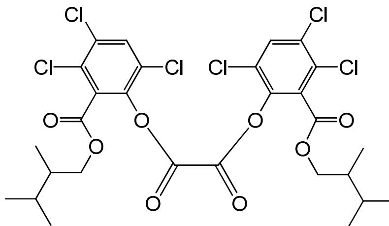
bis{3,4,6-trichloro-2-[(2,3-dimethylbutoxy)carbonyl]phenyl} oxalate
