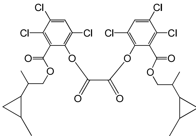
bis(3,4,6-trichloro-2-[(2-(2-methylcyclopropyl)propoxy)carbonyl]phenyl) oxalate
