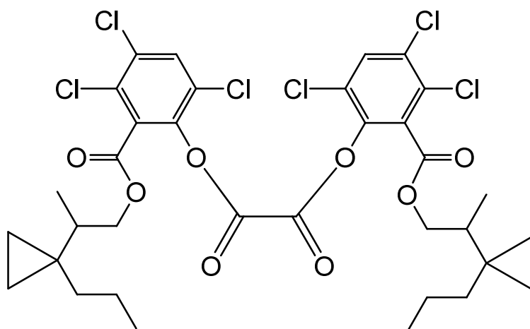
bis(3,4,6-trichloro-2-{[2-(1-propylcyclopropyl)propoxy]carbonyl}phenyl) oxalate
