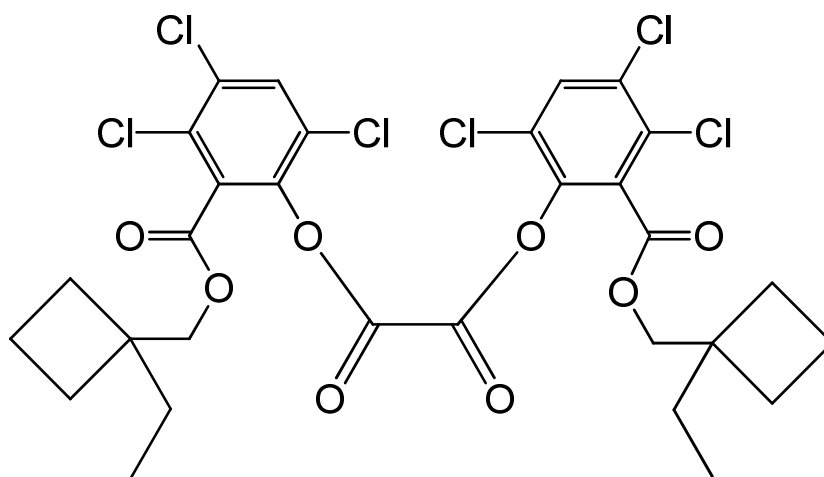
bis(3,4,6-trichloro-2-[[1-ethylcyclobutyl)methoxy]carbonyl]phenyl) oxalate
