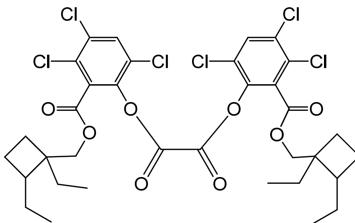
bis(3,4,6-trichloro-2-[[1,2-diethylcyclobutyl)methoxy]carbonyl)phenyl) oxalate
