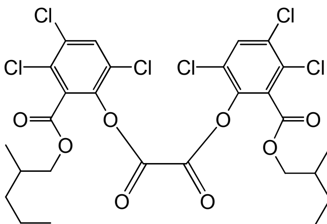
bis{3,4,6-trichloro-2-[(2-methylpentyloxy)carbonyl]phenyl} oxalate
