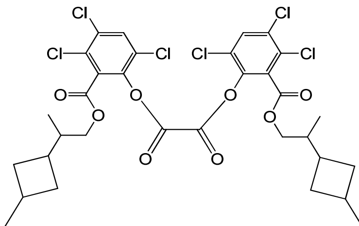
bis(3,4,6-trichloro-2-([2-(3-methylcyclobutyl)propoxy]carbonyl)phenyl) oxalate
