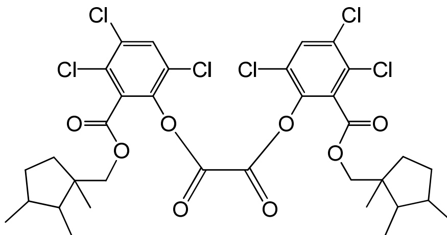
bis(3,4,6-trichloro-2-[[1,2,3-trimethylcyclopentyl)methoxy]carbonyl}phenyl) oxalate
