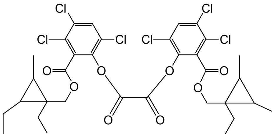
bis(3,4,6-trichloro-2-[(1,2-diethyl-3-methylcyclopropyl)methoxy]carbonyl)phenyl oxalate
