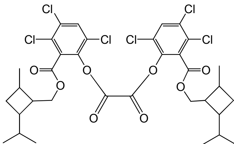
bis[3,4,6-trichloro-2-({[2-methyl-4-(1-methylethyl)cyclobutyl]methoxy}carbonyl)phenyl] oxalate
