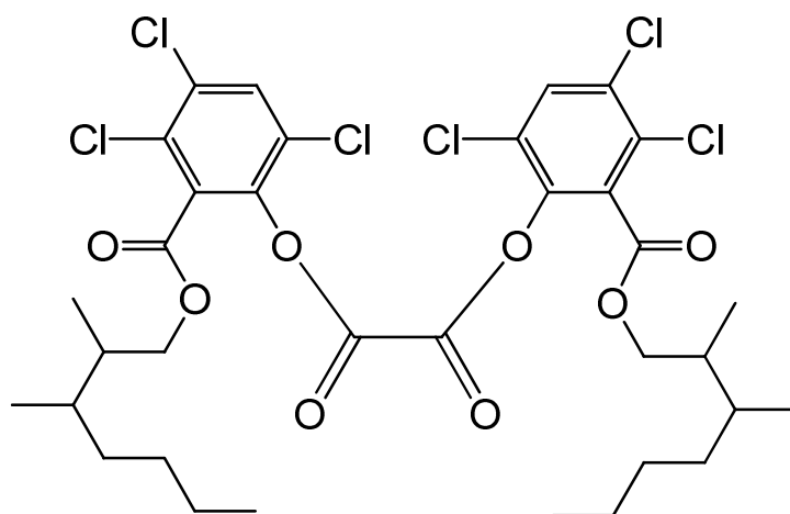
bis{3,4,6-trichloro-2-[(2,3-dimethylheptyloxy)carbonyl]phenyl} oxalate
