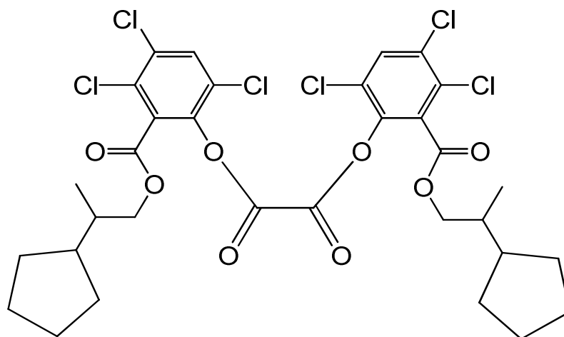
bis{3,4,6-trichloro-2-[(2-cyclopentylpropoxy)carbonyl]phenyl} oxalate
