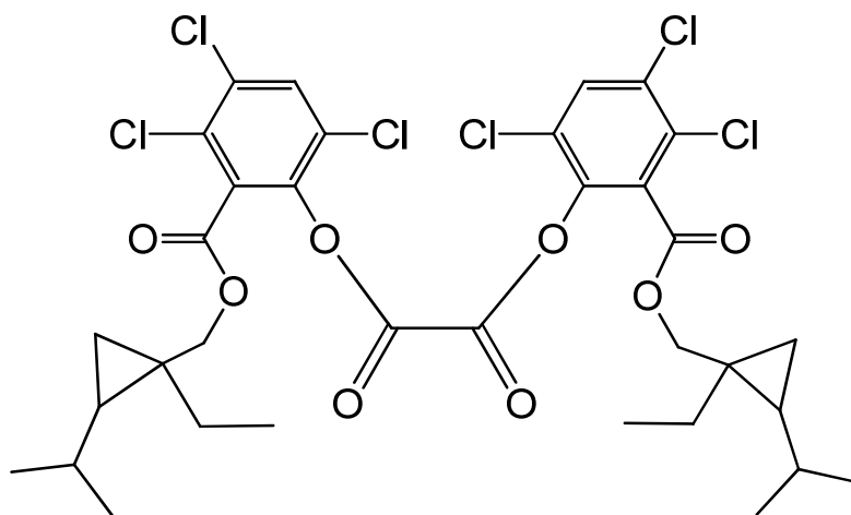
bis[3,4,6-trichloro-2-([1-ethyl-2-(1-methylethyl)-cyclopropyl]methoxy)carbonyl]phenyl] oxalate
