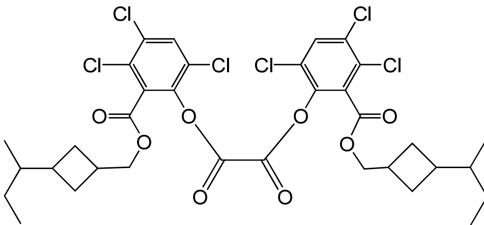
bis[3,4,6-trichloro-2-({[3-(1-methylpropyl)cyclobutyl]methoxy}carbonyl)phenyl] oxalate
