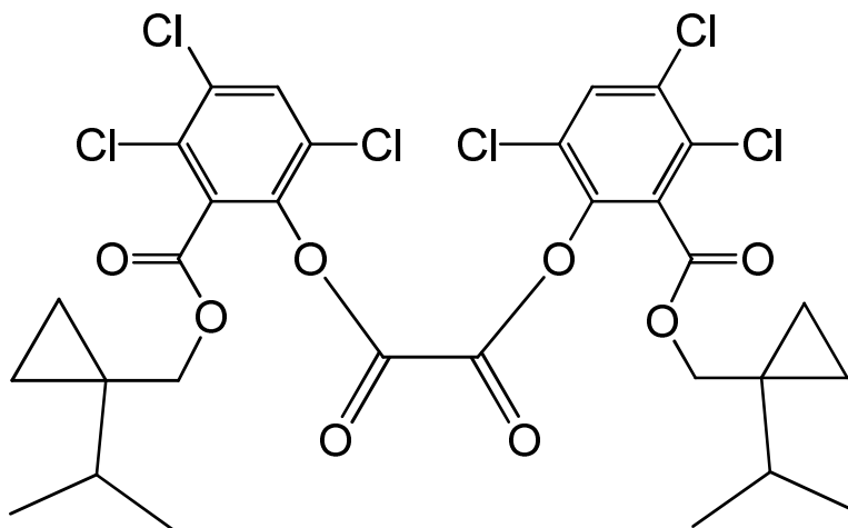
bis[3,4,6-trichloro-2-([1-(1-methyl-ethyl)cyclopropyl]methoxy)carbonyl]phenyl] oxalate
