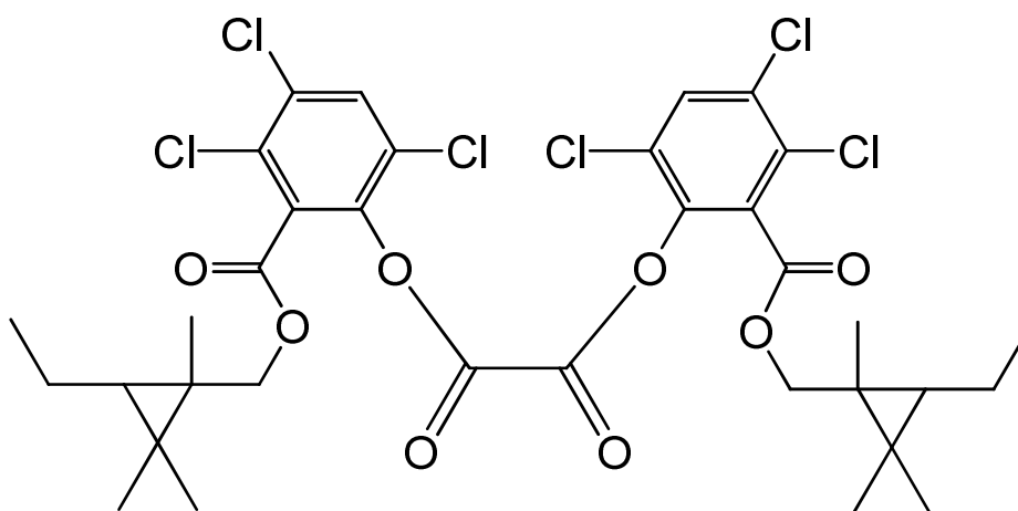
bis(3,4,6-trichloro-2-[[3-ethyl-1,2,2-trimethylcyclopropyl)methoxy]carbonyl}phenyl) oxalate
