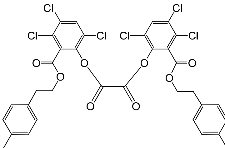
bis(3,4,6-trichloro-2-{[2-(4-methylphenyl)ethoxy]carbonyl}phenyl) oxalate
