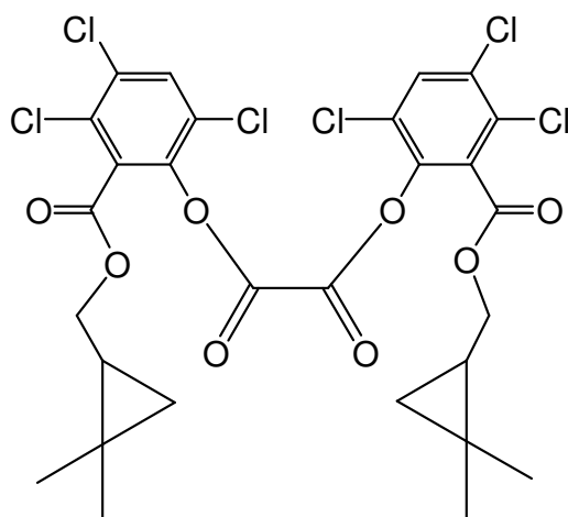
bis(3,4,6-trichloro-2-[[2-(2,2-dimethylcyclopropyl)methoxy]carbonyl]phenyl) oxalate
