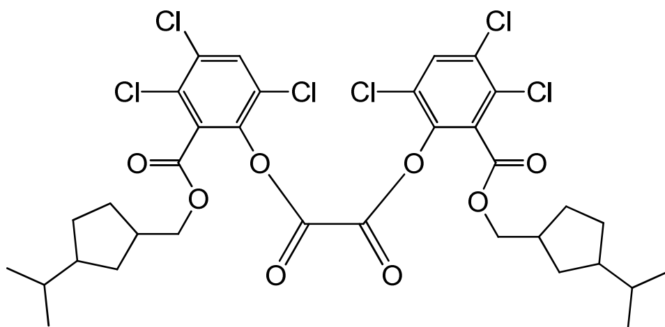
bis[3,4,6-trichloro-2-({[3-(1-methylethyl)-cyclopentyl]methoxy}carbonyl)phenyl] oxalate
