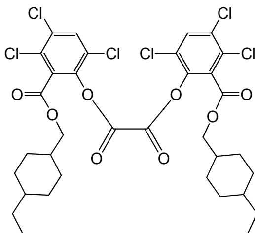
bis(3,4,6-trichloro-2-[[4-ethylcyclohexyl]methoxy]carbonyl)phenyl oxalate
