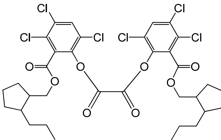
bis(3,4,6-trichloro-2-{[(2-propylcyclopentyl)methoxy]carbonyl}phenyl) oxalate
