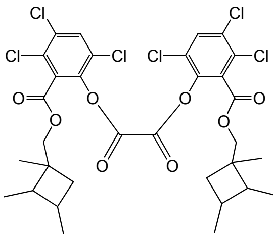
bis(3,4,6-trichloro-2-{[(1,2,3-trimethylcyclobutyl)methoxy]carbonyl}phenyl) oxalate
