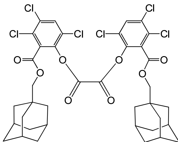
bis{3,4,6-trichloro-2-[(1-adamantylmethoxy)carbonyl]phenyl} oxalate
