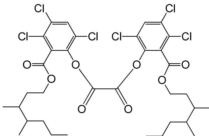
bis{3,4,6-trichloro-2-[(3,4-dimethylheptyloxy)carbonyl]phenyl} oxalate
