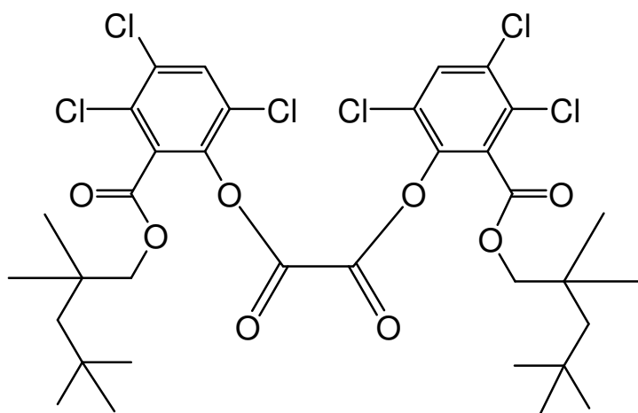
bis{3,4,6-trichloro-2-[(2,2,4,4-tetramethylpentyloxy)carbonyl]phenyl} oxalate
