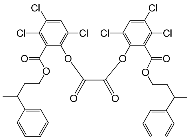
bis{3,4,6-trichloro-2-[(3-phenylbutoxy)carbonyl]phenyl} oxalate
