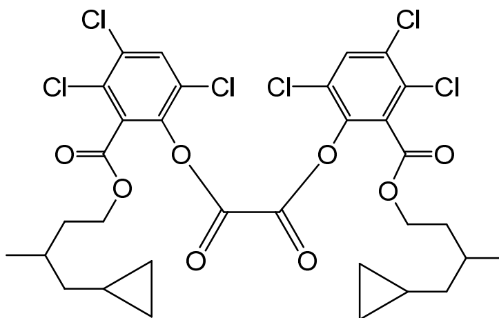
bis{3,4,6-trichloro-2-[(4-cyclopropyl-3-methylbutoxy)carbonyl]phenyl} oxalate
