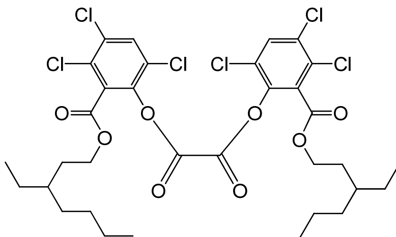
bis{3,4,6-trichloro-2-[(3-ethylheptyloxy)carbonyl]phenyl} oxalate
