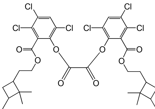
bis(3,4,6-trichloro-2-{[2-(2,2,3-trimethylcyclobutyl)ethoxy]carbonyl}phenyl) oxalate
