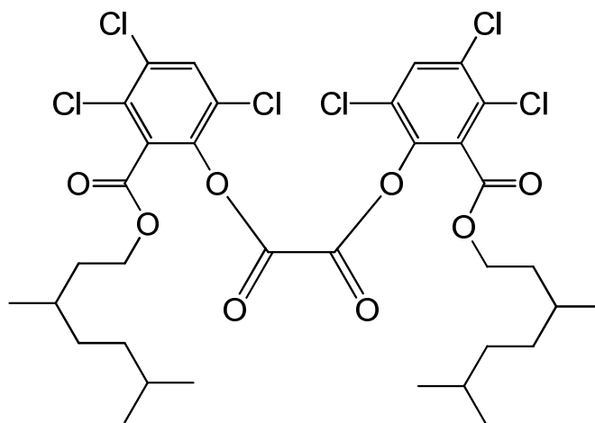
bis{3,4,6-trichloro-2-[(3,6-dimethylheptyloxy)carbonyl]phenyl} oxalate
