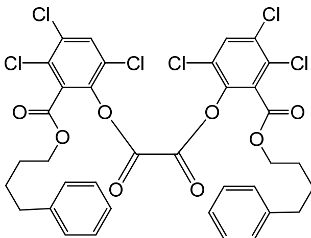
bis{3,4,6-trichloro-2-[(4-phenylbutoxy)carbonyl]phenyl} oxalate
