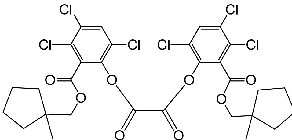
bis(3,4,6-trichloro-2-[(1-methylcyclopentyl)methoxy]carbonyl)phenyl oxalate
