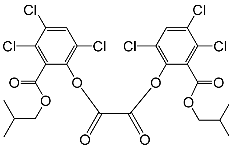
bis{3,4,6-trichloro-2-[(2-methylpropoxy)carbonyl]phenyl} oxalate
