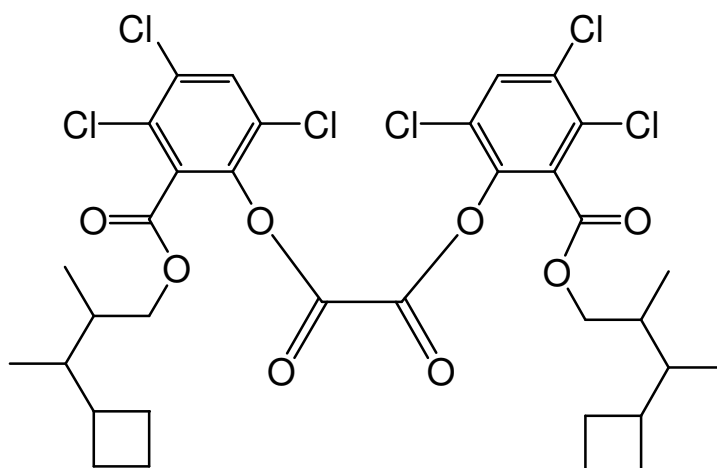
bis{3,4,6-trichloro-2-[(3-cyclobutyl-2-methylbutoxy)carbonyl]phenyl} oxalate
