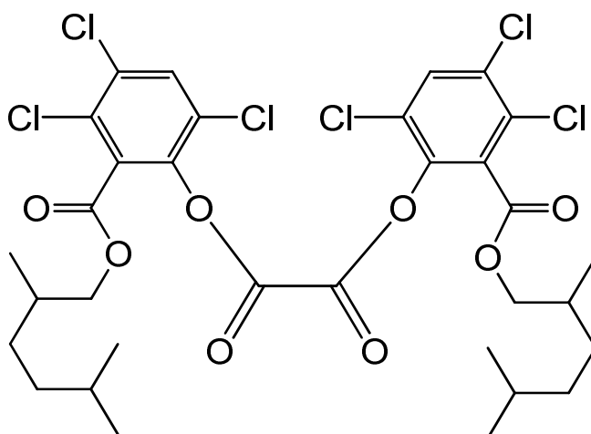
bis{3,4,6-trichloro-2-[(2,5-dimethylhexyloxy)carbonyl]phenyl} oxalate
