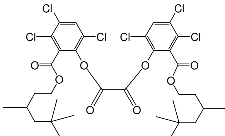
bis{3,4,6-trichloro-2-[(3,5,5-trimethylhexyloxy)carbonyl]phenyl} oxalate
