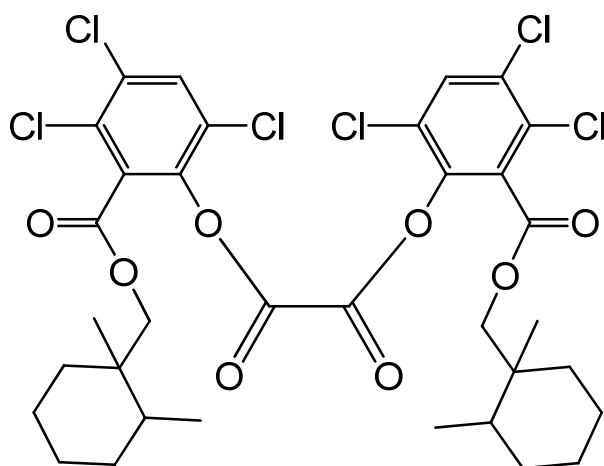
bis(3,4,6-trichloro-2-[[1,2-dimethylcyclohexyl)methoxy]carbonyl]phenyl) oxalate
