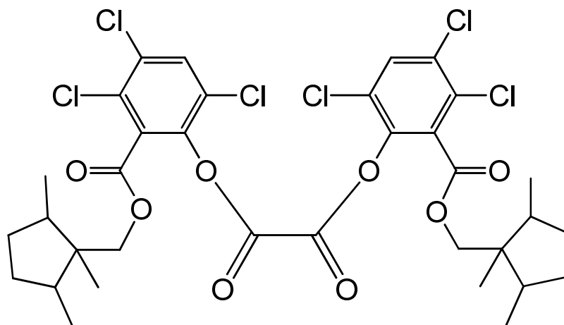
bis(3,4,6-trichloro-2-[(1,2,5-trimethylcyclopentyl)methoxy]carbonyl)phenyl) oxalate
