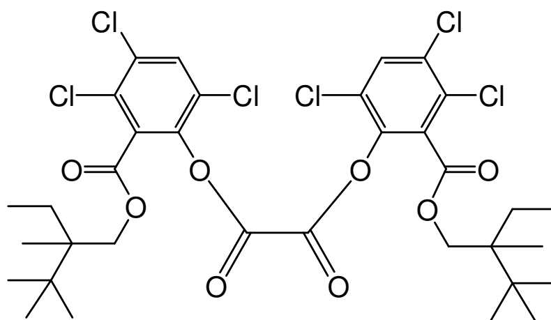
bis{3,4,6-trichloro-2-[(2-ethyl-2,3,3-trimethylbutoxy)carbonyl]phenyl} oxalate
