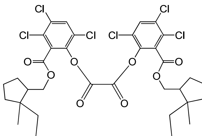
bis(3,4,6-trichloro-2-[(2-ethyl-2-methylcyclopentyl)methoxy]carbonyl)phenyl) oxalate
