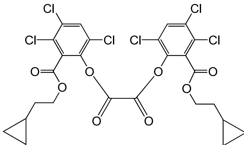
bis{3,4,6-trichloro-2-[(2-cyclopropylethoxy)carbonyl]phenyl} oxalate
