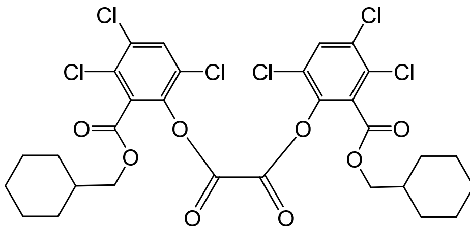
bis{3,4,6-trichloro-2-[(cyclohexylmethoxy)carbonyl]phenyl} oxalate
