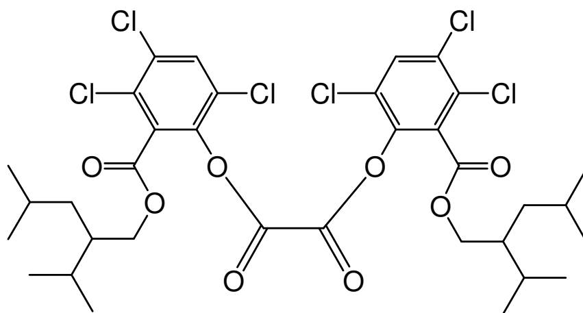
bis(3,4,6-trichloro-2-[[4-methyl-2-(1-methylethyl)pentyloxy]carbonyl]phenyl) oxalate
