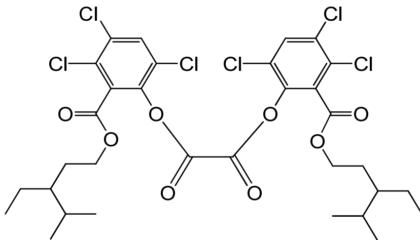
bis{3,4,6-trichloro-2-[(3-ethyl-4-methylpentyloxy)carbonyl]phenyl} oxalate
