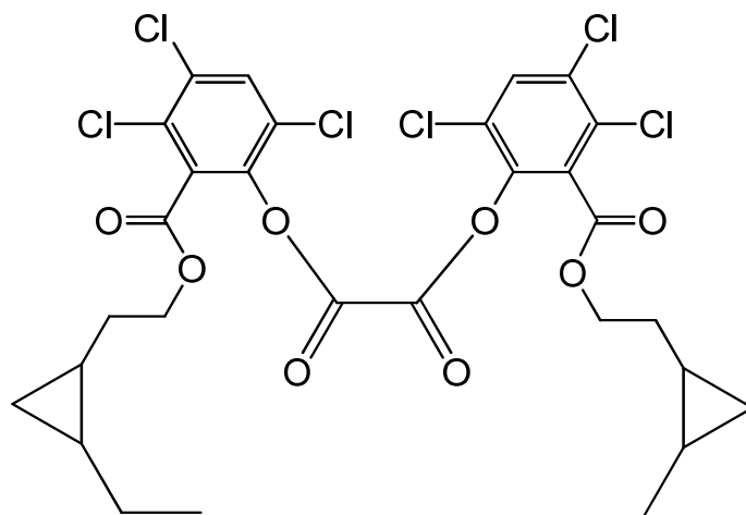
bis(3,4,6-trichloro-2-{[2-(2-ethylcyclopropyl)ethoxy]carbonyl}phenyl) oxalate
