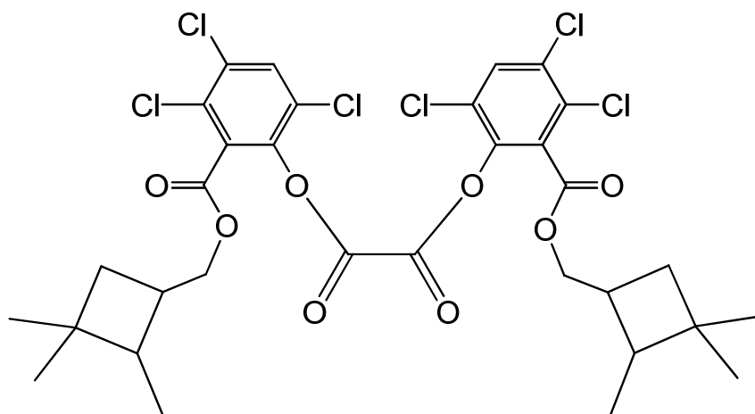
bis(3,4,6-trichloro-2-{[(2,3,3-trimethylcyclobutyl)methoxy]carbonyl}phenyl) oxalate
