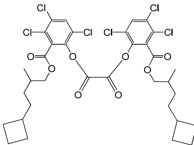
bis{3,4,6-trichloro-2-[(4-cyclobutyl-2-methylbutoxy)carbonyl]phenyl} oxalate
