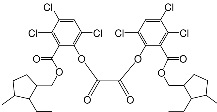
bis(3,4,6-trichloro-2-[(2-ethyl-3-methylcyclopentyl)methoxy]carbonyl)phenyl) oxalate
