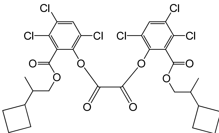
bis{3,4,6-trichloro-2-[(2-cyclobutylpropoxy)carbonyl]phenyl} oxalate
