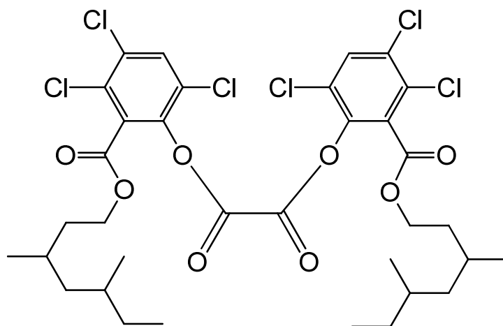
bis{3,4,6-trichloro-2-[(3,5-dimethylheptyloxy)carbonyl]phenyl} oxalate
