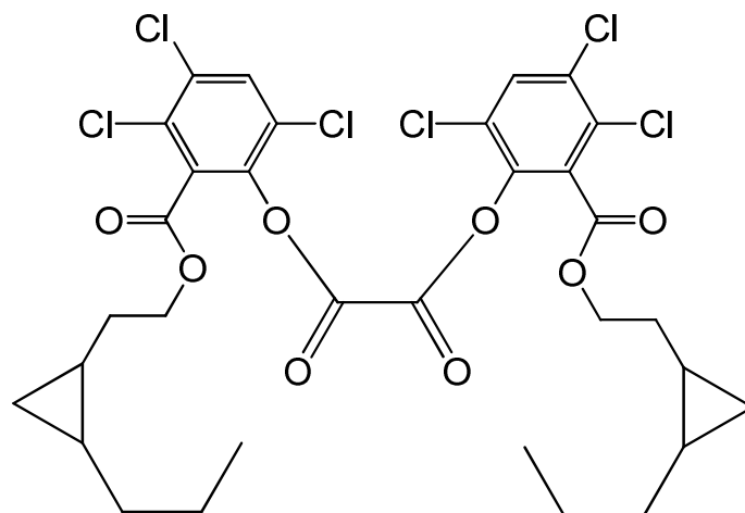
bis(3,4,6-trichloro-2-{[2-(2-propylcyclopropyl)ethoxy]carbonyl}phenyl) oxalate
