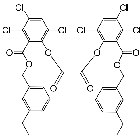
bis(3,4,6-trichloro-2-[[3-ethylphenyl)methoxy]carbonyl}phenyl) oxalate
