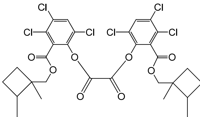
bis(3,4,6-trichloro-2-([(1,2-dimethylcyclobutyl)methoxy]carbonyl)phenyl) oxalate
