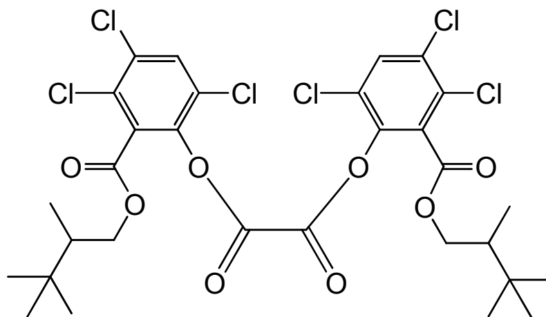
bis{3,4,6-trichloro-2-[(2,3,3-trimethylbutoxy)carbonyl]phenyl} oxalate
