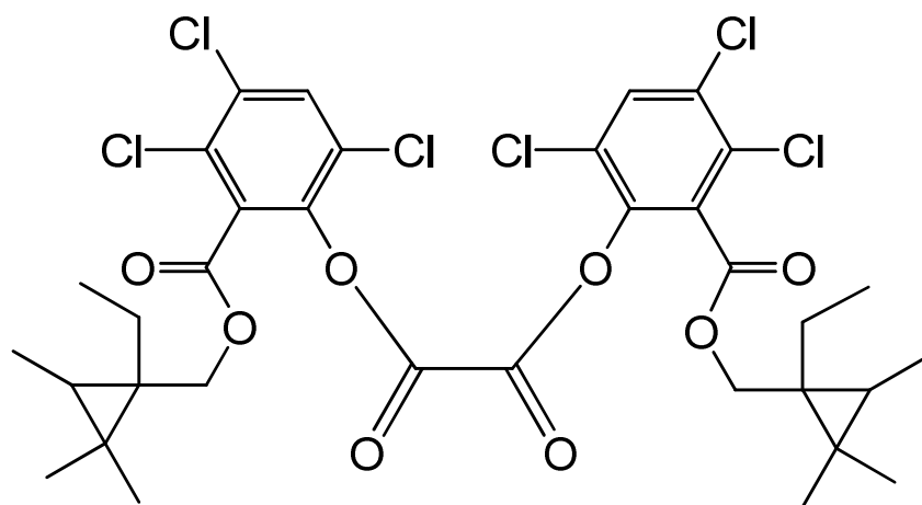
bis(3,4,6-trichloro-2-[[1-ethyl-2,2,3-trimethylcyclopropyl)methoxy]carbonyl}phenyl) oxalate
