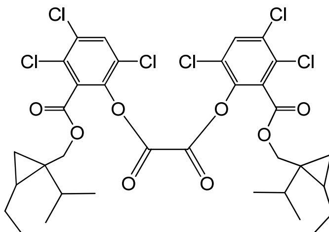
bis[3,4,6-trichloro-2-([2-ethyl-1-(1-methylethyl)-cyclopropyl]methoxy)carbonyl]phenyl oxalate
