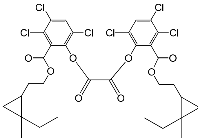
bis(3,4,6-trichloro-2-{{2-(2-ethyl-2-methylcyclopropyl)ethoxy}carbonyl}phenyl) oxalate
