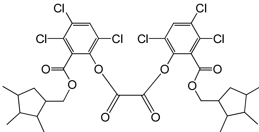
bis(3,4,6-trichloro-2-[(2,3,4-trimethylcyclopentyl)methoxy]carbonyl)phenyl oxalate
