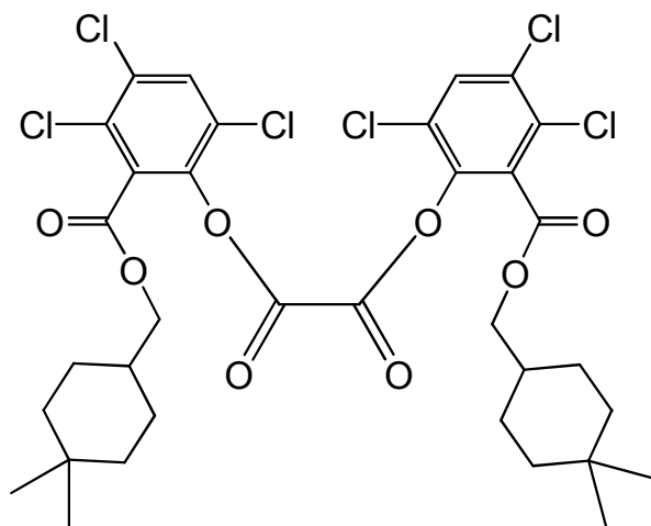
bis(3,4,6-trichloro-2-[[4,4-dimethylcyclohexyl)methoxy]carbonyl}phenyl) oxalate
