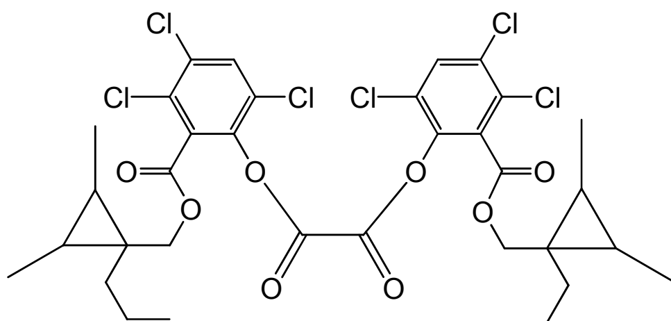
bis(3,4,6-trichloro-2-[(2,3-dimethyl-1-propylcyclopropyl)methoxy]carbonyl)phenyl oxalate
