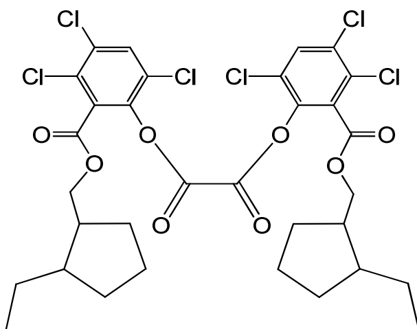
bis(3,4,6-trichloro-2-[(2-ethylcyclopentyl)methoxy]carbonyl)phenyl oxalate
