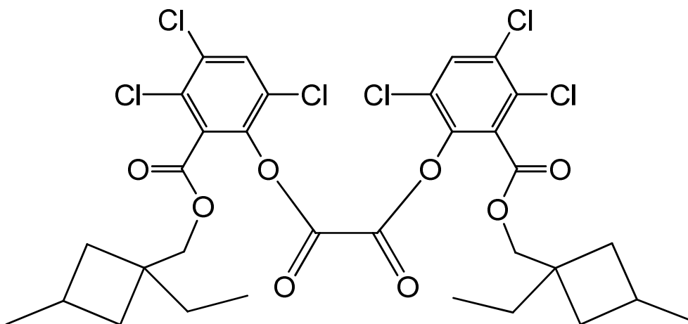
bis(3,4,6-trichloro-2-([(1-ethyl-3-methylcyclobutyl)methoxy]carbonyl)phenyl) oxalate
