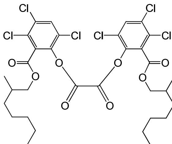
bis{3,4,6-trichloro-2-[(2-methylheptyloxy)carbonyl]phenyl} oxalate
