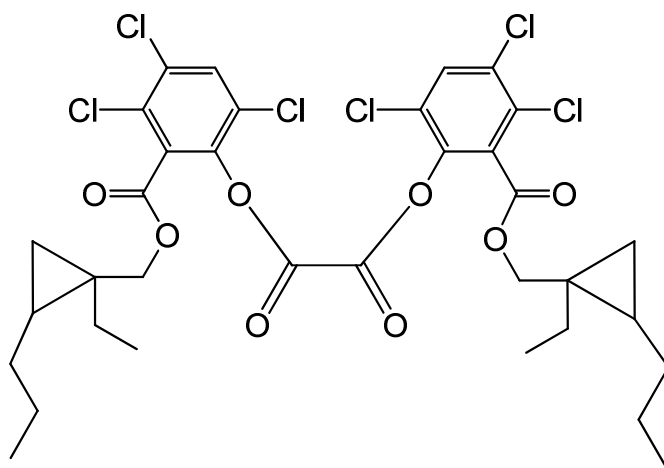
bis(3,4,6-trichloro-2-{{[(1-ethyl-2-propylcyclopropyl)methoxy]carbonyl}phenyl} oxalate
