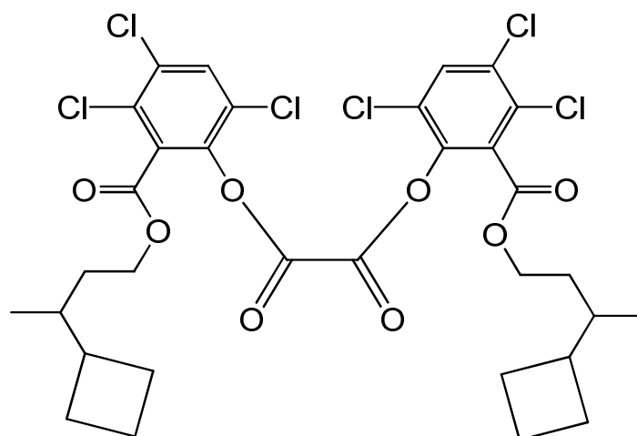
bis{3,4,6-trichloro-2-[(3-cyclobutylbutoxy)carbonyl]phenyl} oxalate
