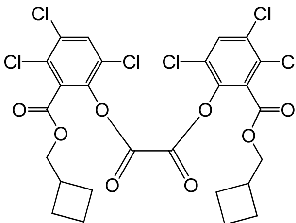
bis{3,4,6-trichloro-2-[(cyclobutylmethoxy)carbonyl]phenyl} oxalate
