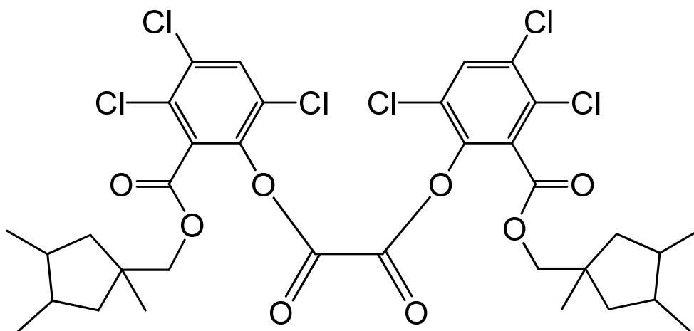
bis(3,4,6-trichloro-2-[(1,3,4-trimethylcyclopentyl)methoxy]carbonyl)phenyl oxalate
