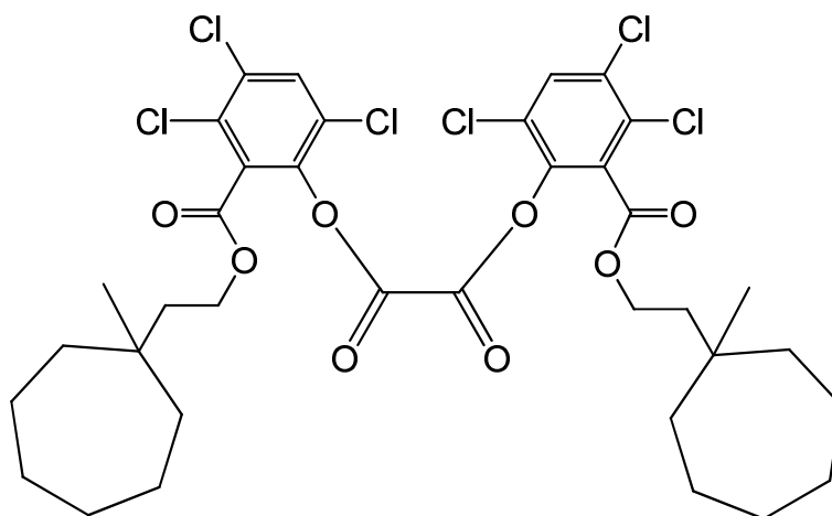
bis(3,4,6-trichloro-2-[[1-(1-methylcyclooctyl)methoxy]carbonyl]phenyl) oxalate
