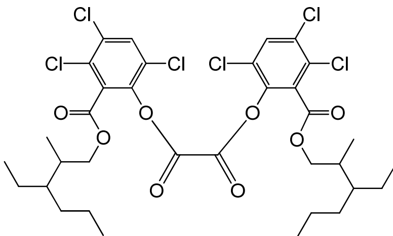
bis{3,4,6-trichloro-2-[(3-ethyl-2-methylhexyloxy)carbonyl]phenyl} oxalate
