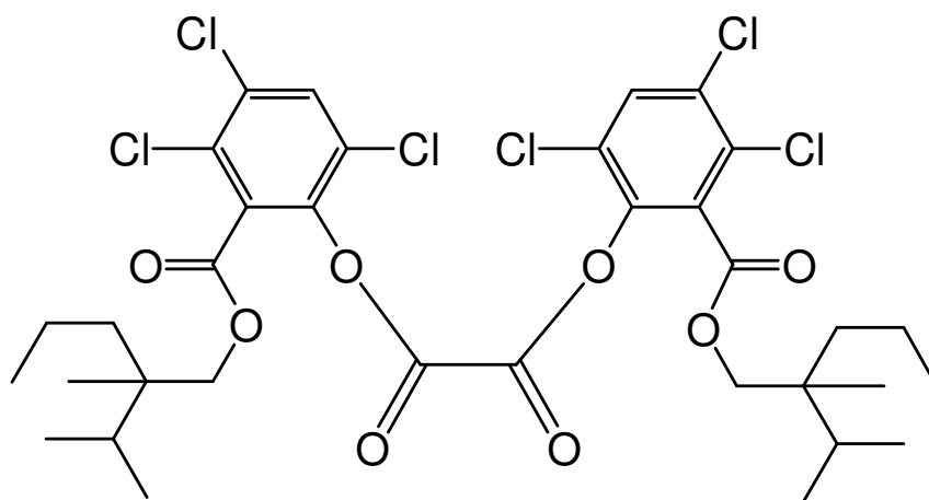
bis(3,4,6-trichloro-2-[[2-methyl-2-(1-methylethyl)pentyloxy]carbonyl]phenyl) oxalate
