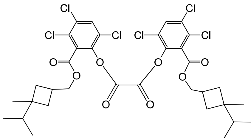
bis[3,4,6-trichloro-2-({[3-methyl-3-(1-methylethyl)cyclobutyl]methoxy}carbonyl)phenyl] oxalate
