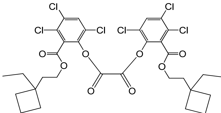
bis(3,4,6-trichloro-2-{[2-(1-ethylcyclobutyl)ethoxy]carbonyl}phenyl) oxalate
