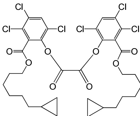
bis{3,4,6-trichloro-2-[(6-cyclopropylhexyloxy)carbonyl]phenyl} oxalate
