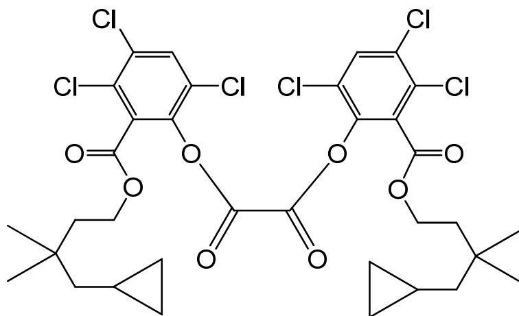
bis{3,4,6-trichloro-2-[(4-cyclopropyl-3,3-dimethylbutoxy)carbonyl]phenyl} oxalate
