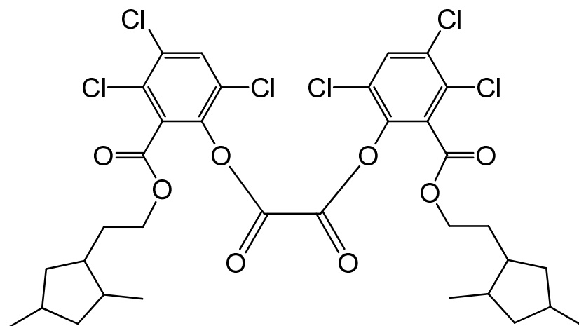
bis(3,4,6-trichloro-2-[[2-(2,4-dimethylcyclopentyl)ethoxy]carbonyl]phenyl) oxalate
