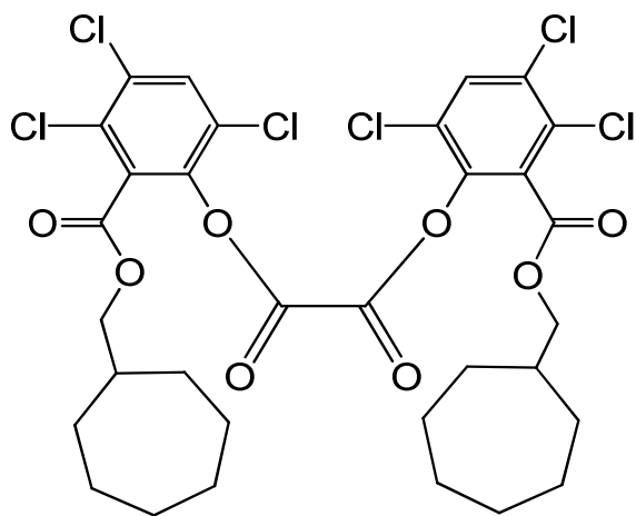
bis{3,4,6-trichloro-2-[(cycloheptylmethoxy)carbonyl]phenyl} oxalate
