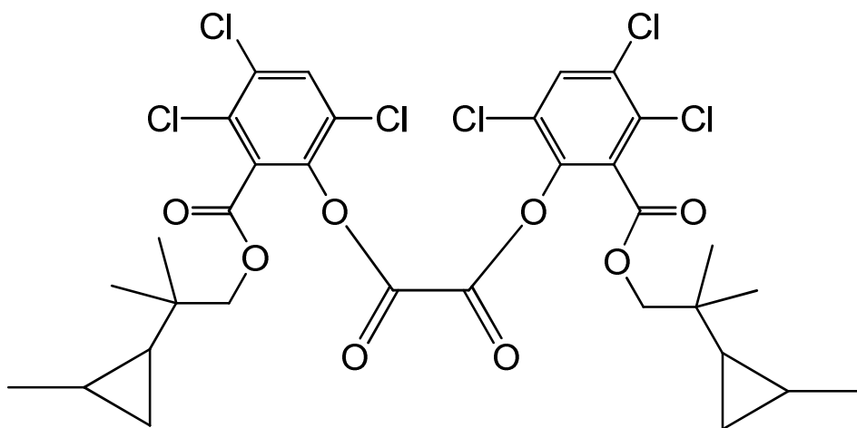
bis(3,4,6-trichloro-2-[[2-methyl-2-(2-methylcyclopropyl)propoxy]carbonyl]phenyl) oxalate
