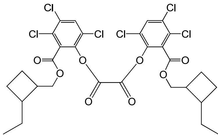
bis(3,4,6-trichloro-2-[(2-ethylcyclobutyl)methoxy]carbonyl)phenyl oxalate
