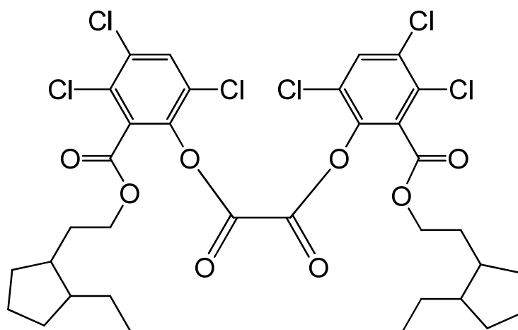
bis(3,4,6-trichloro-2-{[2-(2-ethylcyclopentyl)ethoxy]carbonyl}phenyl) oxalate
