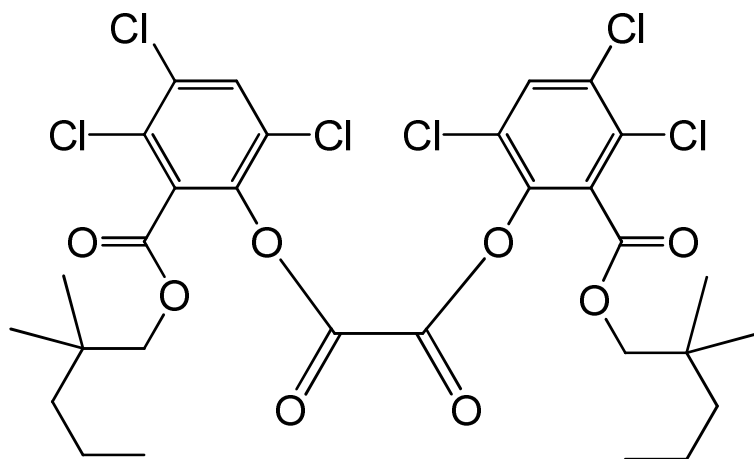
bis{3,4,6-trichloro-2-[(2,2-dimethylpentyloxy)carbonyl]phenyl} oxalate
