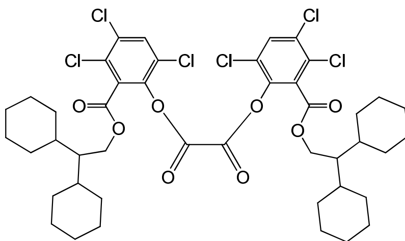
bis{3,4,6-trichloro-2-[(2,2-dicyclohexylethoxy)carbonyl]phenyl} oxalate
