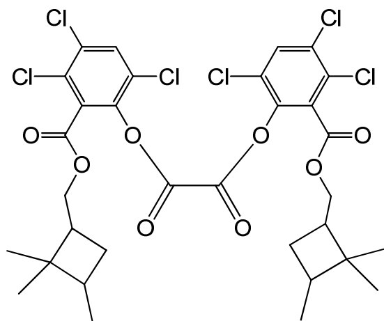
bis(3,4,6-trichloro-2-([(2,3-trimethylcyclobutyl)methoxy]carbonyl)phenyl) oxalate
