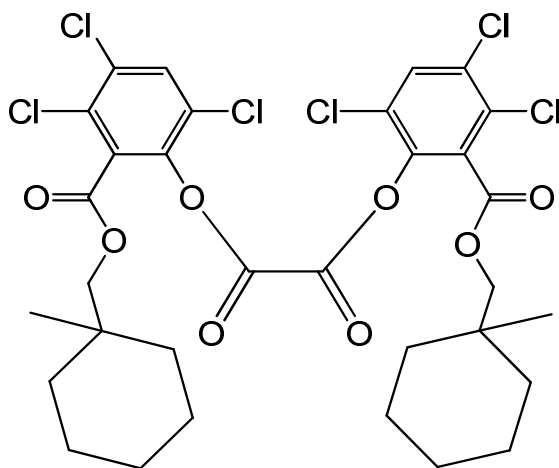
bis(3,4,6-trichloro-2-[(1-methylcyclohexyl)methoxy]carbonyl]phenyl) oxalate
