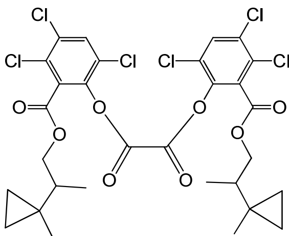
bis(3,4,6-trichloro-2-{[2-(1-methylcyclopropyl)propoxy]carbonyl}phenyl) oxalate
