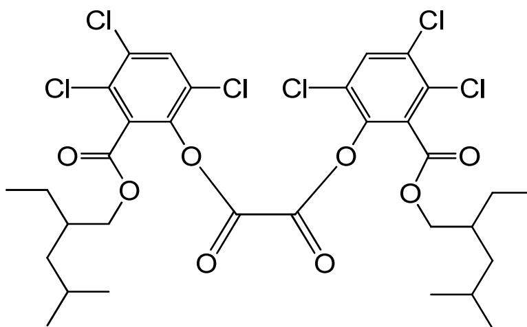
bis{3,4,6-trichloro-2-[(2-ethyl-4-methylpentyloxy)carbonyl]phenyl} oxalate
