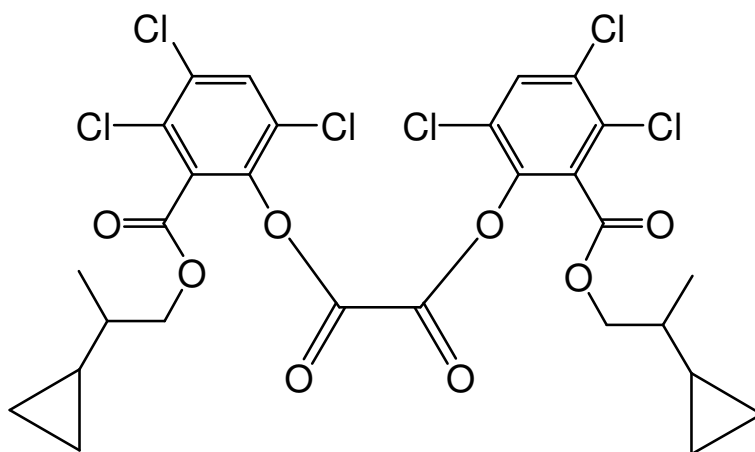
bis{3,4,6-trichloro-2-[(2-cyclopropylpropoxy)carbonyl]phenyl} oxalate
