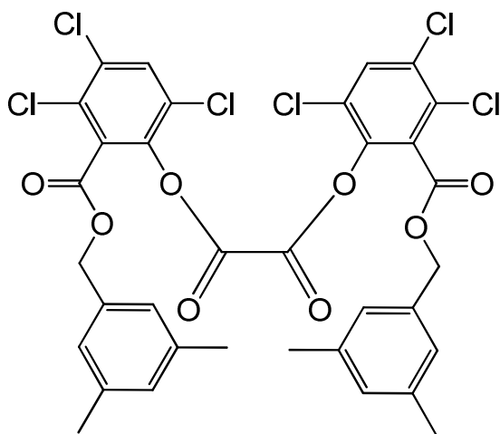
bis(3,4,6-trichloro-2-[[3,5-dimethylphenyl)methoxy]carbonyl}phenyl) oxalate
