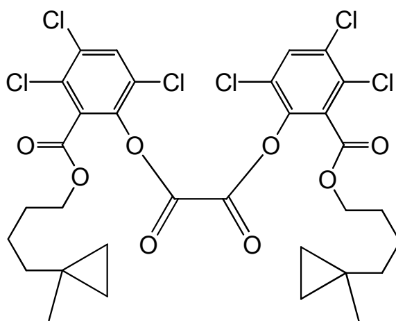
bis(3,4,6-trichloro-2-{[4-(1-methylcyclopropyl)butoxy]carbonyl}phenyl) oxalate
