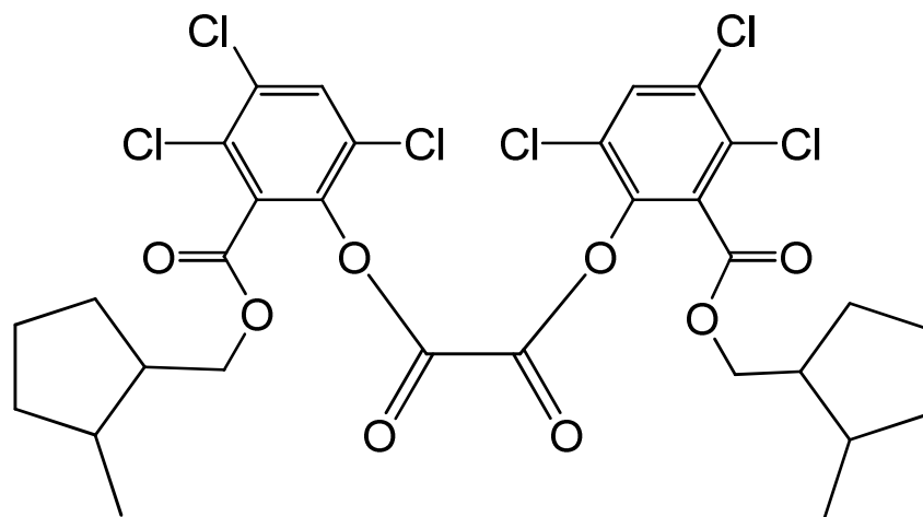
bis(3,4,6-trichloro-2-{[(2-methylcyclopentyl)methoxy]carbonyl}phenyl) oxalate
