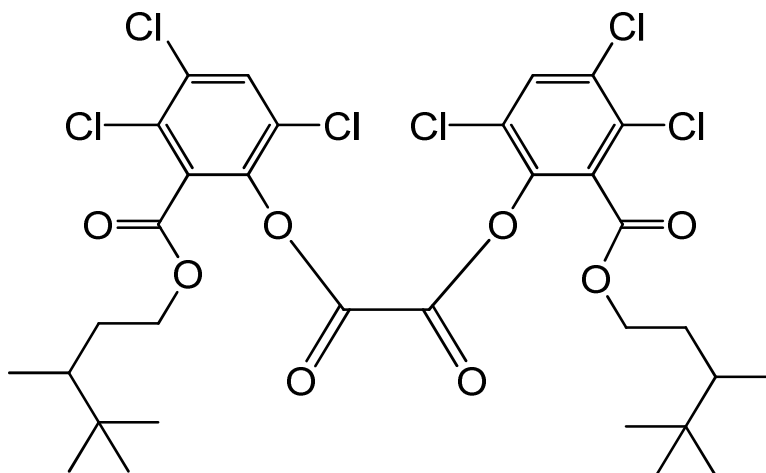
bis{3,4,6-trichloro-2-[(3,4,4-trimethylpentyloxy)carbonyl]phenyl} oxalate
