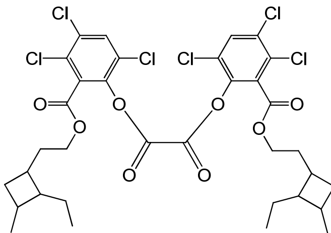
bis(3,4,6-trichloro-2-[[2-(2-ethyl-3-methylcyclobutyl)ethoxy]carbonyl]phenyl) oxalate
