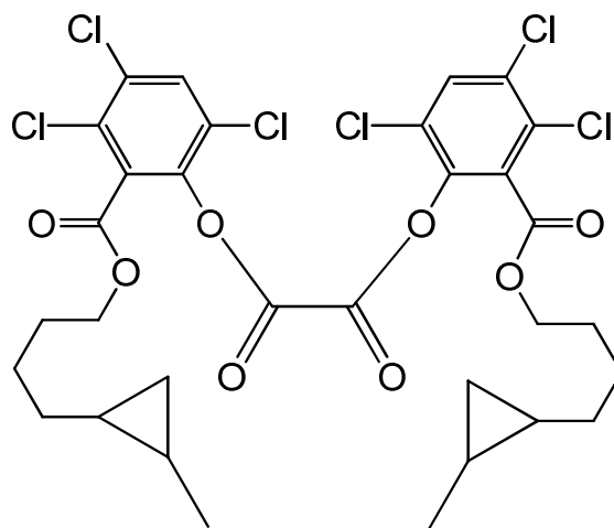
bis(3,4,6-trichloro-2-{[4-(2-methylcyclopropyl)butoxy]carbonyl}phenyl) oxalate
