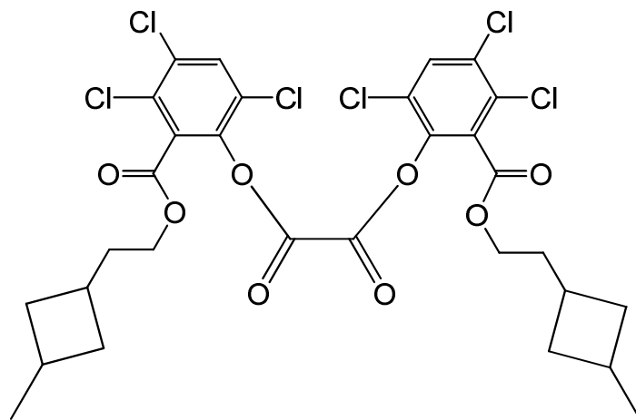
bis(3,4,6-trichloro-2-[[2-(3-methylcyclobutyl)ethoxy]carbonyl]phenyl) oxalate
