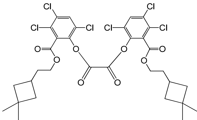
bis(3,4,6-trichloro-2-{[2-(3,3-dimethylcyclobutyl)ethoxy]carbonyl}phenyl) oxalate
