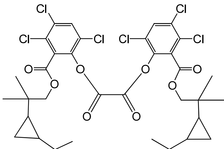
bis(3,4,6-trichloro-2-{-2-(2-ethylcyclopropyl)-2-methylpropoxy}carbonyl}phenyl) oxalate
