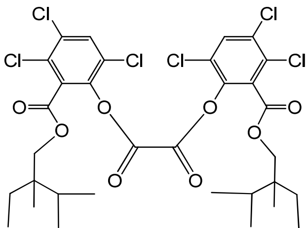
bis{3,4,6-trichloro-2-[(2-ethyl-2,3-dimethylbutoxy)carbonyl]phenyl} oxalate
