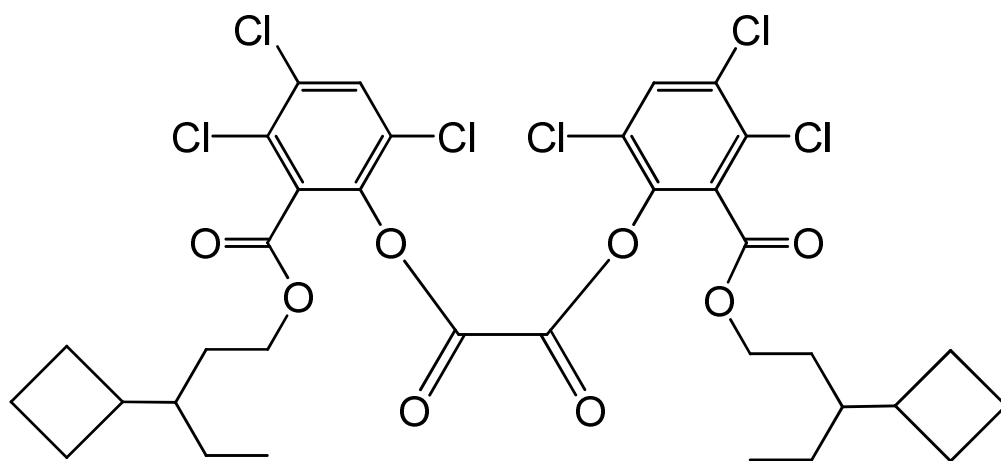
bis{3,4,6-trichloro-2-[(3-cyclobutylpentyl)oxy]carbonyl}phenyl} oxalate
