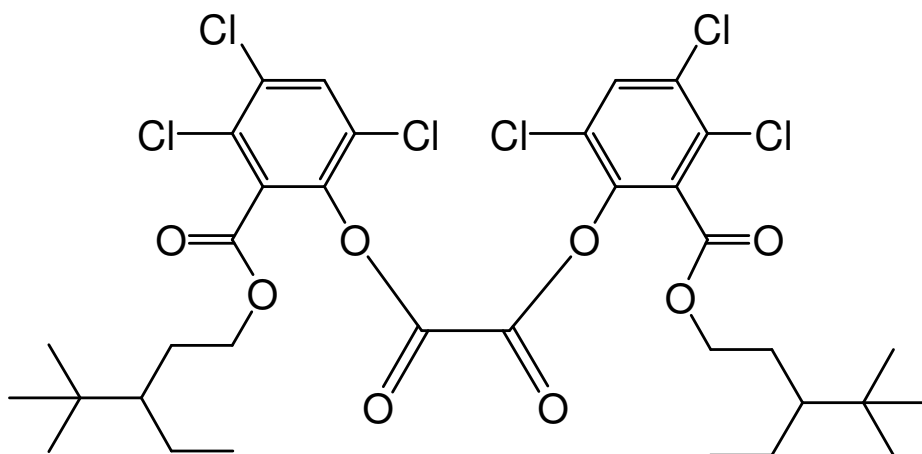
bis(3,4,6-trichloro-2-{[2-(1,1-dimethylethyl)pentyloxy]carbonyl}phenyl) oxalate
