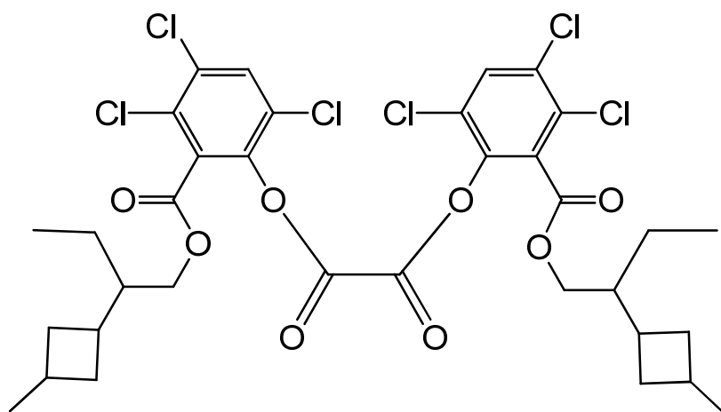
bis(3,4,6-trichloro-2-[[2-(3-methylcyclobutyl)butoxy]carbonyl]phenyl) oxalate
