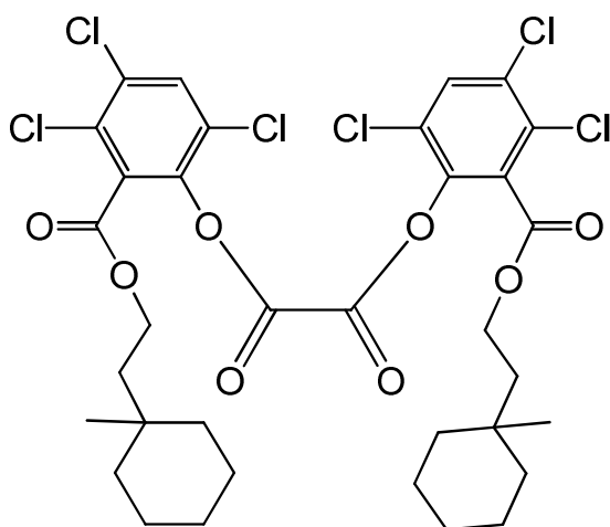
bis(3,4,6-trichloro-2-[[2-(1-methylcyclohexyl)ethoxy]carbonyl]phenyl) oxalate
