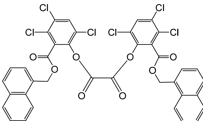
bis{3,4,6-trichloro-2-[1-naphthalenylmethoxy]carbonyl}phenyl} oxalate
