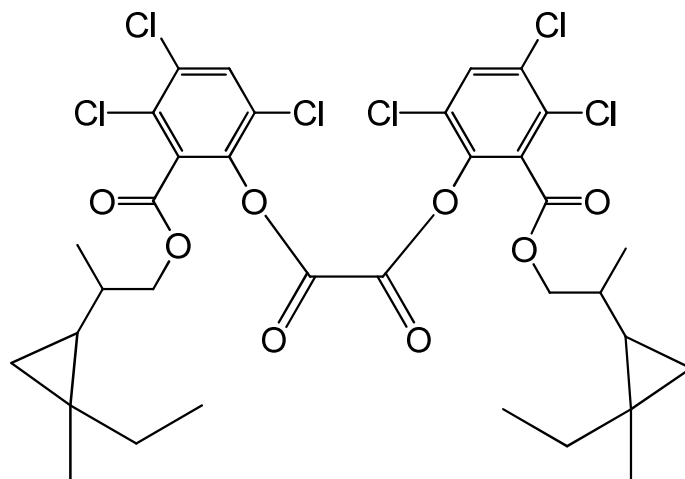
bis(3,4,6-trichloro-2-{[2-(2-ethyl-2-methylcyclopropyl)propoxy]carbonyl}phenyl) oxalate
