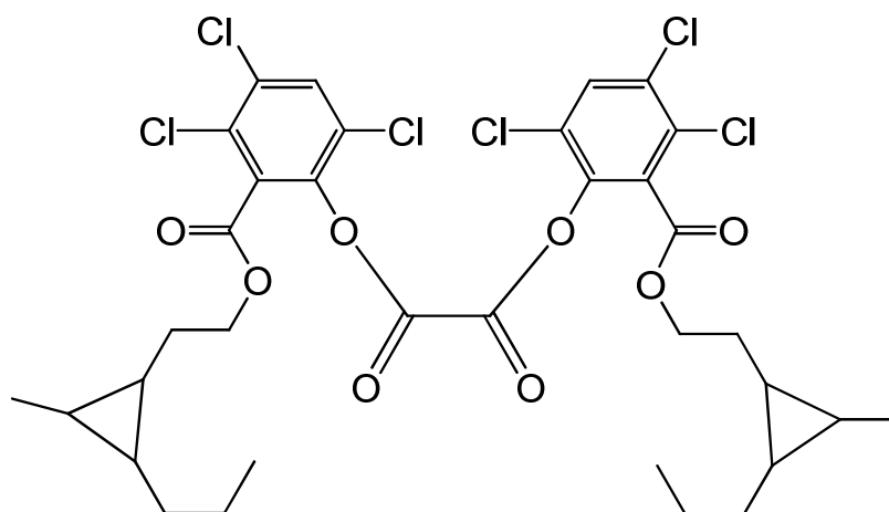
bis(3,4,6-trichloro-2-{[2-(2-methyl-3-propylcyclopropyl)ethoxy]carbonyl}phenyl) oxalate
