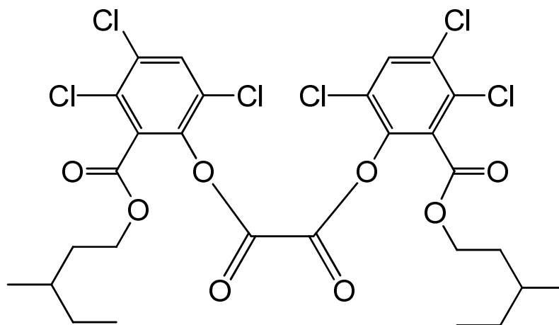
bis{3,4,6-trichloro-2-[(3-methylpentyl)oxy]carbonyl}phenyl oxalate
