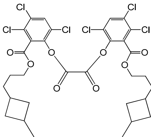
bis(3,4,6-trichloro-2-[[3-(3-methylcyclobutyl)propoxy]carbonyl]phenyl) oxalate
