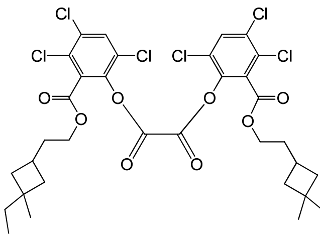
bis(3,4,6-trichloro-2-{[2-(3-ethyl-3-methylcyclobutyl)ethoxy]carbonyl}phenyl) oxalate
