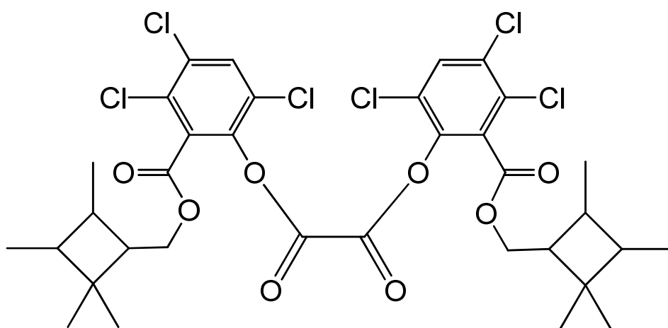
bis(3,4,6-trichloro-2-[(2,2,3,4-tetramethylcyclobutyl)methoxy]carbonyl}phenyl) oxalate
