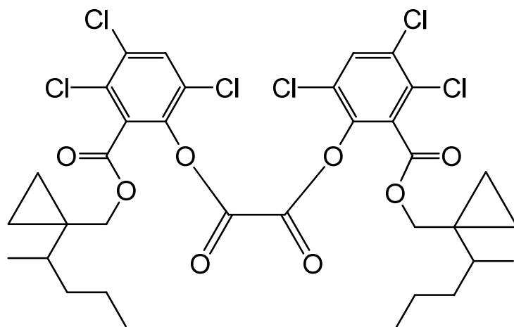
bis[3,4,6-trichloro-2-([1-(1-methylbutyl)cyclopropyl]methoxy)carbonyl]phenyl] oxalate
