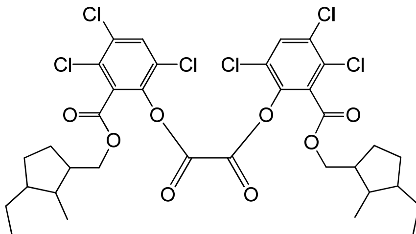
bis(3,4,6-trichloro-2-[(3-ethyl-2-methylcyclopentyl)methoxy]carbonyl)phenyl oxalate
