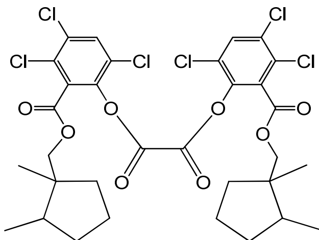
bis(3,4,6-trichloro-2-[[1,2-dimethylcyclopentyl)methoxy]carbonyl}phenyl) oxalate
