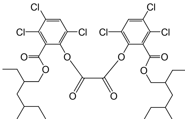
bis{3,4,6-trichloro-2-[(2-ethyl-4-methylhexyloxy)carbonyl]phenyl} oxalate
