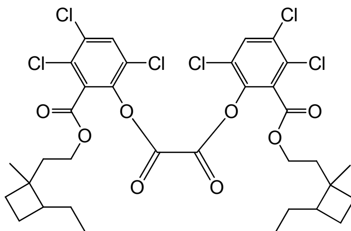
bis(3,4,6-trichloro-2-{[2-(2-ethyl-1-methylcyclobutyl)ethoxy]carbonyl}phenyl) oxalate
