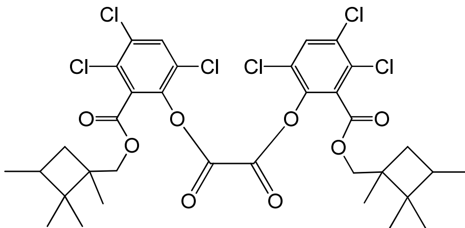
bis(3,4,6-trichloro-2-[(1,2,2,3-tetramethylcyclobutyl)methoxy]carbonyl}phenyl) oxalate
