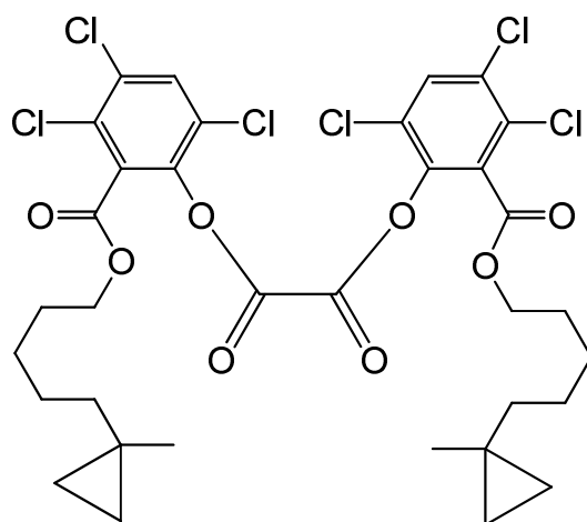
bis(3,4,6-trichloro-2-{[5-(1-methylcyclopropyl)pentyloxy]carbonyl}phenyl) oxalate
