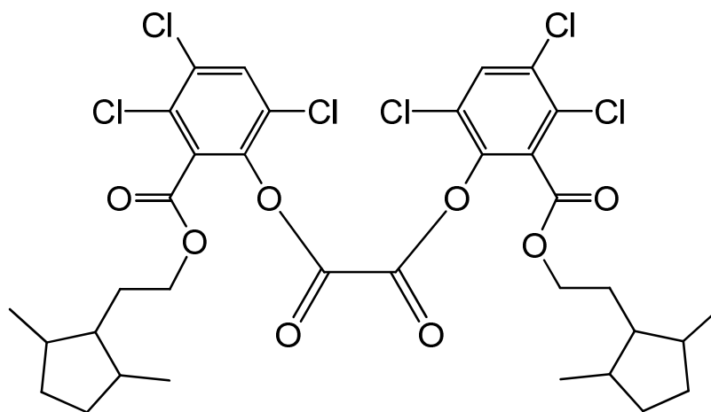
bis(3,4,6-trichloro-2-[[2-(2,5-dimethylcyclopentyl)ethoxy]carbonyl]phenyl) oxalate
