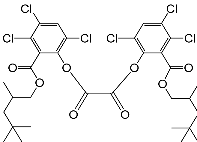
bis{3,4,6-trichloro-2-[(2,4,4-trimethylpentyloxy)carbonyl]phenyl} oxalate
