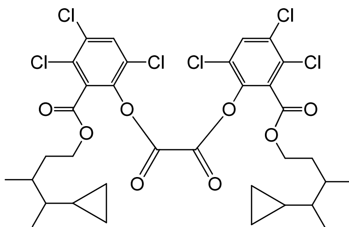
bis{3,4,6-trichloro-2-[(4-cyclopropyl-3-methylpentyloxy)carbonyl]phenyl} oxalate
