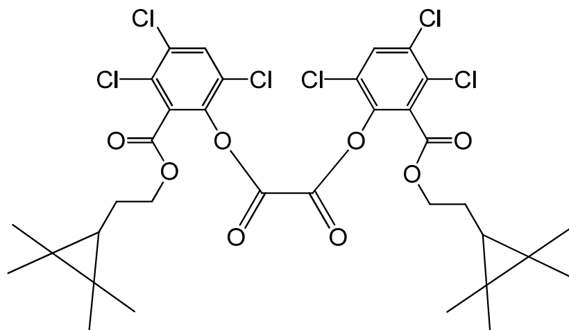
bis(3,4,6-trichloro-2-{[2-(2,2,3,3-tetramethylcyclopropyl)ethoxy]carbonyl}phenyl) oxalate
