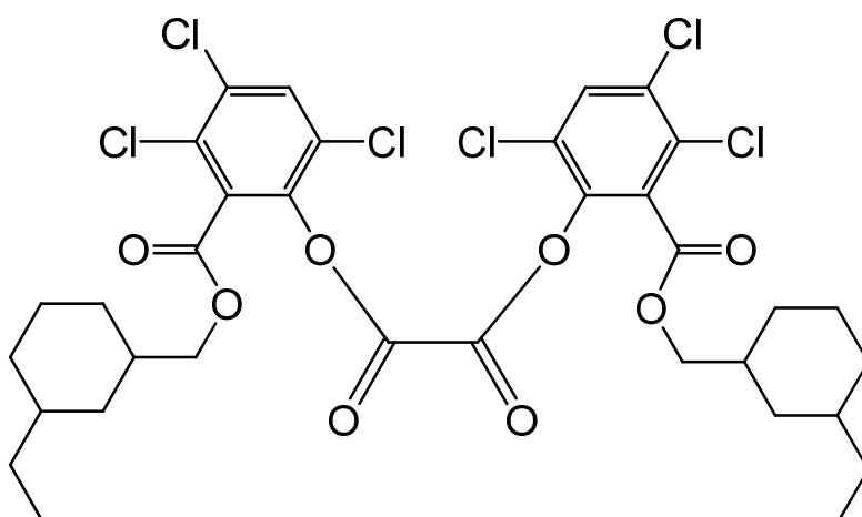
bis(3,4,6-trichloro-2-{[3-ethylcyclohexyl)methoxy]carbonyl}phenyl) oxalate
