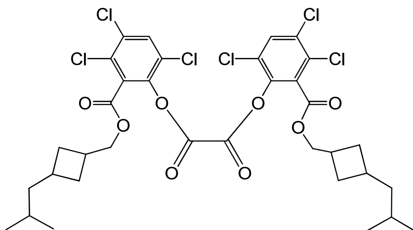
bis[3,4,6-trichloro-2-({[3-(2-methylpropyl)cyclobutyl]methoxy}carbonyl)phenyl] oxalate
