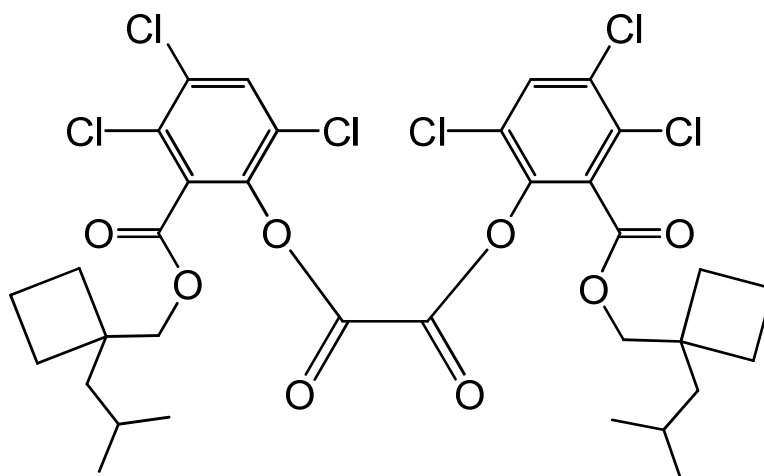
bis[3,4,6-trichloro-2-([1-(2-methylpropyl)cyclobutyl]methoxy)carbonyl]phenyl oxalate
