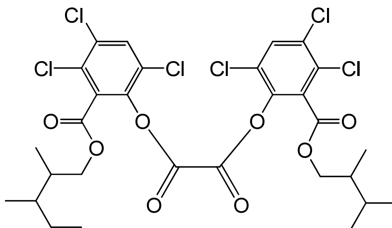
bis{3,4,6-trichloro-2-[(2,3-dimethylpentyloxy)carbonyl]phenyl} oxalate
