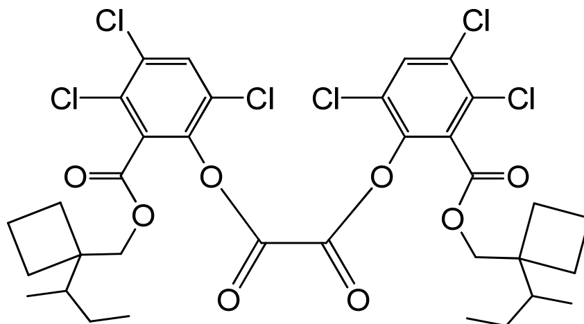
bis[3,4,6-trichloro-2-([1-(1-methylpropyl)cyclobutyl]methoxy)carbonyl]phenyl oxalate
