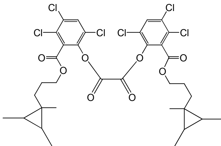
bis(3,4,6-trichloro-2-[[3-(1,2,3-trimethylcyclopropyl)propoxy]carbonyl]phenyl) oxalate
