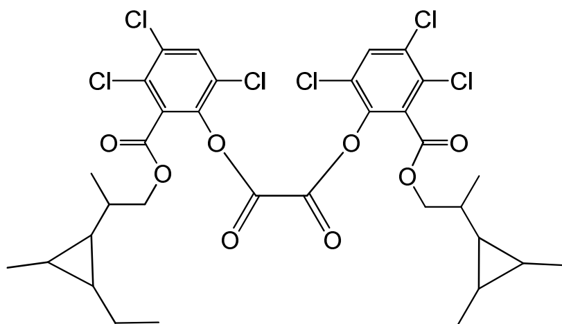
bis(3,4,6-trichloro-2-[[2-(2-ethyl-3-methylcyclopropyl)propoxy]carbonyl]phenyl) oxalate
