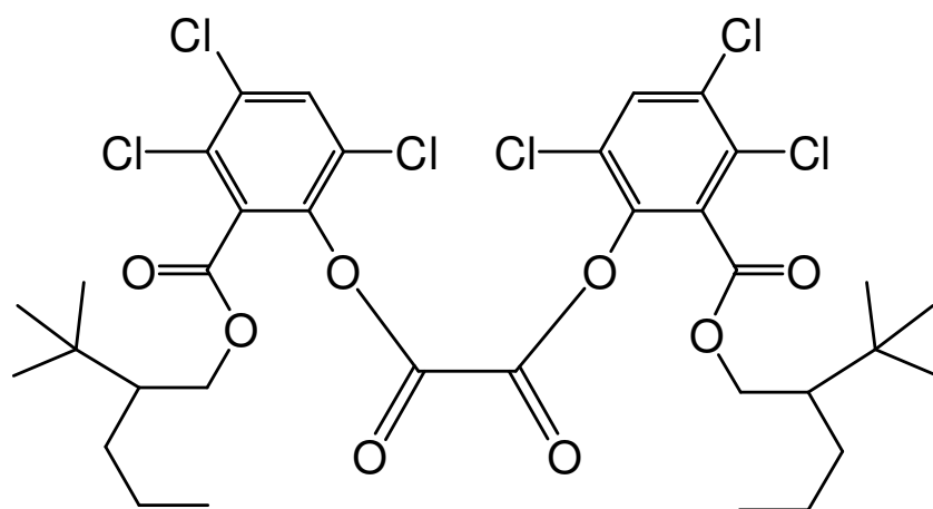
bis(3,4,6-trichloro-2-{[2-(1,1-dimethylethyl)pentyloxy]carbonyl}phenyl) oxalate
