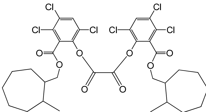
bis(3,4,6-trichloro-2-[[2-(2-methylcyclooctyl)methoxy]carbonyl]phenyl) oxalate
