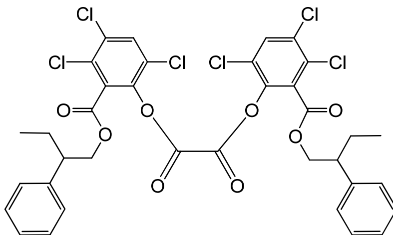
bis{3,4,6-trichloro-2-[(2-phenylbutoxy)carbonyl]phenyl} oxalate
