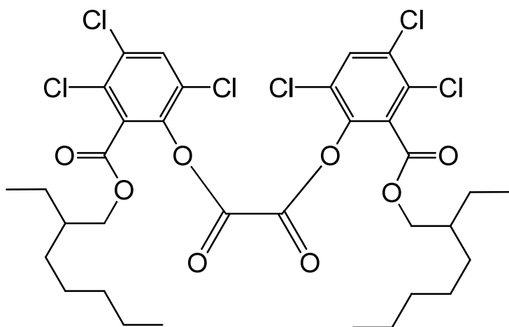
bis{3,4,6-trichloro-2-[(2-ethylheptyloxy)carbonyl]phenyl} oxalate
