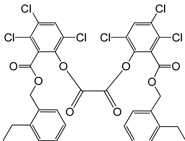
bis(3,4,6-trichloro-2-[[2-ethylphenyl)methoxy]carbonyl}phenyl) oxalate
