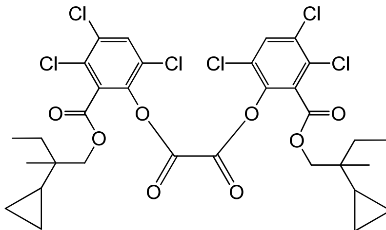
bis{3,4,6-trichloro-2-[(2-cyclopropyl-2-methylbutoxy)carbonyl]phenyl} oxalate
