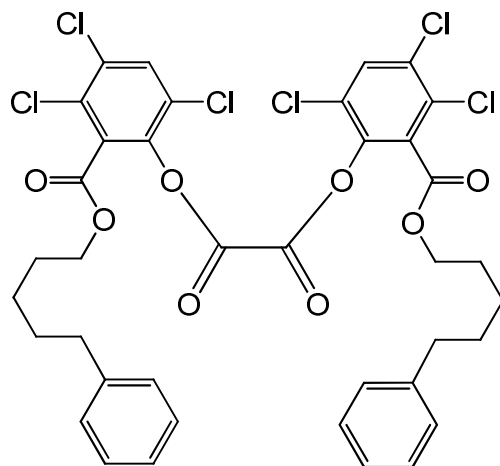
bis{3,4,6-trichloro-2-[(5-phenylpentyl)oxy]carbonyl}phenyl} oxalate
