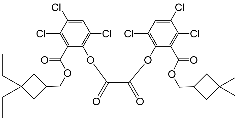
bis(3,4,6-trichloro-2-[[3,3-diethylcyclobutyl)methoxy]carbonyl}phenyl) oxalate
