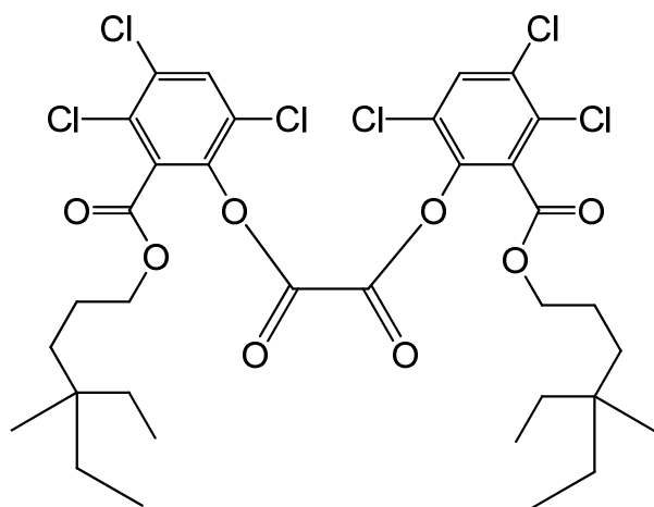
bis{3,4,6-trichloro-2-[(4-ethyl-4-methylhexyloxy)carbonyl]phenyl} oxalate
