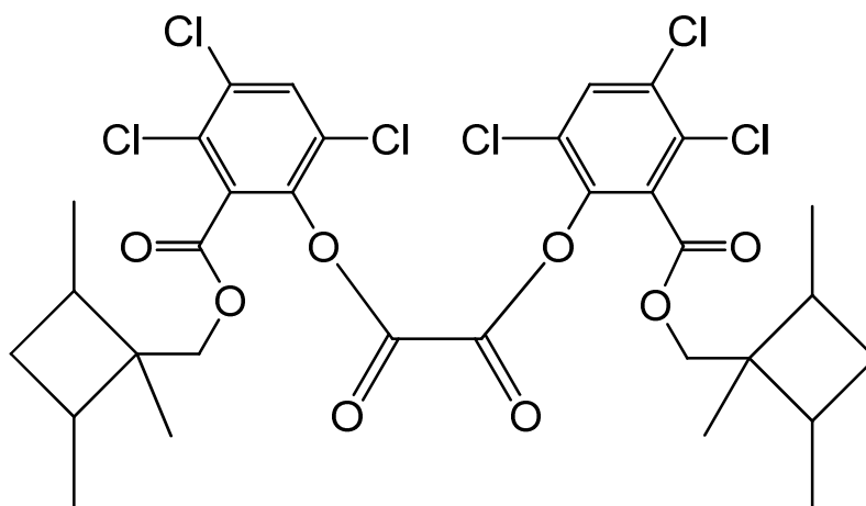
bis(3,4,6-trichloro-2-([(1,2,4-trimethylcyclobutyl)methoxy]carbonyl)phenyl) oxalate
