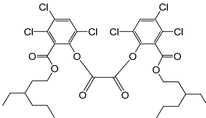
bis{3,4,6-trichloro-2-[(3-ethylhexyloxy)carbonyl]phenyl} oxalate
