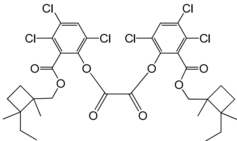
bis(3,4,6-trichloro-2-[[2-ethyl-1,2-dimethylcyclobutyl)methoxy]carbonyl]phenyl) oxalate
