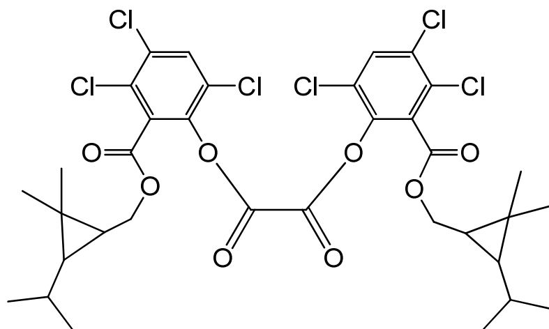
bis[3,4,6-trichloro-2-([2,2-dimethyl-3-(1-methylethyl)-cyclopropyl]methoxy)carbonyl]phenyl] oxalate
