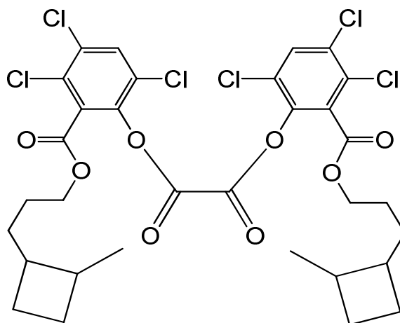
bis(3,4,6-trichloro-2-[[3-(2-methylcyclobutyl)propoxy]carbonyl]phenyl) oxalate
