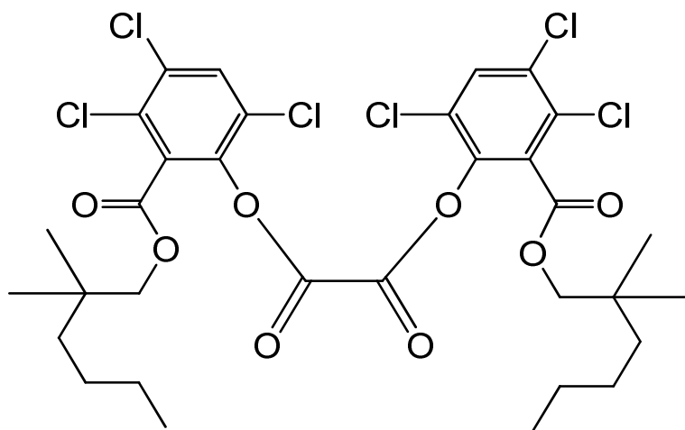
bis{3,4,6-trichloro-2-[(2,2-dimethylhexyloxy)carbonyl]phenyl} oxalate
