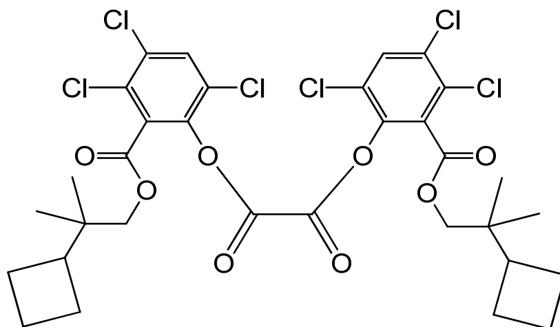
bis{3,4,6-trichloro-2-[(2-cyclobutyl-2-methylpropoxy)carbonyl]phenyl} oxalate
