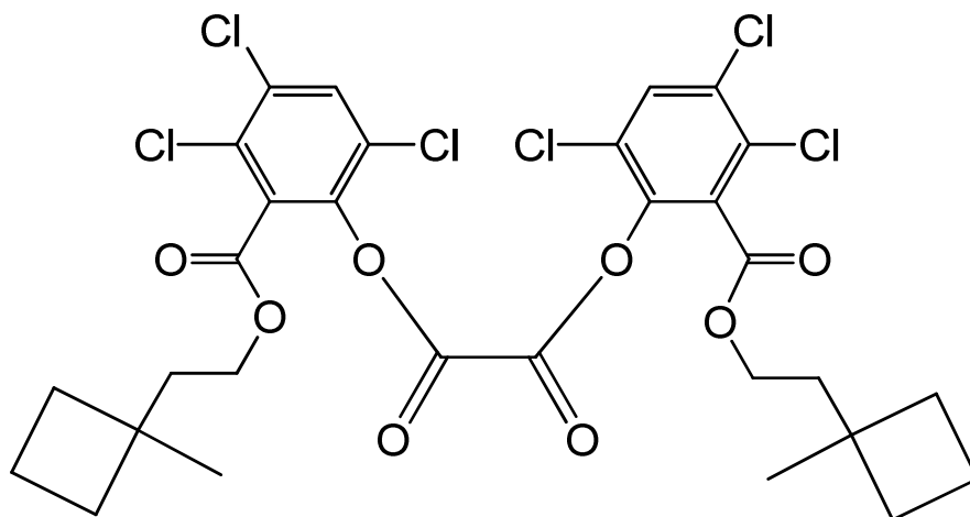
bis(3,4,6-trichloro-2-[2-(1-methylcyclobutyl)ethoxy]carbonyl)phenyl oxalate
