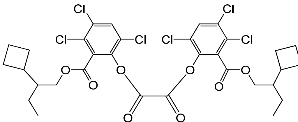
bis{3,4,6-trichloro-2-[(2-cyclobutylbutoxy)carbonyl]phenyl} oxalate
