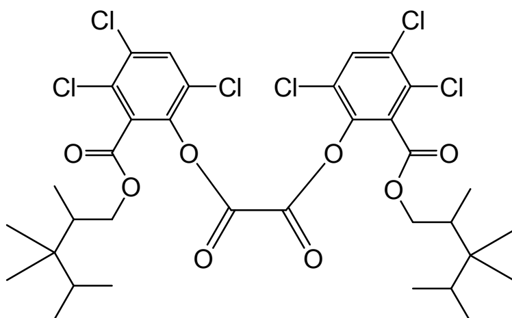
bis{3,4,6-trichloro-2-[(2,3,3,4-tetramethylpentyloxy)carbonyl]phenyl} oxalate
