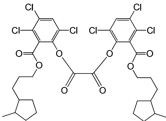
bis(3,4,6-trichloro-2-[[3-(2-methylcyclopentyl)propoxy]carbonyl]phenyl) oxalate
