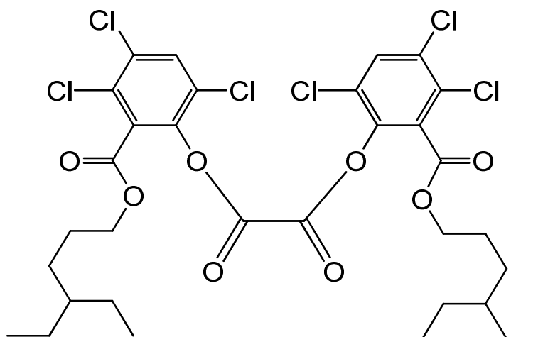
bis{3,4,6-trichloro-2-[(4-ethylhexyloxy)carbonyl]phenyl} oxalate
