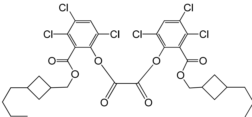
bis(3,4,6-trichloro-2-[(3-butylcyclobutyl)methoxy]carbonyl)phenyl oxalate
