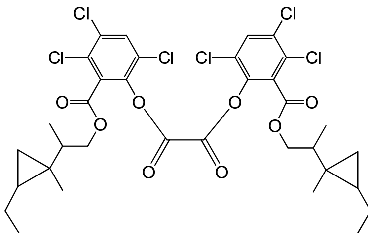
bis(3,4,6-trichloro-2-[[2-(2-ethyl-1-methylcyclopropyl)propoxy]carbonyl]phenyl) oxalate
