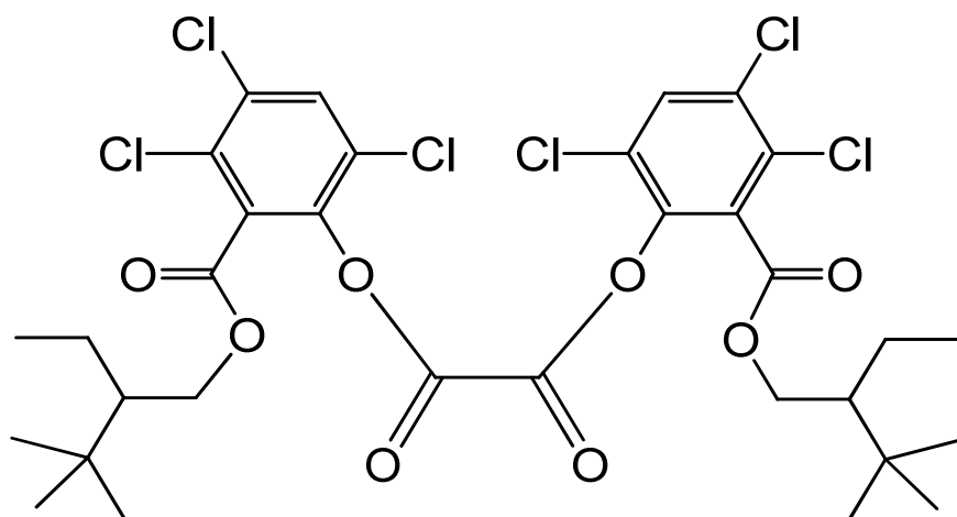
bis{3,4,6-trichloro-2-[(2-ethyl-3,3-dimethylbutoxy)carbonyl]phenyl} oxalate
