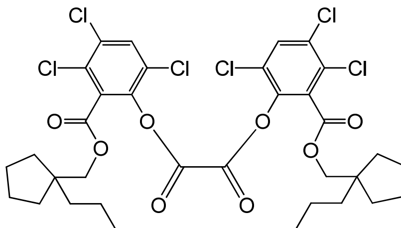
bis(3,4,6-trichloro-2-[[1-propylcyclopentyl)methoxy]carbonyl}phenyl) oxalate
