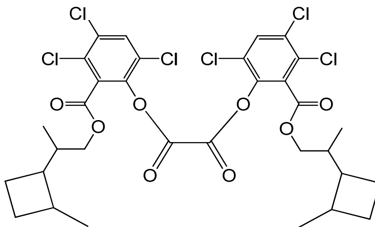
bis(3,4,6-trichloro-2-([2-(2-methylcyclobutyl)propoxy]carbonyl)phenyl) oxalate
