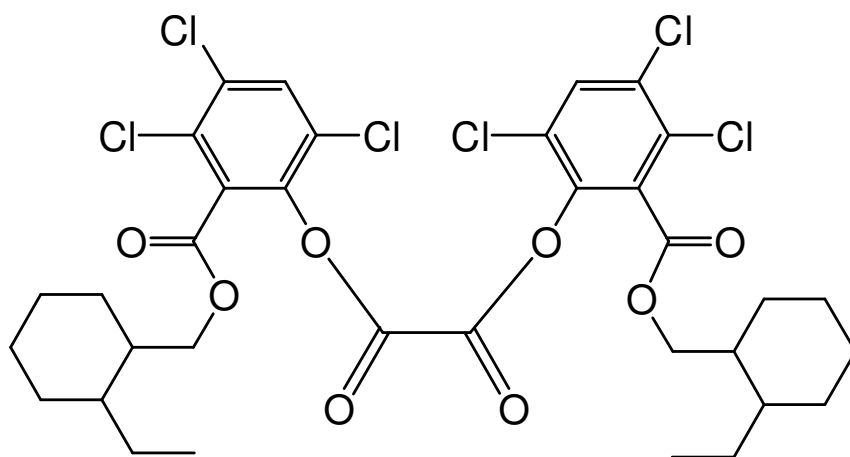
bis(3,4,6-trichloro-2-{[2-ethylcyclohexyl)methoxy]carbonyl}phenyl) oxalate
