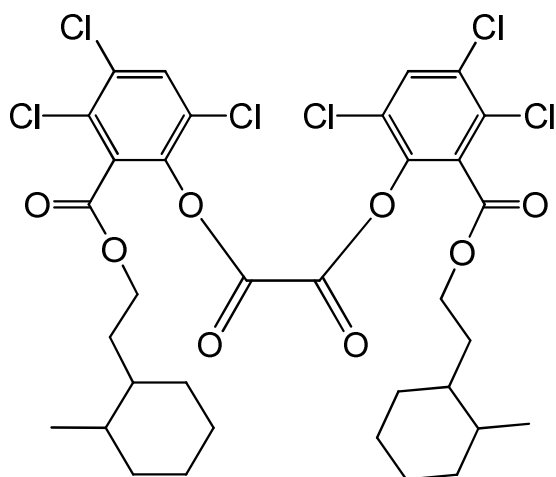
bis(3,4,6-trichloro-2-{[2-(2-methylcyclohexyl)ethoxy]carbonyl}phenyl) oxalate
