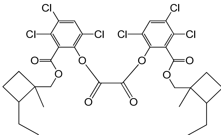
bis(3,4,6-trichloro-2-[(2-ethyl-1-methylcyclobutyl)methoxy]carbonyl)phenyl oxalate
