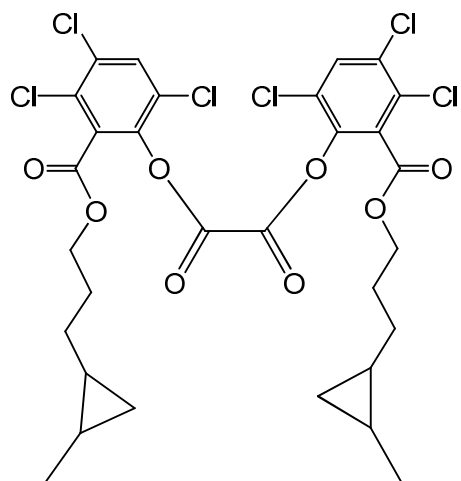
bis(3,4,6-trichloro-2-[[3-(2-methylcyclopropyl)propoxy]carbonyl]phenyl) oxalate
