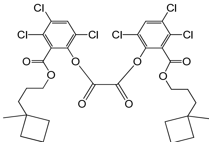
bis(3,4,6-trichloro-2-[[3-(1-methylcyclobutyl)propoxy]carbonyl]phenyl) oxalate
