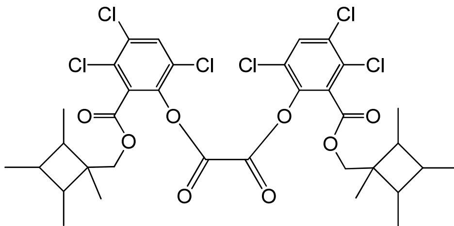
bis(3,4,6-trichloro-2-[(1,2,3,4-tetramethylcyclobutyl)methoxy]carbonyl}phenyl) oxalate
