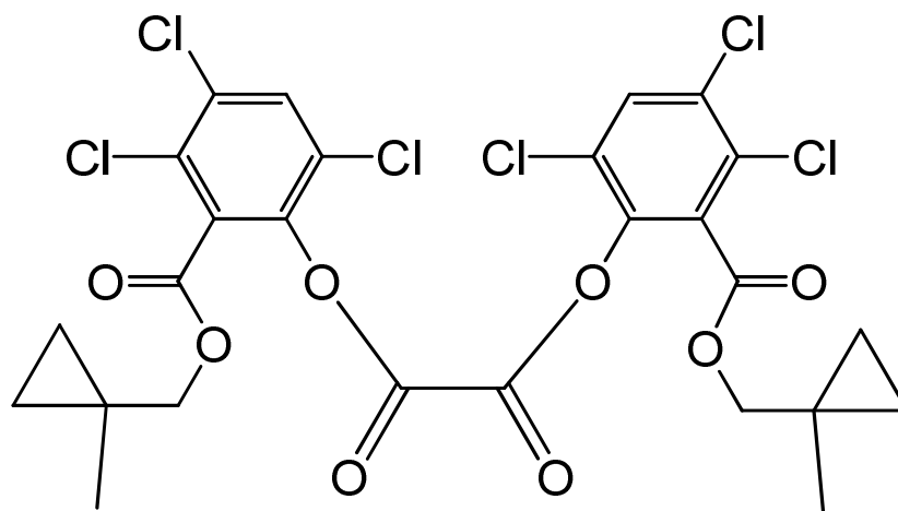
bis(3,4,6-trichloro-2-[[1-methylcyclopropyl)methoxy]carbonyl)phenyl) oxalate
