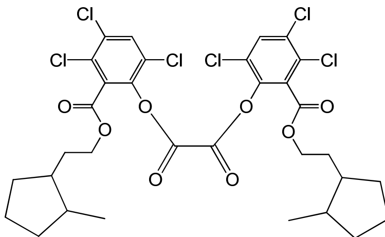
bis(3,4,6-trichloro-2-{[2-(2-methylcyclopentyl)ethoxy]carbonyl}phenyl) oxalate
