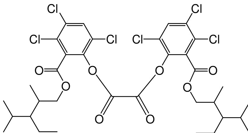
bis{3,4,6-trichloro-2-[(3-ethyl-2,4-dimethylpentyloxy)carbonyl]phenyl} oxalate
