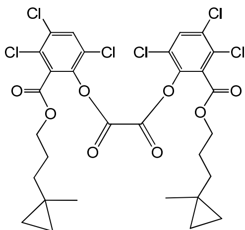
bis(3,4,6-trichloro-2-[[3-(1-methylcyclopropyl)propoxy]carbonyl]phenyl) oxalate
