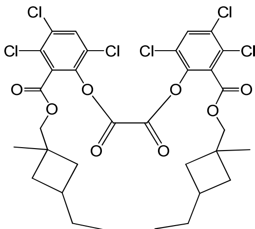
bis(3,4,6-trichloro-2-[(3-ethyl-1-methylcyclobutyl)methoxy]carbonyl)phenyl oxalate
