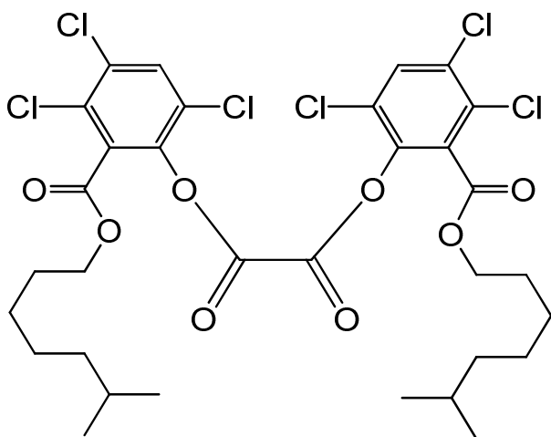
bis{3,4,6-trichloro-2-[(6-methylheptyloxy)carbonyl]phenyl} oxalate
