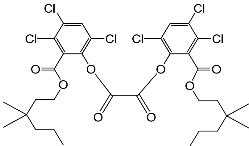
bis{3,4,6-trichloro-2-[(3,3-dimethylhexyloxy)carbonyl]phenyl} oxalate
