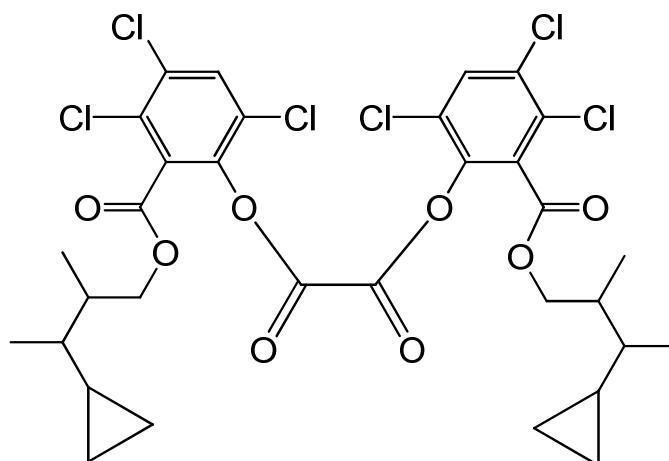
bis{3,4,6-trichloro-2-[(3-cyclopropyl-2-methylbutoxy)carbonyl]phenyl} oxalate
