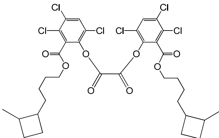
bis(3,4,6-trichloro-2-{[4-(2-methylcyclobutyl)butoxy]carbonyl}phenyl) oxalate
