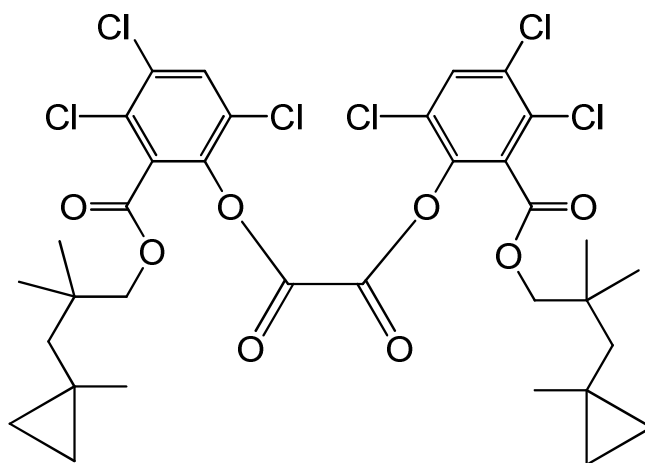
bis(3,4,6-trichloro-2-{[2,2-dimethyl-3-(1-methylcyclopropyl)propoxy]carbonyl}phenyl) oxalate
