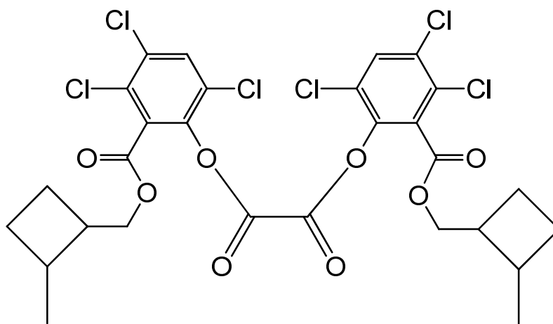
bis(3,4,6-trichloro-2-[[2-methylcyclobutyl)methoxy]carbonyl}phenyl) oxalate
