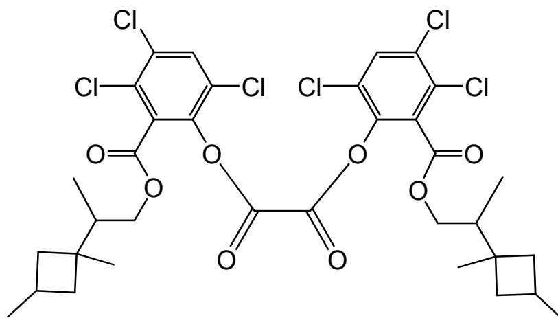
bis(3,4,6-trichloro-2-{[2-(1,3-dimethylcyclobutyl)propoxy]carbonyl}phenyl) oxalate
