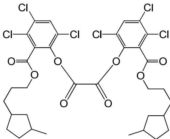
bis(3,4,6-trichloro-2-[[3-(3-methylcyclopentyl)propoxy]carbonyl]phenyl) oxalate
