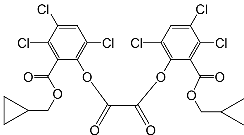
bis{3,4,6-trichloro-2-[(cyclopropylmethoxy)carbonyl]phenyl} oxalate
