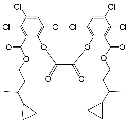
bis{3,4,6-trichloro-2-[(3-cyclopropylbutoxy)carbonyl]phenyl} oxalate
