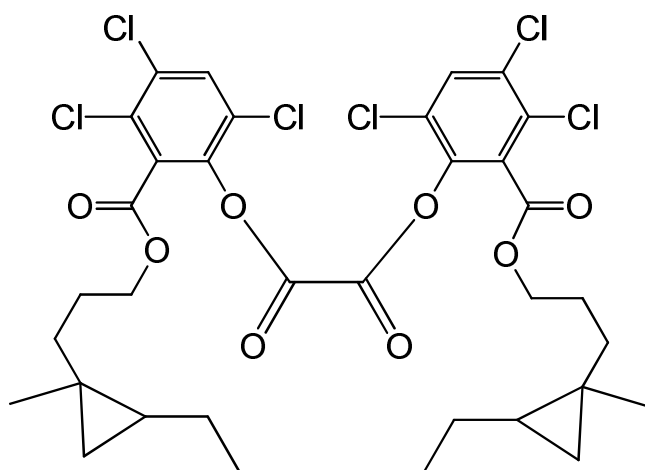
bis(3,4,6-trichloro-2-[[3-(2-ethyl-1-methylcyclopropyl)propoxy]carbonyl]phenyl) oxalate
