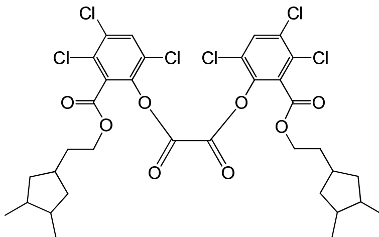
bis(3,4,6-trichloro-2-[[2-(3,4-dimethylcyclopentyl)ethoxy]carbonyl]phenyl) oxalate
