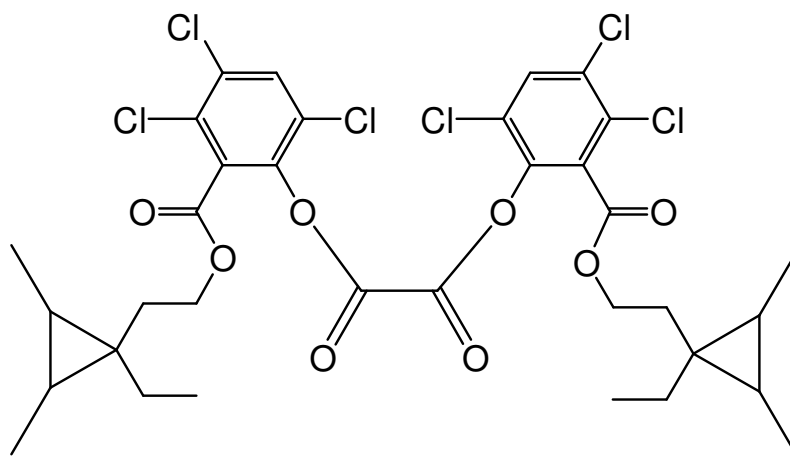
bis(3,4,6-trichloro-2-{[2-(1-ethyl-2,3-dimethylcyclopropyl)ethoxy]carbonyl}phenyl) oxalate
