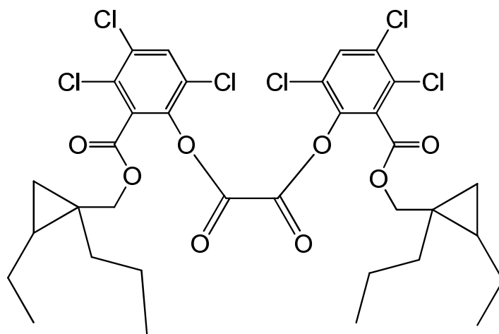
bis(3,4,6-trichloro-2-[(2-ethyl-1-propylcyclopropyl)methoxy]carbonyl)phenyl) oxalate
