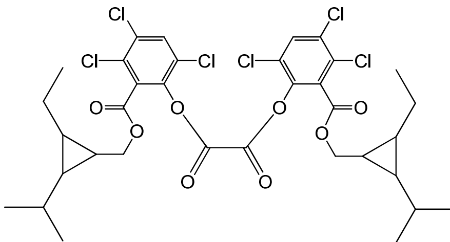
bis[3,4,6-trichloro-2-([2-ethyl-3-(1-methylethyl)-cyclopropyl]methoxy)carbonyl]phenyl] oxalate
