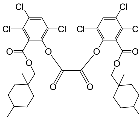
bis(3,4,6-trichloro-2-{[(1,4-dimethylcyclohexyl)methoxy]carbonyl}phenyl) oxalate
