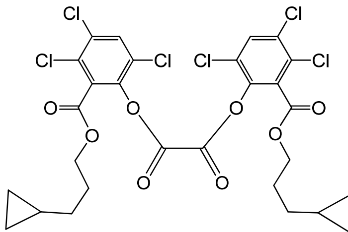
bis{3,4,6-trichloro-2-[(3-cyclopropylpropoxy)carbonyl]phenyl} oxalate
