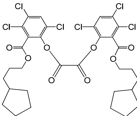
bis{3,4,6-trichloro-2-[(3-cyclopentylpropoxy)carbonyl]phenyl} oxalate
