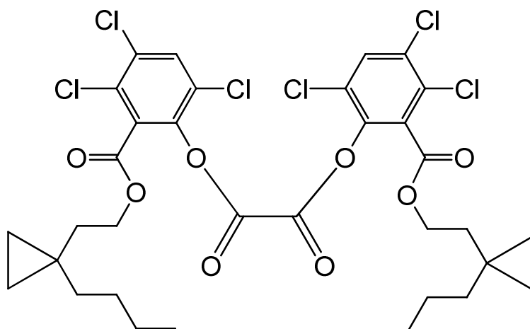
bis(3,4,6-trichloro-2-{{2-[1-butylcyclopropyl]ethoxy}carbonyl}phenyl) oxalate
