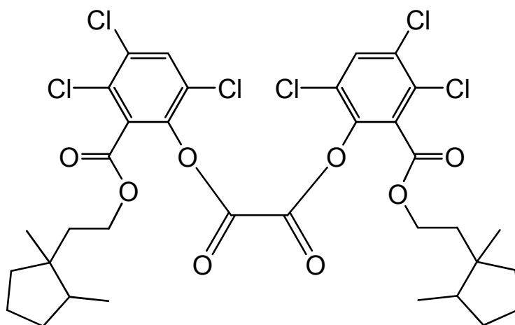
bis(3,4,6-trichloro-2-{{[2-(1,2-dimethylcyclopentyl)ethoxy]carbonyl}}phenyl) oxalate
