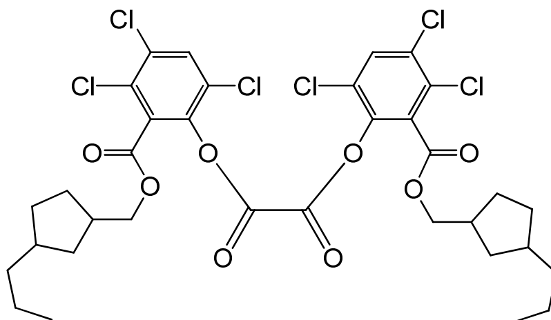
bis(3,4,6-trichloro-2-{[(3-propylcyclopentyl)methoxy]carbonyl}phenyl) oxalate
