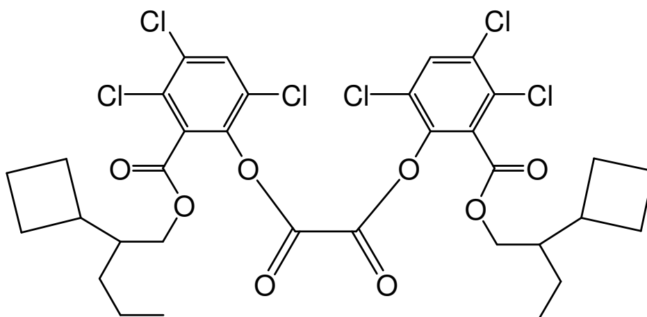
bis{3,4,6-trichloro-2-[(2-cyclobutylpentyl)oxy]carbonyl}phenyl} oxalate
