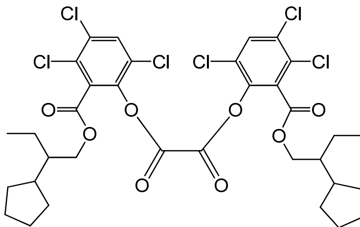
bis{3,4,6-trichloro-2-[(2-cyclopentylbutoxy)carbonyl]phenyl} oxalate
