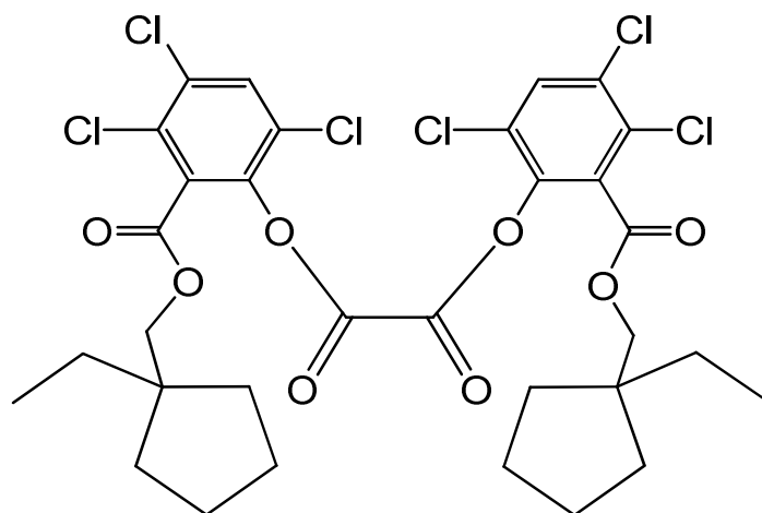
bis(3,4,6-trichloro-2-[(1-ethylcyclopentyl)methoxy]carbonyl)phenyl oxalate
