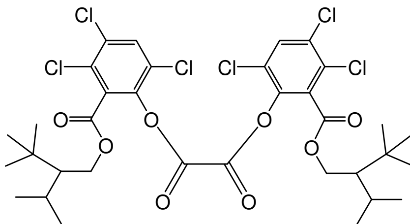
bis(3,4,6-trichloro-2-{[3,3-dimethyl-2-(1-methylethyl)butoxy]carbonyl}phenyl) oxalate
