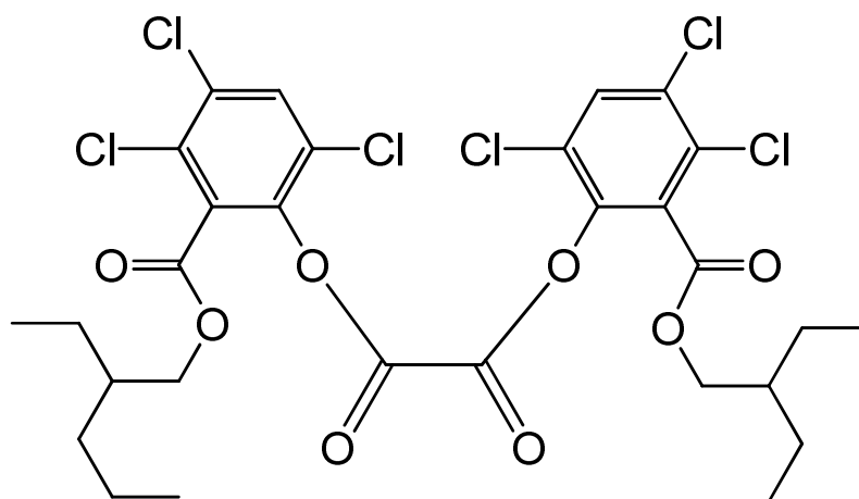
bis{3,4,6-trichloro-2-[(2-ethylpentyloxy)carbonyl]phenyl} oxalate
