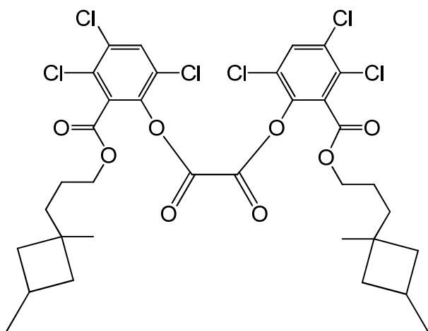
bis(3,4,6-trichloro-2-{[3-(1,3-dimethylcyclobutyl)propoxy]carbonyl}phenyl) oxalate
