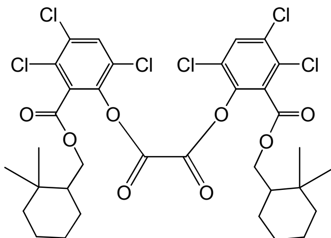
bis(3,4,6-trichloro-2-[(2,2-dimethylcyclohexyl)methoxy]carbonyl)phenyl) oxalate
