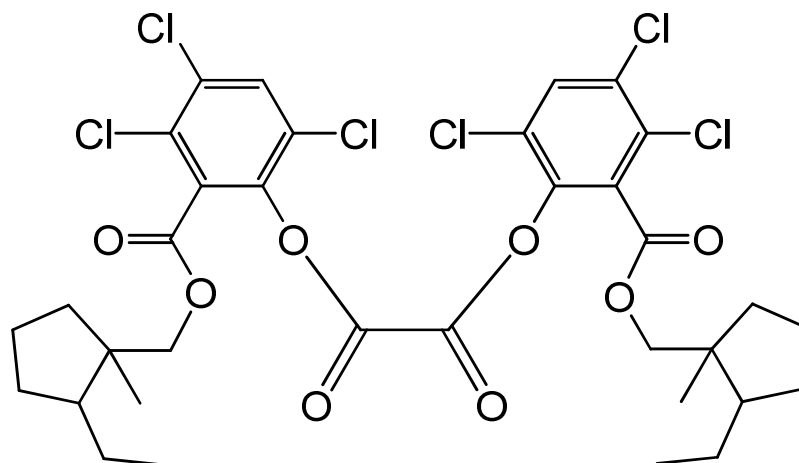
bis(3,4,6-trichloro-2-[(2-ethyl-1-methylcyclopentyl)methoxy]carbonyl)phenyl oxalate
