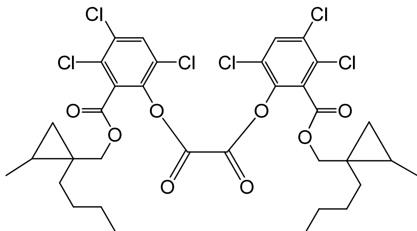
bis(3,4,6-trichloro-2-[(1-butyl-2-methylcyclopropyl)methoxy]carbonyl)phenyl oxalate
