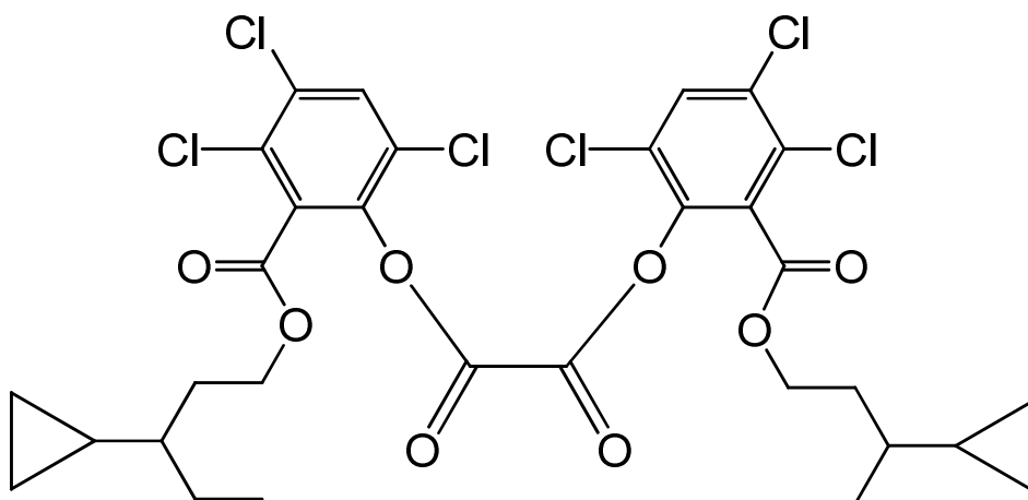
bis{3,4,6-trichloro-2-[(3-cyclopropylpentyl)oxy]carbonyl}phenyl oxalate
