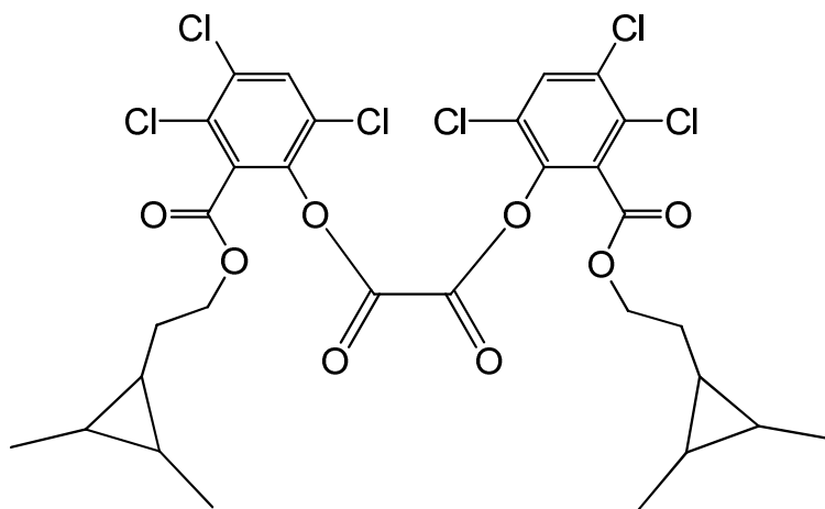
bis(3,4,6-trichloro-2-{[2-(2,3-dimethylcyclopropyl)ethoxy]carbonyl}phenyl) oxalate
