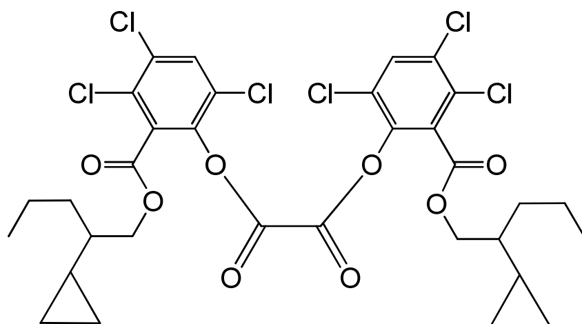
bis{3,4,6-trichloro-2-[(2-cyclopropylpentyl)oxy]carbonyl}phenyl oxalate
