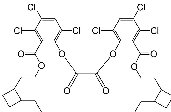
bis(3,4,6-trichloro-2-{{2-(2-propylcyclobutyl)ethoxy}carbonyl}phenyl) oxalate
