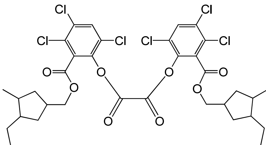
bis(3,4,6-trichloro-2-[(3-ethyl-4-methylcyclopentyl)methoxy]carbonyl)phenyl) oxalate
