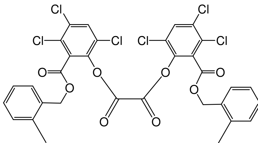
bis(3,4,6-trichloro-2-([(2-methylphenyl)methoxy]carbonyl)phenyl) oxalate
