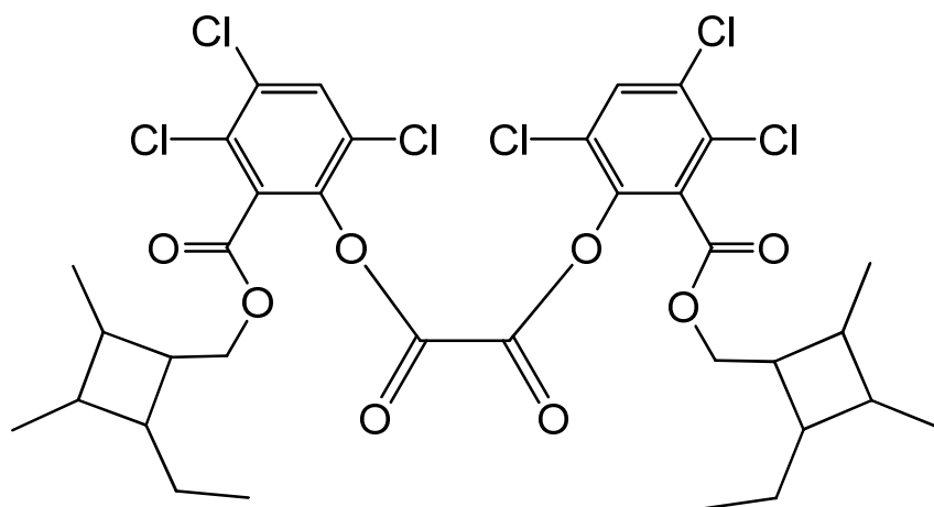
bis(3,4,6-trichloro-2-[(2-ethyl-3,4-dimethylcyclobutyl)methoxy]carbonyl)phenyl) oxalate
