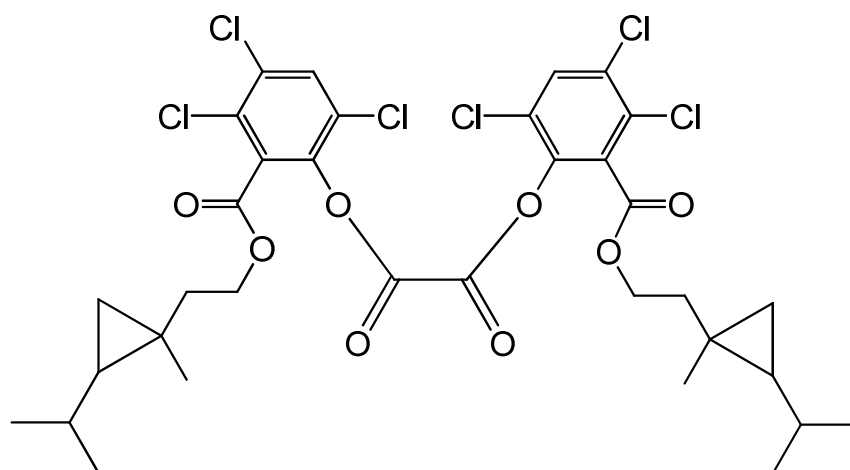
bis[3,4,6-trichloro-2-(2-[1-methyl-2-(1-methylethyl)cyclopropyl]ethoxy)carbonyl]phenyl] oxalate
