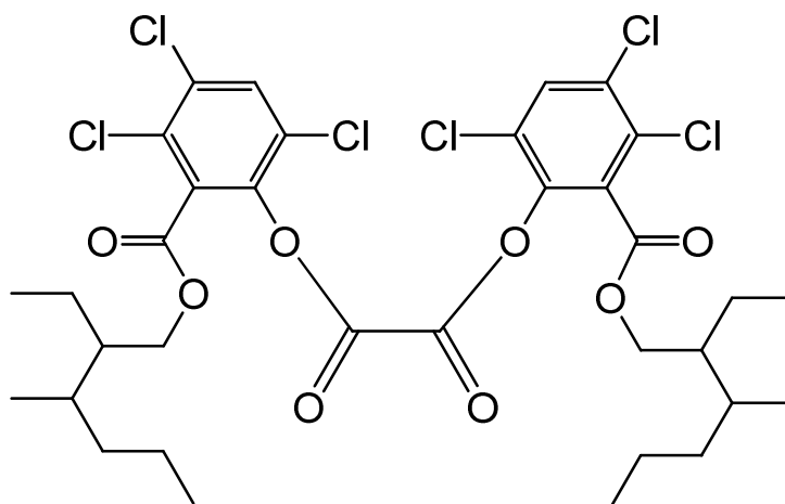
bis{3,4,6-trichloro-2-[(2-ethyl-2-methylhexyloxy)carbonyl]phenyl} oxalate
