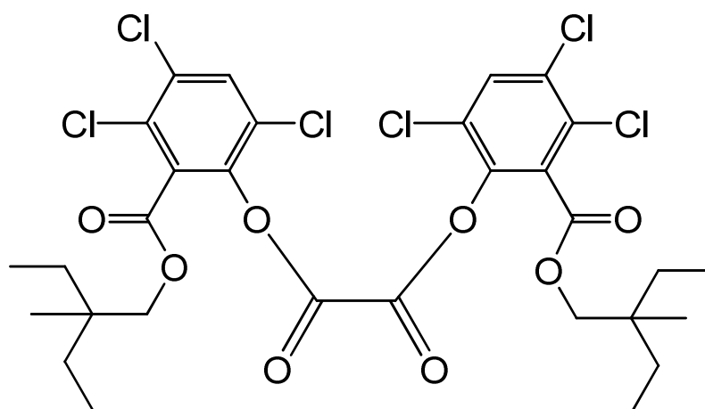
bis{3,4,6-trichloro-2-[(2-ethyl-2-methylbutoxy)carbonyl]phenyl} oxalate
