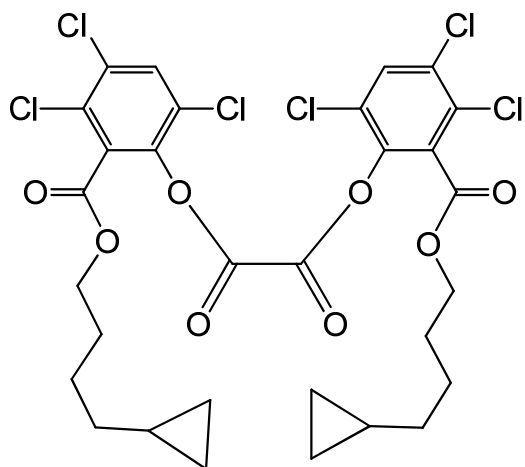
bis{3,4,6-trichloro-2-[(4-cyclopropylbutoxy)carbonyl]phenyl} oxalate
