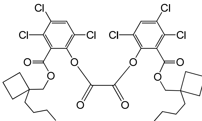
bis(3,4,6-trichloro-2-[(1-butylcyclobutyl)methoxy]carbonyl)phenyl oxalate
