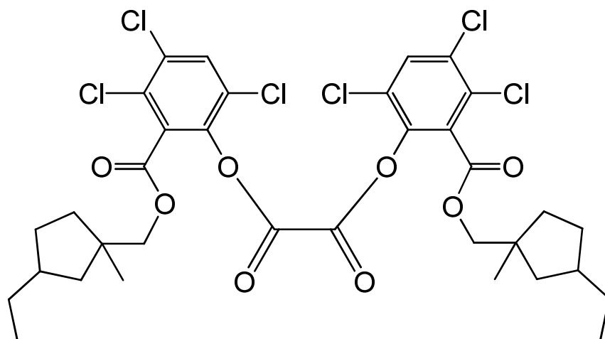
bis(3,4,6-trichloro-2-[(3-ethyl-1-methylcyclopentyl)methoxy]carbonyl)phenyl) oxalate
