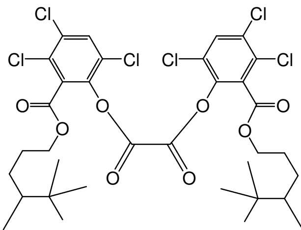
bis{3,4,6-trichloro-2-[(4,5,5-trimethylhexyloxy)carbonyl]phenyl} oxalate
