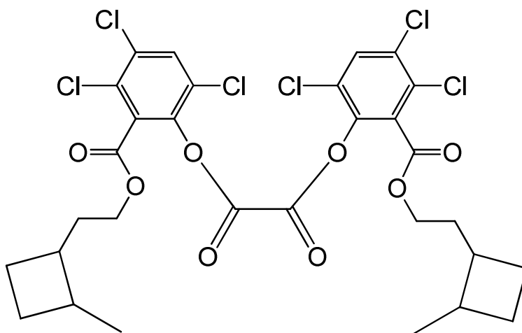
bis(3,4,6-trichloro-2-[[2-(2-methylcyclobutyl)ethoxy]carbonyl]phenyl) oxalate
