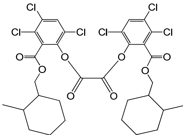
bis(3,4,6-trichloro-2-[[2-methylcyclohexyl)methoxy]carbonyl]phenyl oxalate
