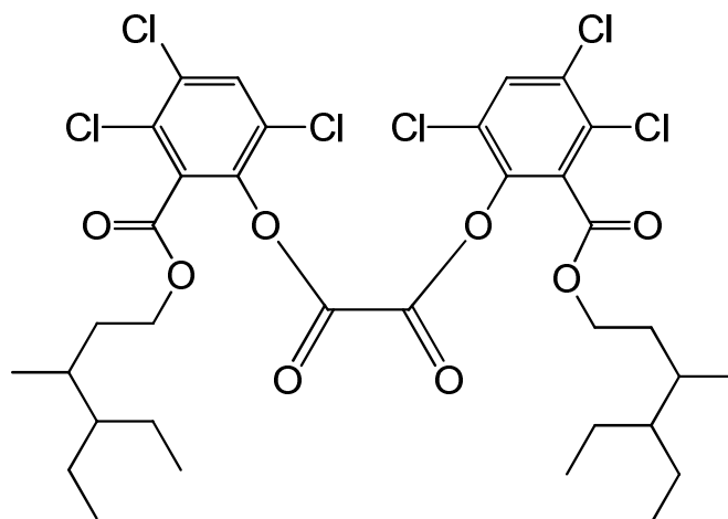
bis{3,4,6-trichloro-2-[(4-ethyl-3-methylhexyloxy)carbonyl]phenyl} oxalate
