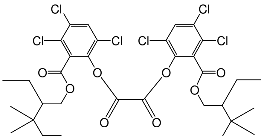
bis{3,4,6-trichloro-2-[(2-ethyl-3,3-dimethylpentyloxy)carbonyl]phenyl} oxalate
