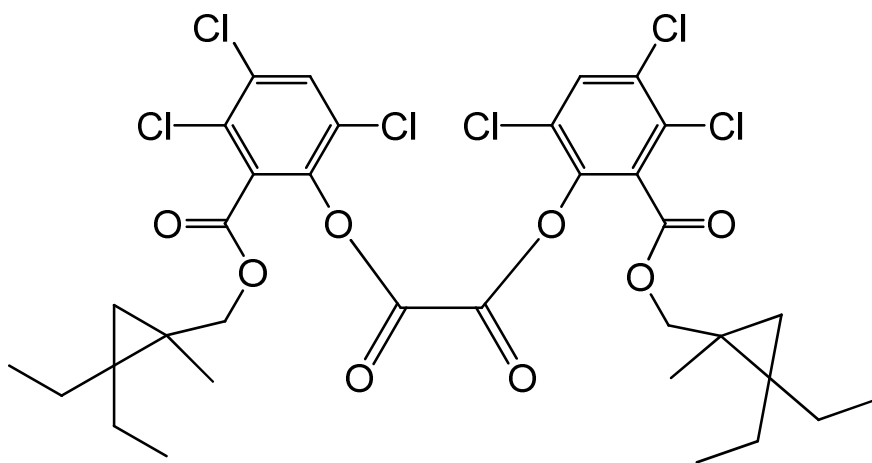
bis(3,4,6-trichloro-2-[(2,2-diethyl-1-methylcyclopropyl)methoxy]carbonyl)phenyl oxalate
