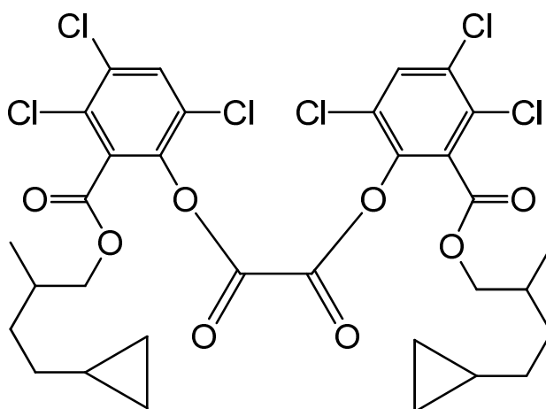
bis{3,4,6-trichloro-2-[(4-cyclopropyl-2-methylbutoxy)carbonyl]phenyl} oxalate
