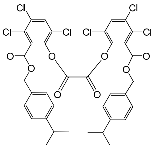
bis[3,4,6-trichloro-2-([4-(1-methylethyl)phenyl]methoxy)carbonyl]phenyl) oxalate
