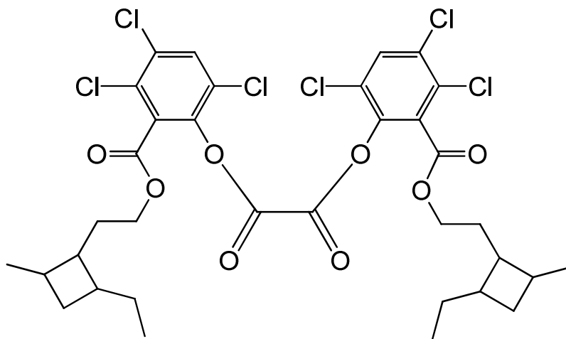
bis(3,4,6-trichloro-2-[[2-(2-ethyl-4-methylcyclobutyl)ethoxy]carbonyl]phenyl) oxalate
