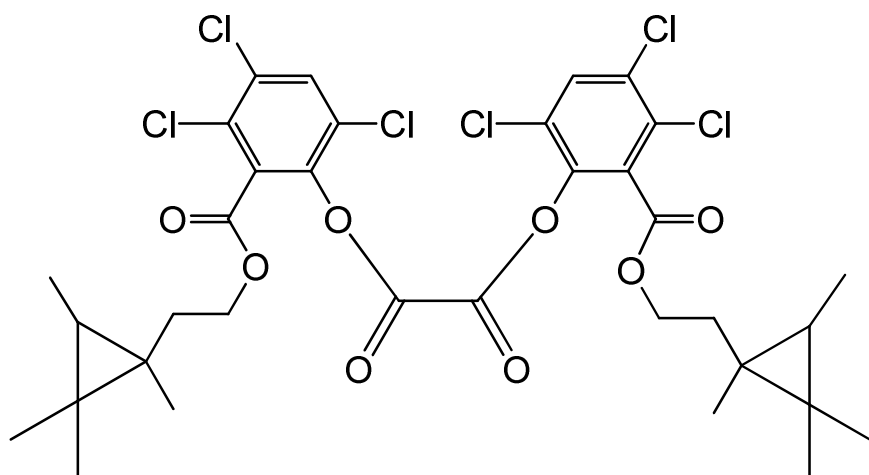
bis(3,4,6-trichloro-2-{[2-(1,2,2,3-tetramethylcyclopropyl)ethoxy]carbonyl}phenyl) oxalate
