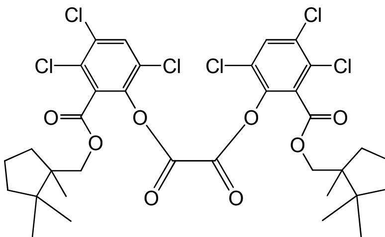
bis(3,4,6-trichloro-2-[(1,2,2-trimethylcyclopentyl)methoxy]carbonyl]phenyl) oxalate
