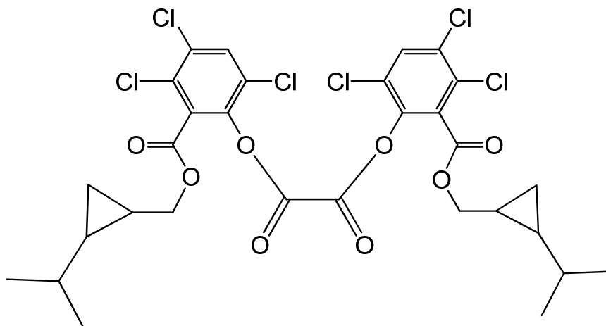
bis[3,4,6-trichloro-2-([2-(1-methyl-ethyl)cyclopropyl]methoxy)carbonyl]phenyl] oxalate
