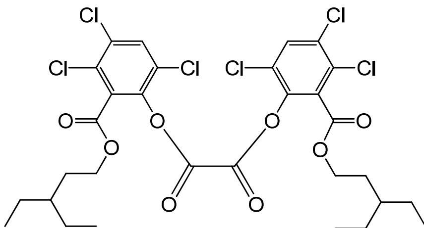
bis{3,4,6-trichloro-2-[(3-ethylpentyloxy)carbonyl]phenyl} oxalate
