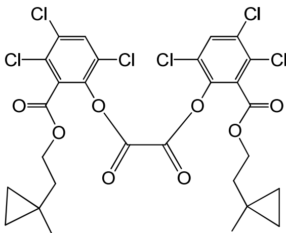
bis(3,4,6-trichloro-2-[[2-(1-methylcyclopropyl)ethoxy]carbonyl]phenyl) oxalate
