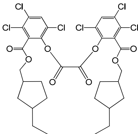
bis(3,4,6-trichloro-2-[(3-ethylcyclopentyl)methoxy]carbonyl)phenyl) oxalate
