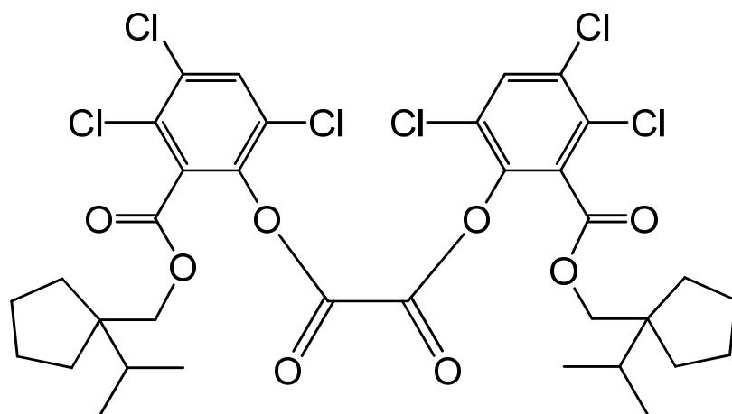
bis[3,4,6-trichloro-2-({[1-(1-methylethyl)-cyclopentyl]methoxy}carbonyl)phenyl] oxalate
