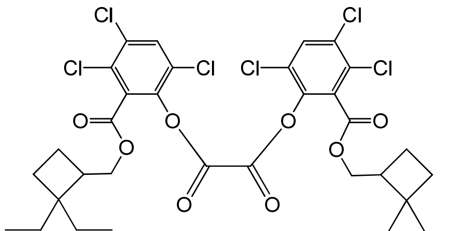
bis(3,4,6-trichloro-2-[[2,2-diethylcyclobutyl)methoxy]carbonyl}phenyl) oxalate
