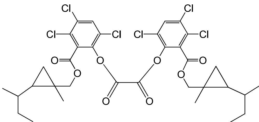
bis[3,4,6-trichloro-2-([1-methyl-2-(1-methylpropyl)cyclopropyl]methoxy)carbonyl]phenyl) oxalate
