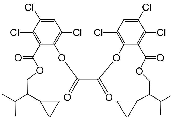
bis{3,4,6-trichloro-2-[(2-cyclopropyl-3-methylbutoxy)carbonyl]phenyl} oxalate
