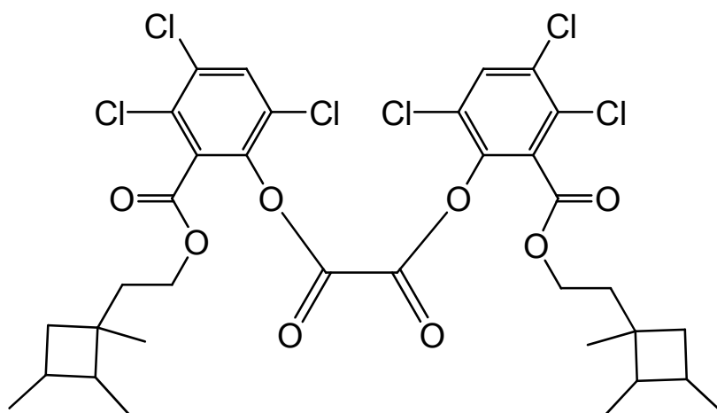
bis(3,4,6-trichloro-2-{[2-(1,2,3-trimethylcyclobutylethoxy)]carbonyl}phenyl) oxalate
