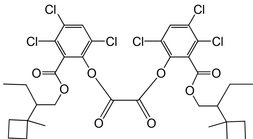
bis(3,4,6-trichloro-2-[[2-(1-methylcyclobutyl)butoxy]carbonyl]phenyl) oxalate
