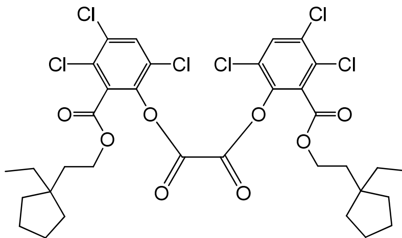
bis(3,4,6-trichloro-2-[[2-(1-ethylcyclopentyl)ethoxy]carbonyl]phenyl) oxalate
