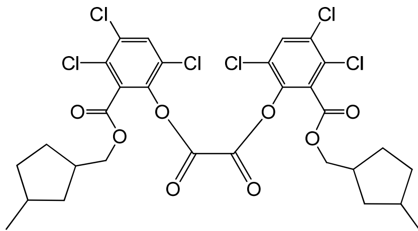
bis(3,4,6-trichloro-2-{[(3-methylcyclopentyl)methoxy]carbonyl}phenyl) oxalate
