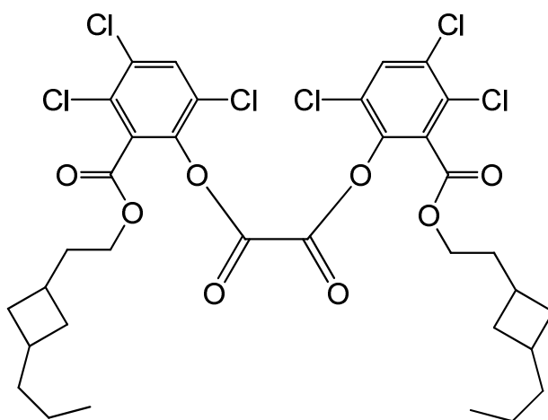
bis(3,4,6-trichloro-2-[[2-(3-propylcyclobutyl)ethoxy]carbonyl]phenyl) oxalate
