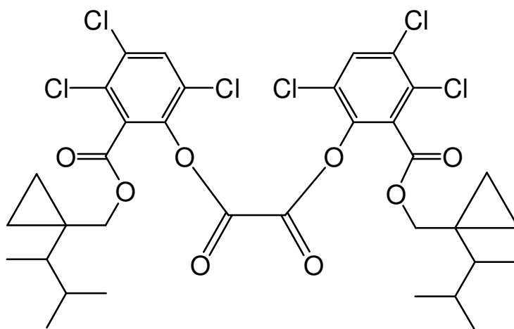
bis[3,4,6-trichloro-2-([1-(1,2-dimethylpropyl)cyclopropyl]methoxy)carbonyl]phenyl] oxalate
