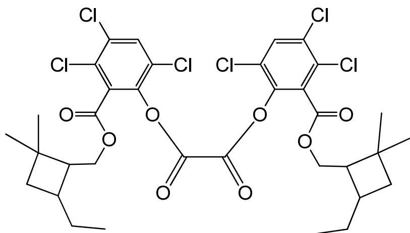
bis(3,4,6-trichloro-2-[[2-ethyl-4,4-dimethylcyclobutyl)methoxy]carbonyl)phenyl) oxalate
