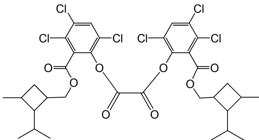
bis[3,4,6-trichloro-2-({[3-methyl-2-(1-methylethyl)cyclobutyl]methoxy}carbonyl)phenyl] oxalate
