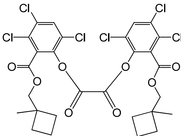
bis(3,4,6-trichloro-2-[[1-methylcyclobutyl)methoxy]carbonyl]phenyl) oxalate
