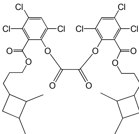
bis(3,4,6-trichloro-2-{[3-(2,3-dimethylcyclobutyl)propoxy]carbonyl}phenyl) oxalate
