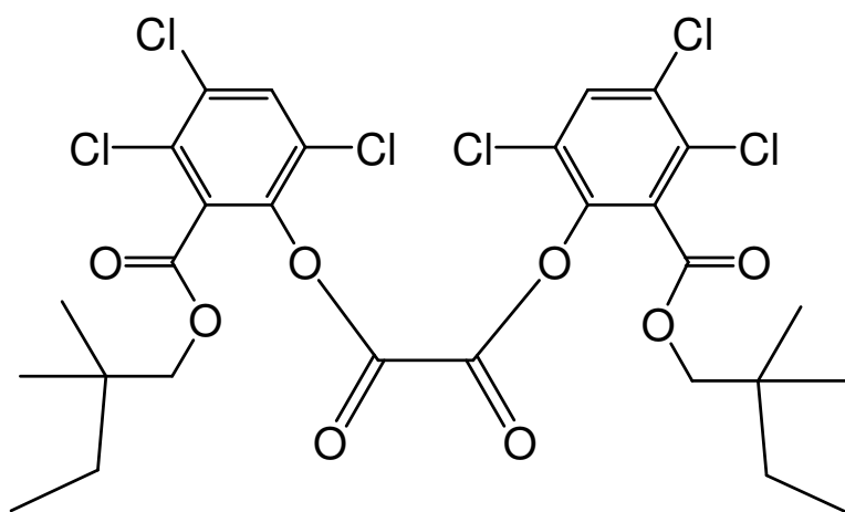
bis{3,4,6-trichloro-2-[(2,2-dimethylbutoxy)carbonyl]phenyl} oxalate
