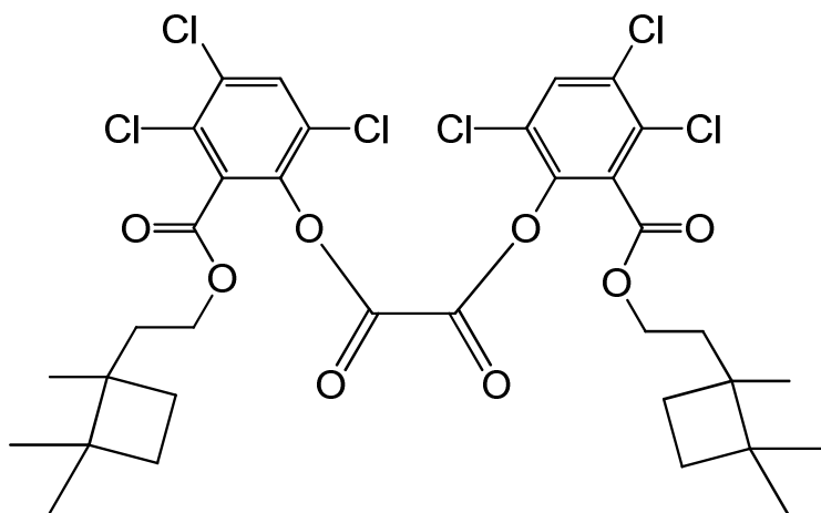
bis(3,4,6-trichloro-2-{[2-(1,2,2-trimethylcyclobutyl)ethoxy]carbonyl}phenyl) oxalate
