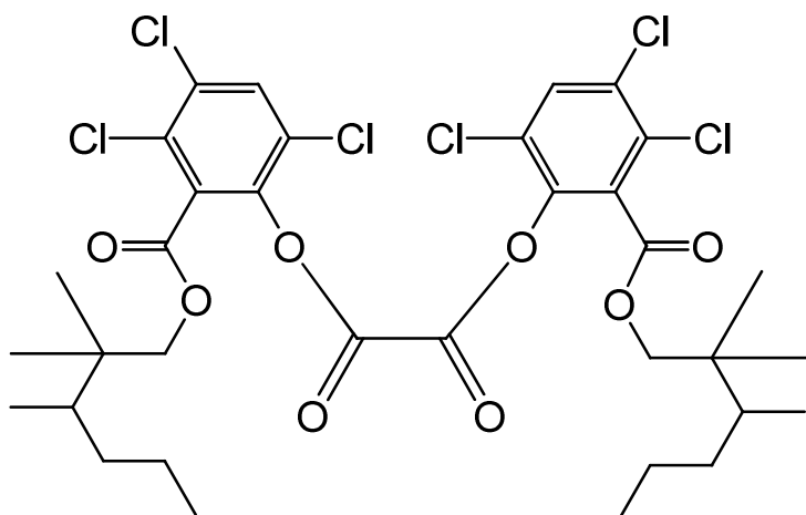
bis{3,4,6-trichloro-2-[(2,2,3-trimethylhexyloxy)carbonyl]phenyl} oxalate
