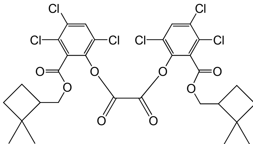
bis(3,4,6-trichloro-2-{[(2,2-dimethylcyclobutyl)methoxy]carbonyl}phenyl) oxalate
