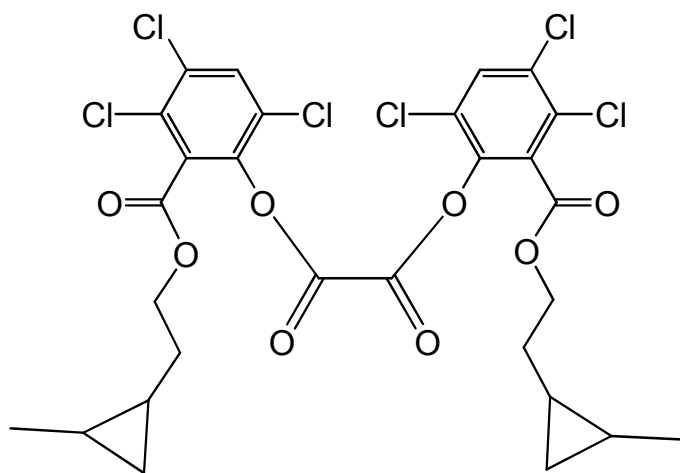
bis(3,4,6-trichloro-2-{[2-(2-methylcyclopropyl)ethoxy]carbonyl}phenyl) oxalate
