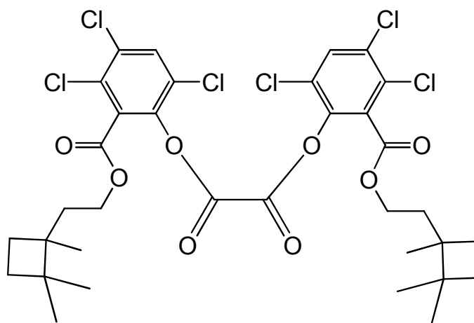
bis(3,4,6-trichloro-2-{[2-(1,2,2-trimethylcyclobutylethoxy]carbonyl}phenyl) oxalate
