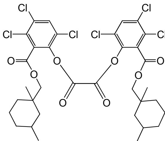
bis(3,4,6-trichloro-2-{[(1,3-dimethylcyclohexyl)methoxy]carbonyl}phenyl) oxalate
