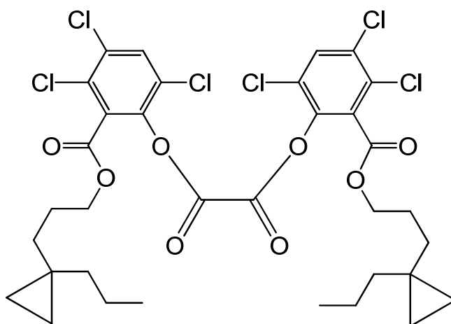
bis(3,4,6-trichloro-2-{[3-(1-propylcyclopropyl)propoxy]carbonyl}phenyl) oxalate
