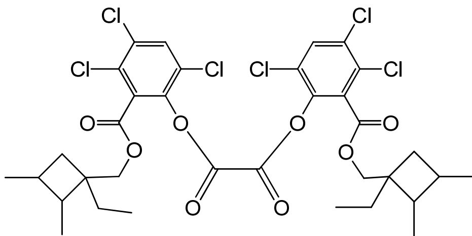
bis(3,4,6-trichloro-2-([(1-ethyl-2,3-dimethylcyclobutyl)methoxy]carbonyl)phenyl) oxalate
