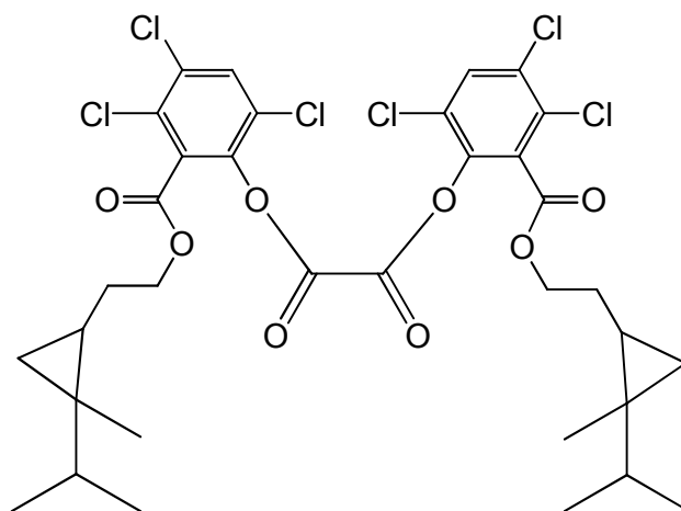
bis[3,4,6-trichloro-2-({2-[2-methyl-1-(1-methylethyl)cyclopropyl]ethoxy}carbonyl)phenyl] oxalate
