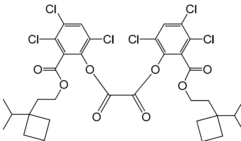
bis[3,4,6-trichloro-2-((2-[1-(1-methylethyl)cyclobutyl]ethoxy)carbonyl)phenyl] oxalate
