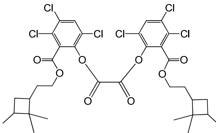
bis(3,4,6-trichloro-2-{[2-(2,2,3-trimethylcyclobutylethoxy)]carbonyl}phenyl) oxalate
