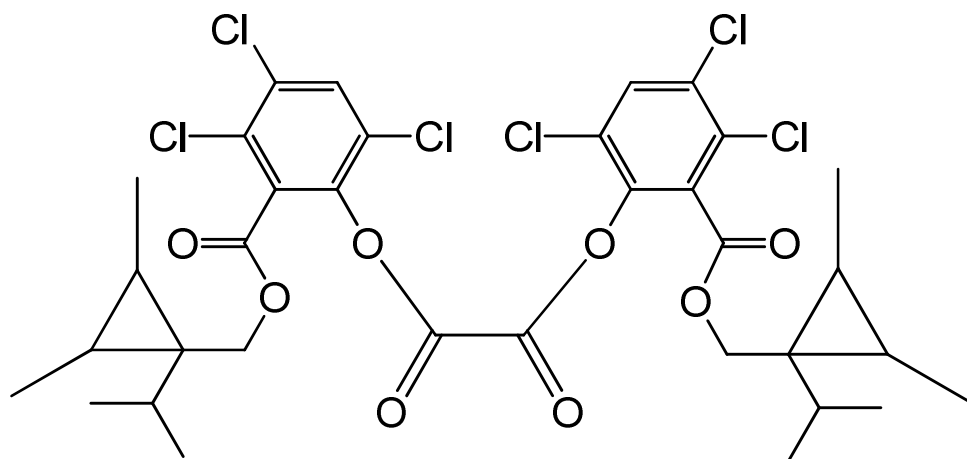
bis[3,4,6-trichloro-2-({[2,3-dimethyl-1-(1-methylethyl)cyclopropyl]methoxy}carbonyl)phenyl] oxalate
