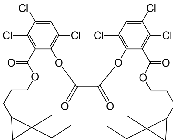
bis(3,4,6-trichloro-2-{[3-(2-ethyl-2-methylcyclopropyl)propoxy]carbonyl}phenyl) oxalate
