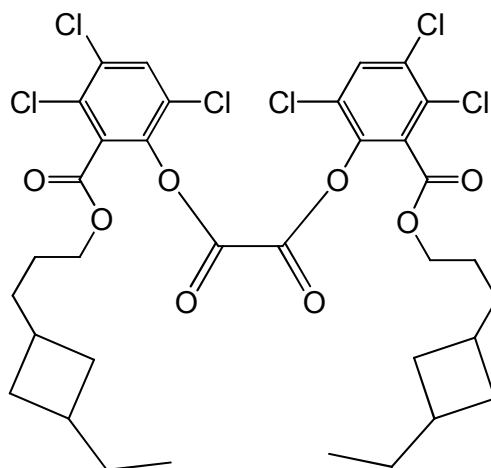
bis(3,4,6-trichloro-2-{[3-(3-ethylcyclobutylpropoxy)]carbonyl}phenyl) oxalate
