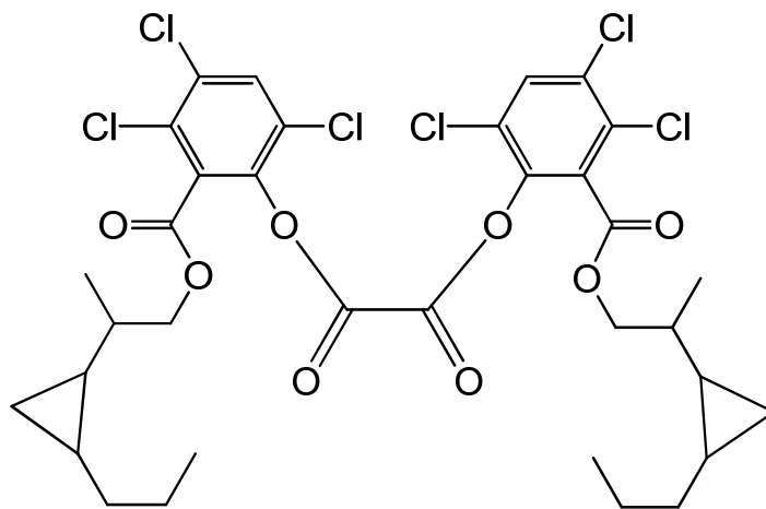
bis(3,4,6-trichloro-2-([2-(2-propylcyclopropyl)propoxy]carbonyl)phenyl) oxalate
