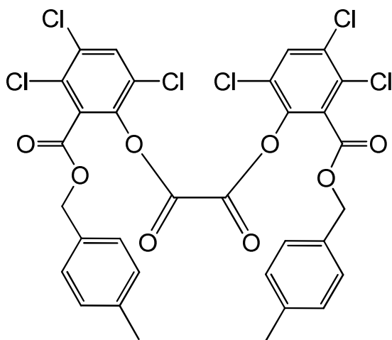
bis(3,4,6-trichloro-2-[[4-methylphenyl)methoxy]carbonyl}phenyl) oxalate
