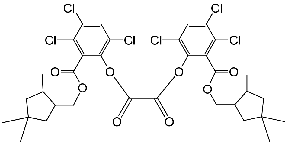
bis(3,4,6-trichloro-2-[[2,4,4-trimethylcyclopentyl)methoxy]carbonyl}phenyl) oxalate
