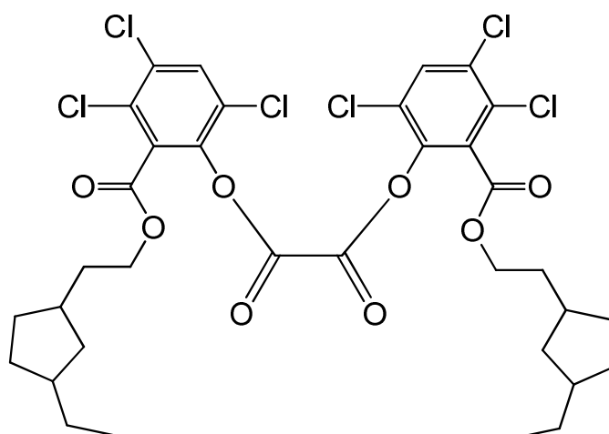
bis(3,4,6-trichloro-2-{[2-(3-ethylcyclopentyl)ethoxy]carbonyl}phenyl) oxalate
