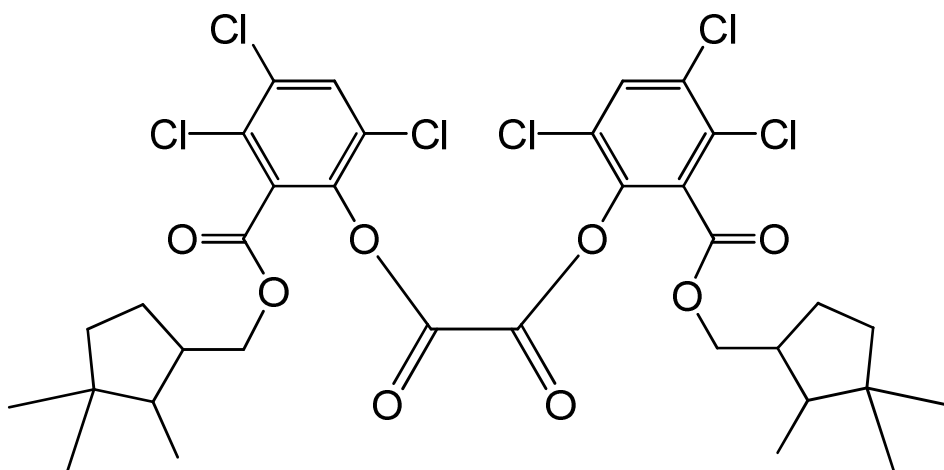
bis(3,4,6-trichloro-2-[[2,3,3-trimethylcyclopentyl)methoxy]carbonyl}phenyl) oxalate
