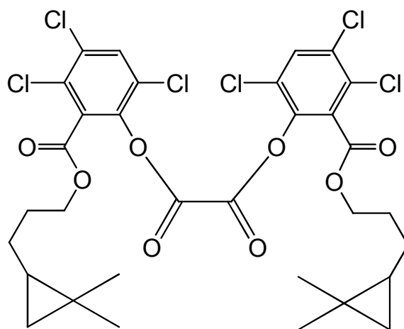
bis(3,4,6-trichloro-2-{{[3-(2,2-dimethylcyclopropyl)propoxy]carbonyl}phenyl}) oxalate
