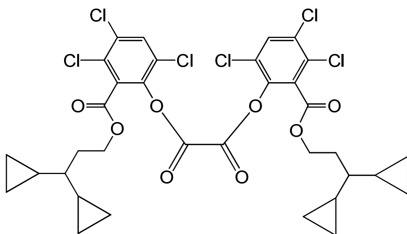
bis{3,4,6-trichloro-2-[(3,3-dicyclopropylpropoxy)carbonyl]phenyl} oxalate
