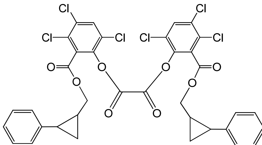
bis(3,4,6-trichloro-2-[(2-phenylcyclopropyl)methoxy]carbonyl]phenyl) oxalate
