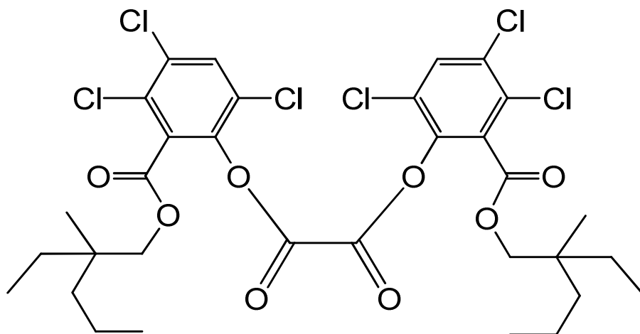
bis{3,4,6-trichloro-2-[(2-ethyl-2-methylpentyloxy)carbonyl]phenyl} oxalate
