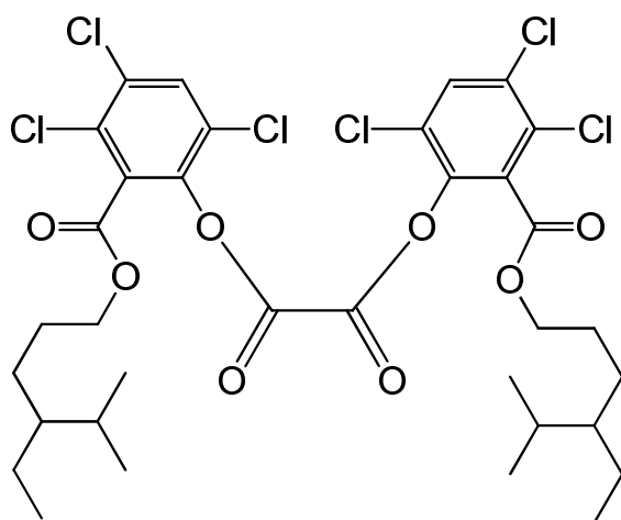
bis{3,4,6-trichloro-2-[(4-ethyl-5-methylhexyloxy)carbonyl]phenyl} oxalate
