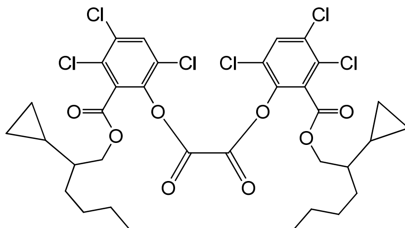
bis{3,4,6-trichloro-2-[(2-cyclopropylhexyloxy)carbonyl]phenyl} oxalate
