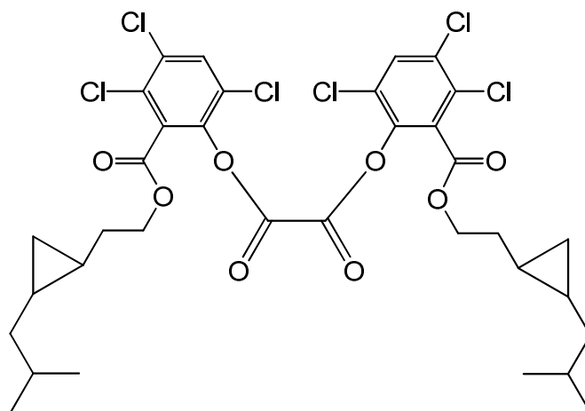
bis[3,4,6-trichloro-2-({2-[2-(2-methylpropyl)cyclopropyl]ethoxy}carbonyl)phenyl] oxalate
