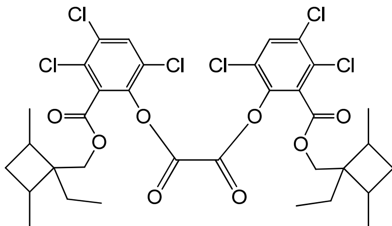
bis(3,4,6-trichloro-2-([(1-ethyl-2,4-dimethylcyclobutyl)methoxy]carbonyl)phenyl) oxalate
