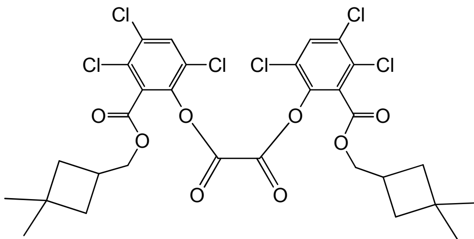
bis(3,4,6-trichloro-2-[(3,3-dimethylcyclobutyl)methoxy]carbonyl)phenyl oxalate
