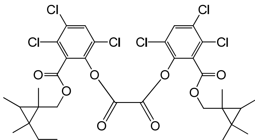
bis(3,4,6-trichloro-2-[[2-ethyl-1,2,3-trimethylcyclopropyl)methoxy]carbonyl}phenyl) oxalate
