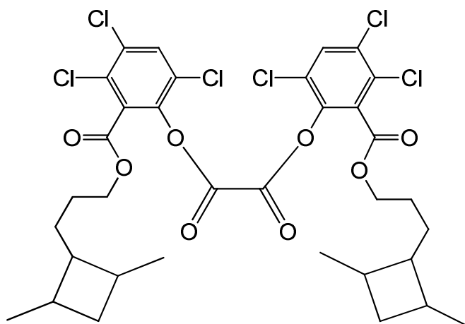
bis(3,4,6-trichloro-2-{[3-(2,4-dimethylcyclobutyl)propoxy]carbonyl}phenyl) oxalate
