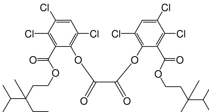
bis{3,4,6-trichloro-2-[(3-ethyl-3,4-dimethylpentyloxy)carbonyl]phenyl} oxalate
