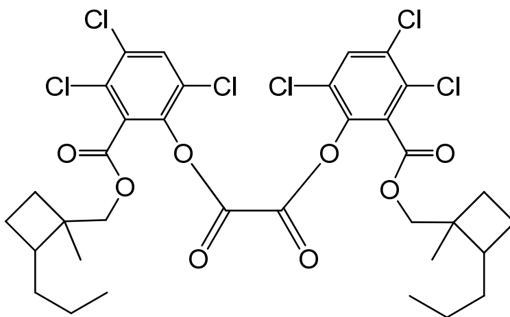
bis(3,4,6-trichloro-2-[[1-methyl-2-propylcyclobutyl)methoxy]carbonyl}phenyl) oxalate
