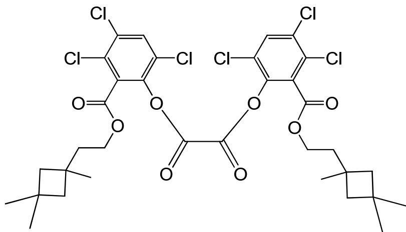
bis(3,4,6-trichloro-2-{[2-(1,3,3-trimethylcyclobutylethoxy)]carbonyl}phenyl) oxalate
