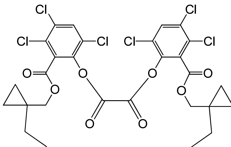
bis(3,4,6-trichloro-2-{[(1-ethylcyclopropyl)methoxy]carbonyl}phenyl) oxalate
