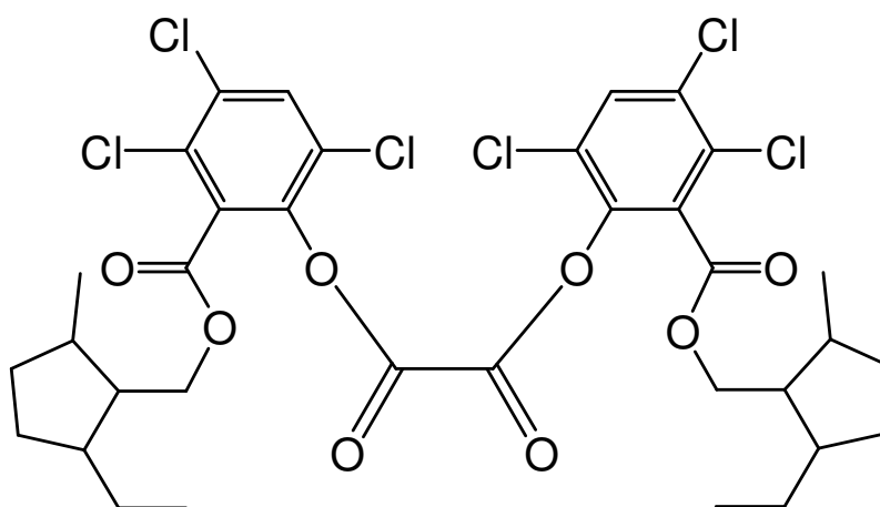
bis(3,4,6-trichloro-2-[(2-ethyl-5-methylcyclopentyl)methoxy]carbonyl)phenyl) oxalate
