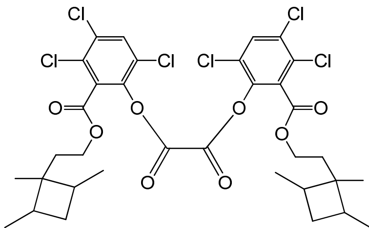
bis(3,4,6-trichloro-2-{[2-(1,2,4-trimethylcyclobutyl)ethoxy]carbonyl}phenyl) oxalate
