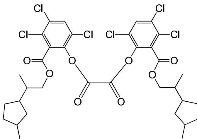
bis(3,4,6-trichloro-2-[[2-(3-methylcyclopentyl)propoxy]carbonyl]phenyl) oxalate
