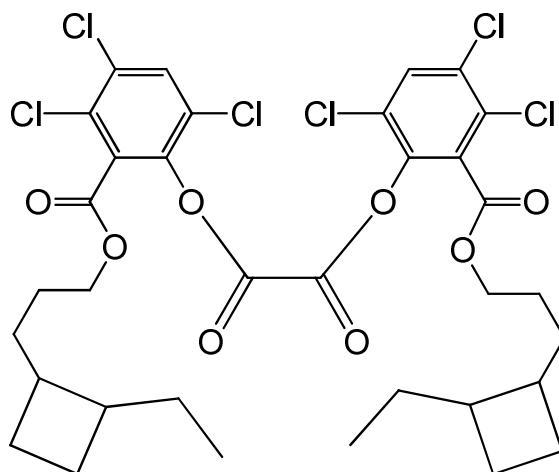
bis(3,4,6-trichloro-2-{[3-(2-ethylcyclobutylpropoxy)]carbonyl}phenyl) oxalate
