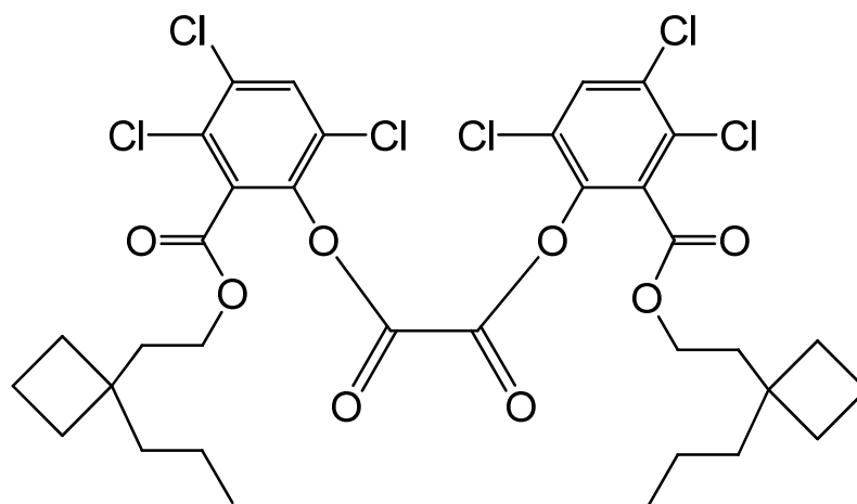
bis(3,4,6-trichloro-2-{{2-(1-propylcyclobutyl)ethoxy}carbonyl}phenyl) oxalate
