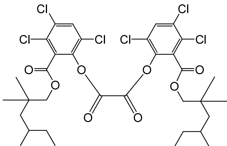
bis{3,4,6-trichloro-2-[(2,2,4-trimethylhexyloxy)carbonyl]phenyl} oxalate
