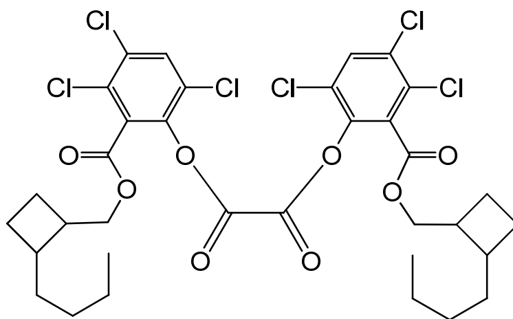
bis(3,4,6-trichloro-2-[(2-butylcyclobutyl)methoxy]carbonyl)phenyl oxalate
