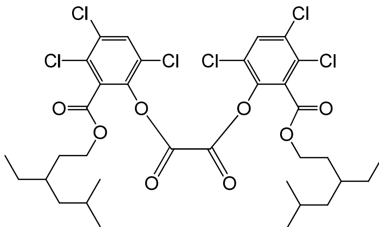
bis{3,4,6-trichloro-2-[(3-ethyl-5-methylhexyloxy)carbonyl]phenyl} oxalate
