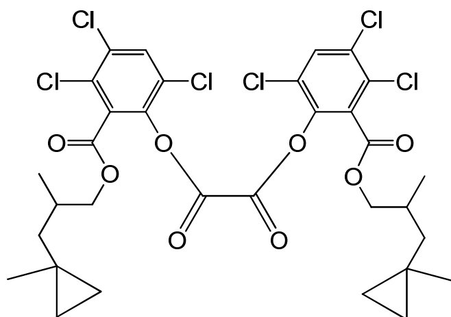
bis(3,4,6-trichloro-2-{[2-methyl-3-(1-methylcyclopropyl)propoxy]carbonyl}phenyl) oxalate
