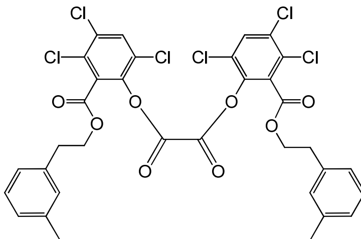
bis(3,4,6-trichloro-2-{[2-(3-methylphenyl)ethoxy]carbonyl}phenyl) oxalate
