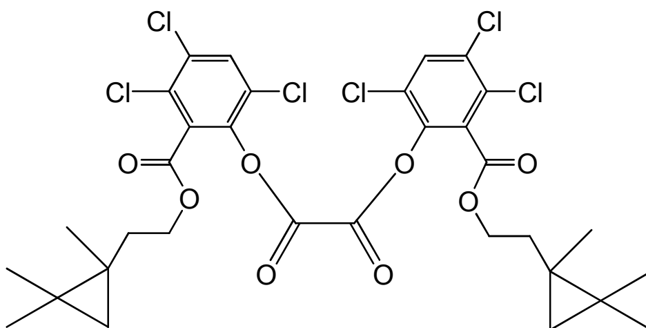
bis(3,4,6-trichloro-2-{[2-(1,2,2-trimethylcyclopropyl)propoxy]carbonyl}phenyl) oxalate
