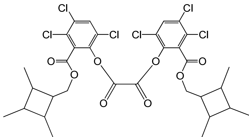
bis(3,4,6-trichloro-2-{[(2,3,4-trimethylcyclobutyl)methoxy]carbonyl}phenyl) oxalate
