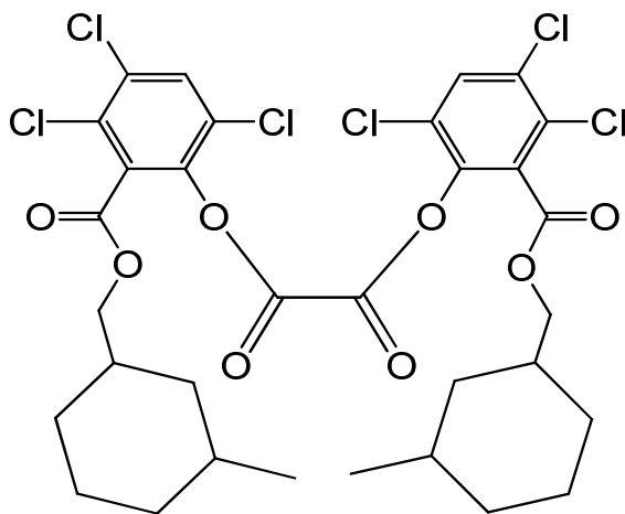
bis(3,4,6-trichloro-2-[[3-methylcyclohexyl)methoxy]carbonyl]phenyl oxalate
