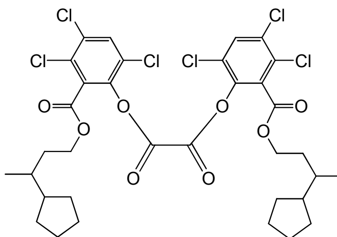
bis{3,4,6-trichloro-2-[(3-cyclopentylbutoxy)carbonyl]phenyl} oxalate
