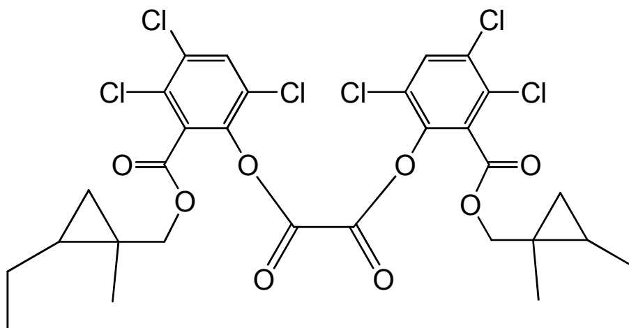
bis(3,4,6-trichloro-2-[(2-ethyl-1-methylcyclopropyl)methoxy]carbonyl)phenyl oxalate
