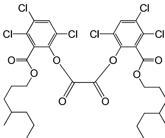
bis{3,4,6-trichloro-2-[(4-methylheptyloxy)carbonyl]phenyl} oxalate
