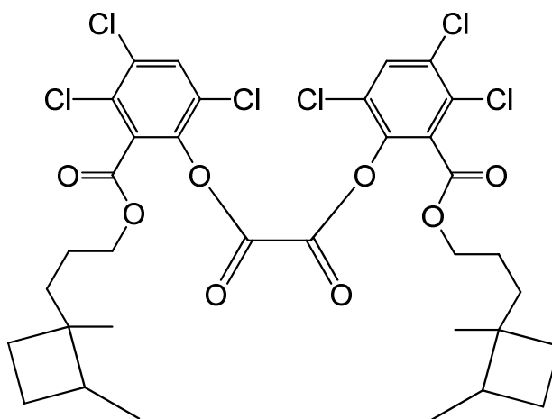
bis(3,4,6-trichloro-2-{[3-(1,2-dimethylcyclobutylpropoxy)]carbonyl}phenyl) oxalate
