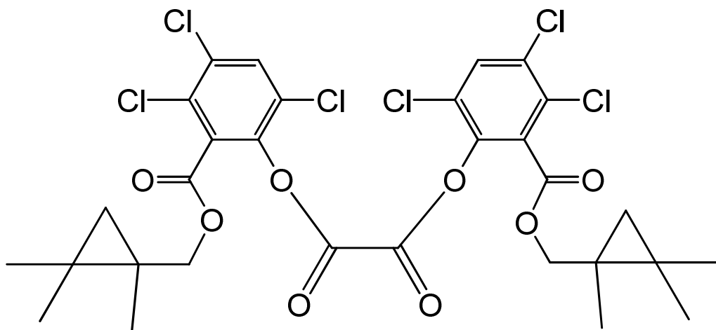
bis(3,4,6-trichloro-2-[[1,2,2-trimethylcyclopropyl)methoxy]carbonyl}phenyl) oxalate
