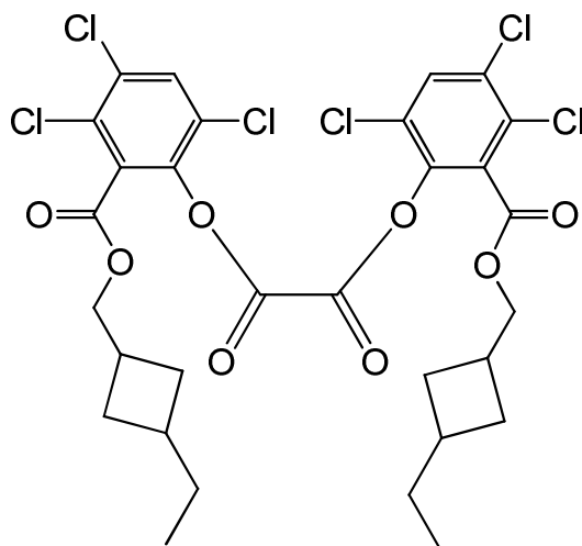
bis(3,4,6-trichloro-2-[(3-ethylcyclobutyl)methoxy]carbonyl)phenyl oxalate
