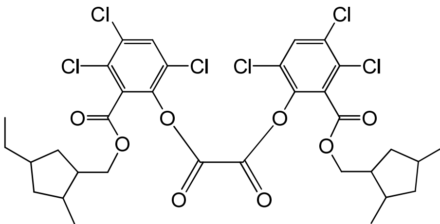
bis(3,4,6-trichloro-2-[(4-ethyl-2-methylcyclopentyl)methoxy]carbonyl)phenyl) oxalate
