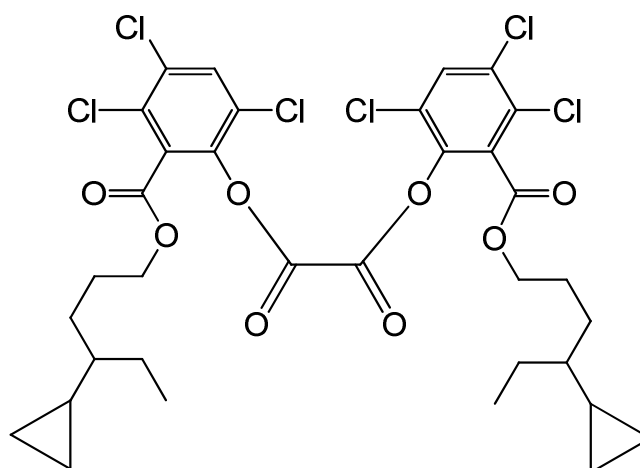
bis{3,4,6-trichloro-2-[(4-cyclopropylhexyloxy)carbonyl]phenyl} oxalate
