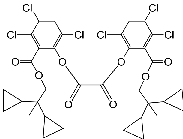
bis{3,4,6-trichloro-2-[(2,2-dicyclopropylpropoxy)carbonyl]phenyl} oxalate
