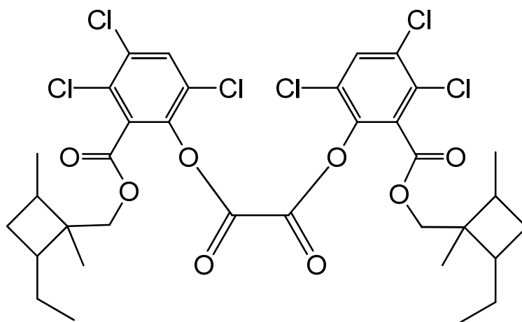
bis(3,4,6-trichloro-2-{[(2-ethyl-1,4-dimethylcyclobutyl)methoxy]carbonyl}phenyl) oxalate
