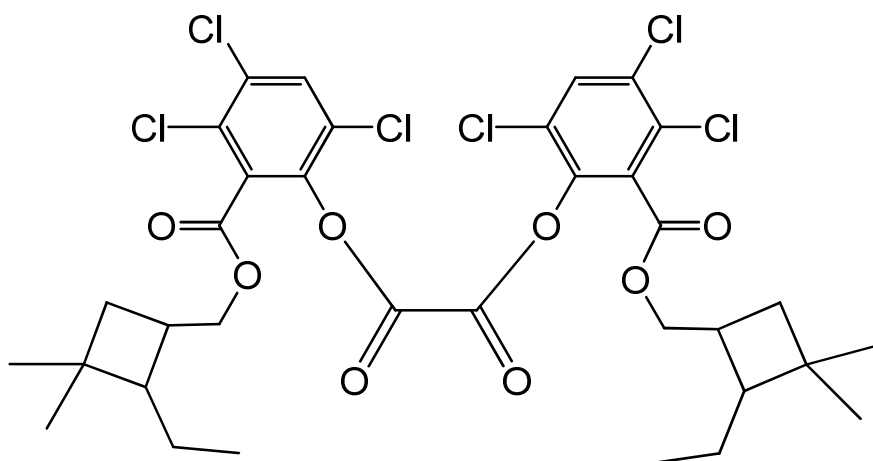
bis(3,4,6-trichloro-2-[(2-ethyl-3,3-dimethylcyclobutyl)methoxy]carbonyl)phenyl) oxalate
