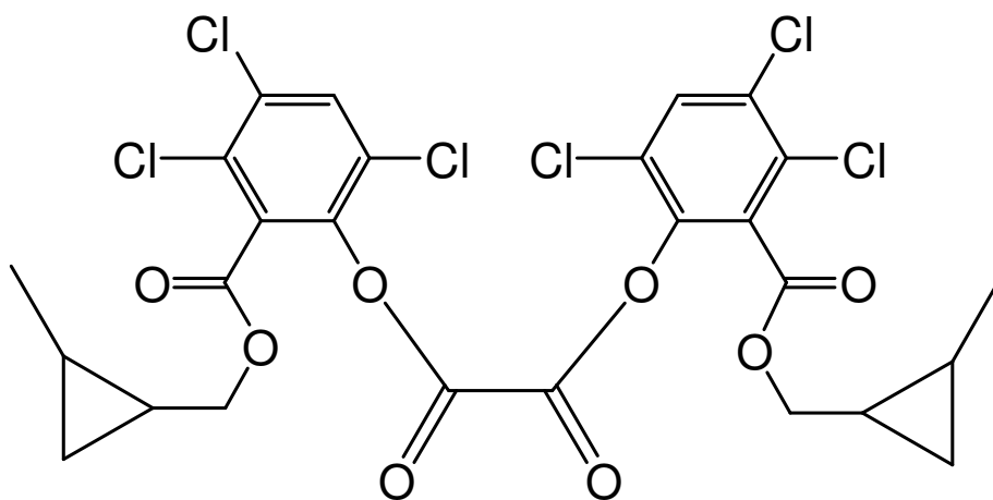
bis(3,4,6-trichloro-2-[[2-methylcyclopropyl)methoxy]carbonyl)phenyl) oxalate
