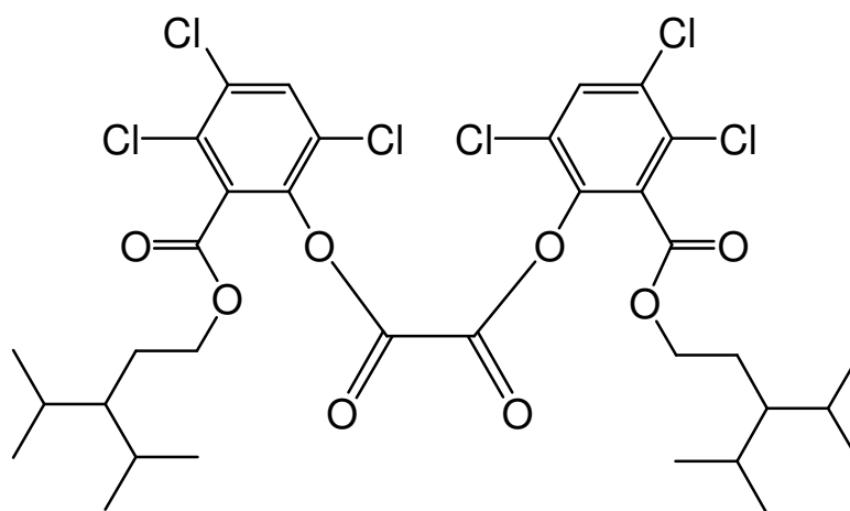
bis(3,4,6-trichloro-2-{[4-methyl-3-(1-methylethyl)pentyloxy]carbonyl}phenyl) oxalate
