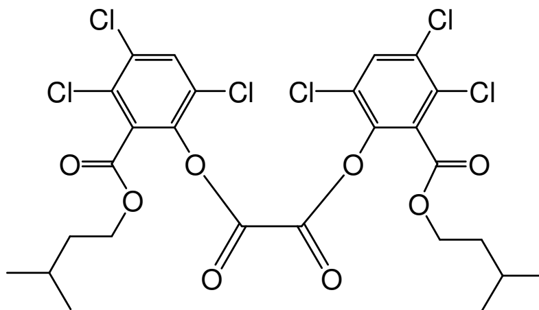
bis{3,4,6-trichloro-2-[(3-methylbutoxy)carbonyl]phenyl} oxalate
