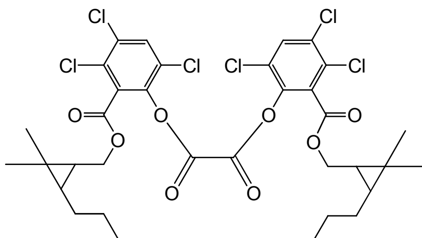
bis(3,4,6-trichloro-2-[[2,2-dimethyl-3-propylcyclopropyl)methoxy]carbonyl}phenyl) oxalate
