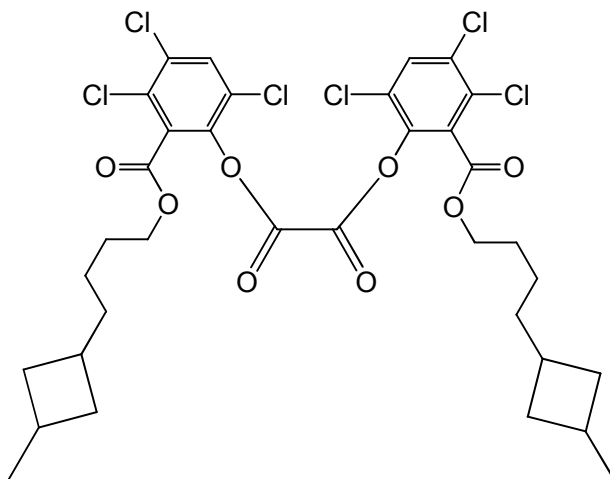
bis(3,4,6-trichloro-2-{[4-(3-methylcyclobutyl)butoxy]carbonyl}phenyl) oxalate
