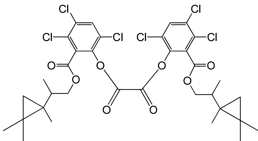
bis[3,4,6-trichloro-2-({2-[2-(1,2,2-trimethylcyclopropyl)propoxy]carbonyl}phenyl) oxalate
