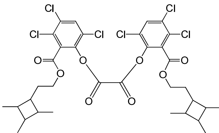
bis(3,4,6-trichloro-2-{[2-(2,3,4-trimethylcyclobutyl)ethoxy]carbonyl}phenyl) oxalate
