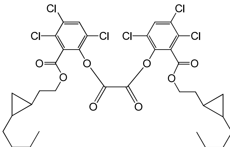
bis(3,4,6-trichloro-2-[[2-(2-butylcyclopropyl)ethoxy]carbonyl]phenyl) oxalate
