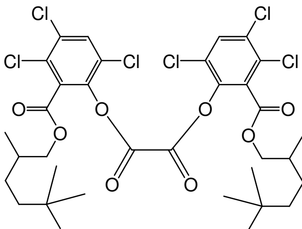
bis{3,4,6-trichloro-2-[(2,5,5-trimethylhexyloxy)carbonyl]phenyl} oxalate
