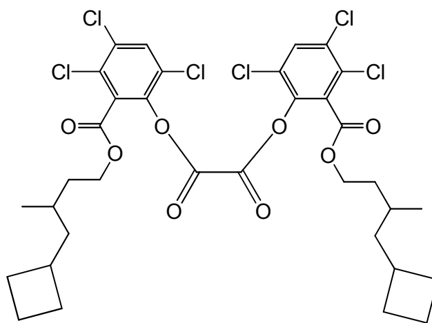
bis{3,4,6-trichloro-2-[(4-cyclobutyl-3-methylbutoxy)carbonyl]phenyl} oxalate
