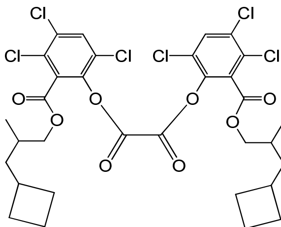
bis{3,4,6-trichloro-2-[(3-cyclobutyl-2-methylpropoxy)carbonyl]phenyl} oxalate
