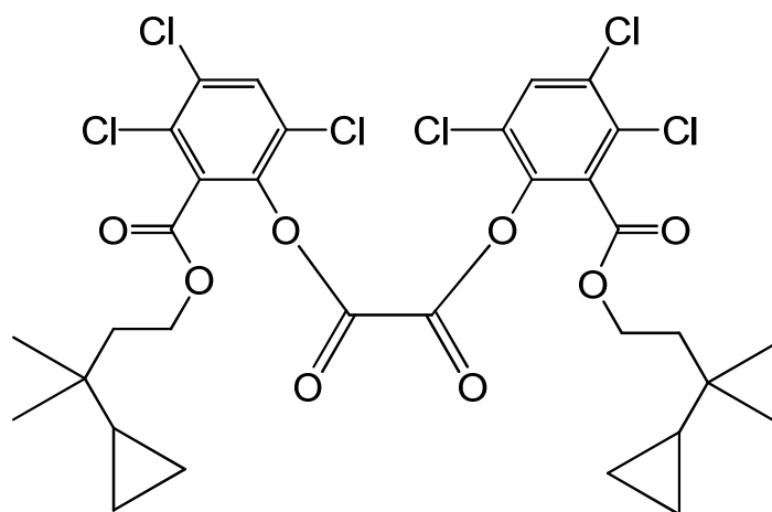
bis{3,4,6-trichloro-2-[(3-cyclopropyl-3-methylbutoxy)carbonyl]phenyl} oxalate
