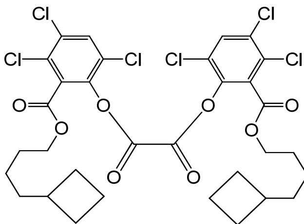
bis{3,4,6-trichloro-2-[(4-cyclobutylbutoxy)carbonyl]phenyl} oxalate
