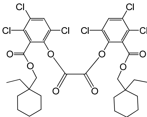
bis(3,4,6-trichloro-2-[[1-ethylcyclohexyl)methoxy]carbonyl}phenyl) oxalate
