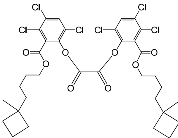
bis(3,4,6-trichloro-2-{[4-(1-methylcyclobutyl)butoxy]carbonyl}phenyl) oxalate
