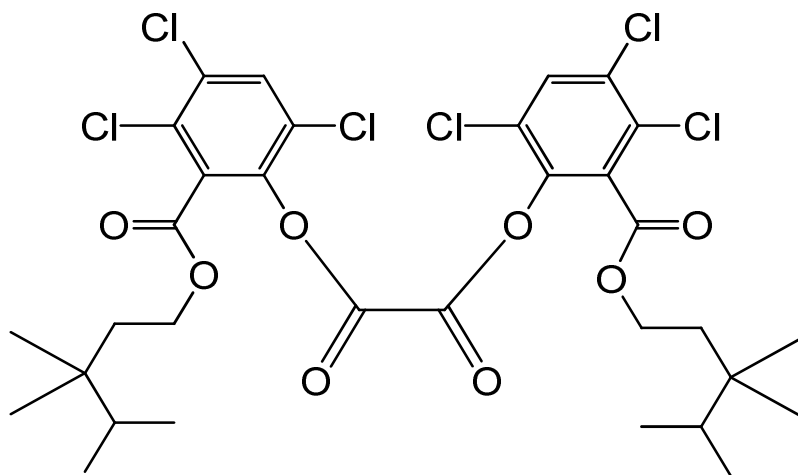
bis{3,4,6-trichloro-2-[(3,3,4-trimethylpentyloxy)carbonyl]phenyl} oxalate
