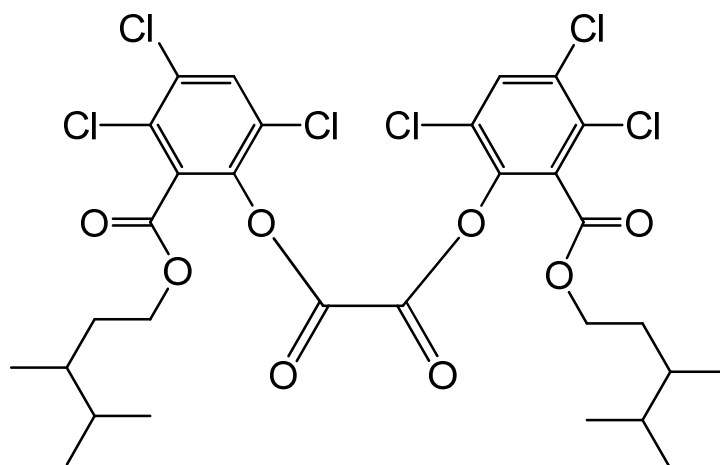
bis{3,4,6-trichloro-2-[(3,4-dimethylpentyloxy)carbonyl]phenyl} oxalate
