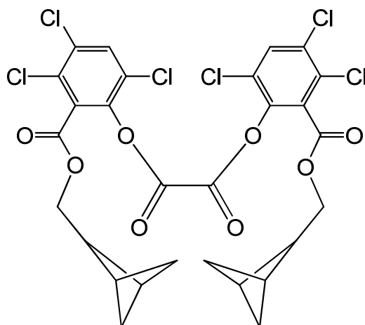
bis{2-[(bicyclo[1.1.1]pentan-5-ylmethoxy)carbonyl]-3,4,6-trichlorophenyl} oxalate
