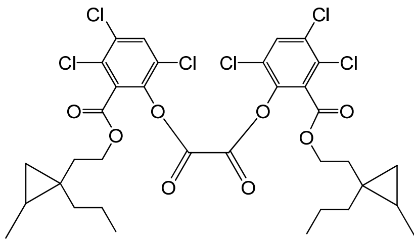
bis(3,4,6-trichloro-2-{[2-(3-methyl-1-propylcyclopropyl)ethoxy]carbonyl}phenyl) oxalate
