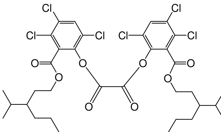
bis(3,4,6-trichloro-2-{[3-(1-methylethyl)hexyloxy]carbonyl}phenyl) oxalate
