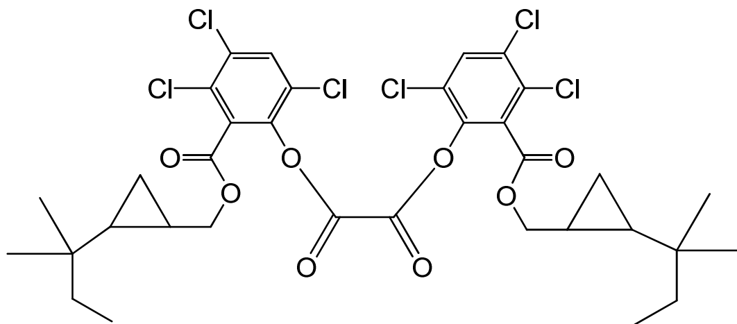
bis[3,4,6-trichloro-2-({[2-(1,1-dimethylpropyl)cyclopropyl]methoxy}carbonyl)phenyl] oxalate
