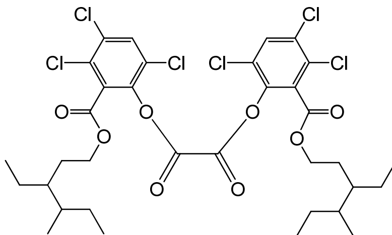
bis{3,4,6-trichloro-2-[(3-ethyl-4-methylhexyloxy)carbonyl]phenyl} oxalate
