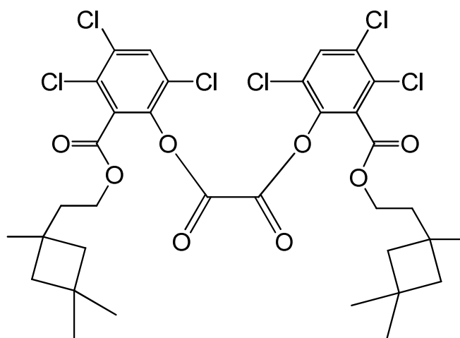
bis(3,4,6-trichloro-2-{[2-(1,3,3-trimethylcyclobutyl)ethoxy]carbonyl}phenyl) oxalate
