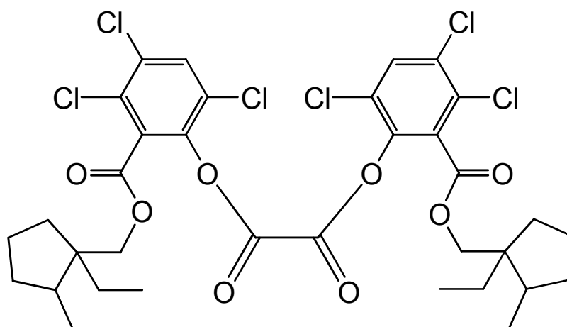
bis(3,4,6-trichloro-2-[(1-ethyl-2-methylcyclopentyl)methoxy]carbonyl)phenyl) oxalate
