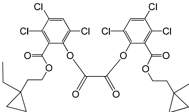
bis(3,4,6-trichloro-2-{[2-(1-ethylcyclopropyl)ethoxy]carbonyl}phenyl) oxalate
