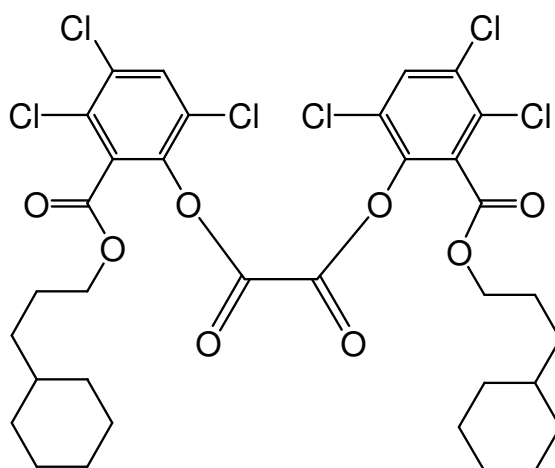
bis{3,4,6-trichloro-2-[(3-cyclohexylpropoxy)carbonyl]phenyl} oxalate
