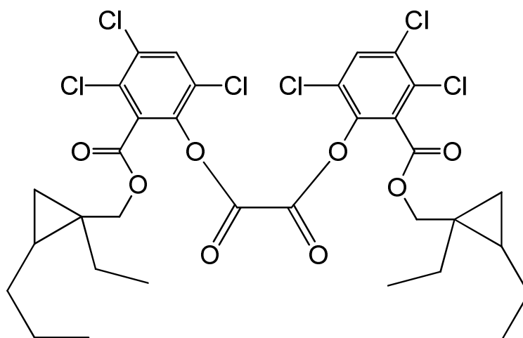
bis(3,4,6-trichloro-2-[(1-ethyl-2-propylcyclopropyl)methoxy]carbonyl)phenyl oxalate
