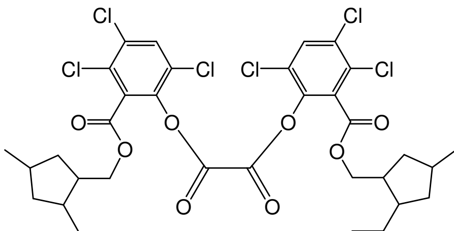
bis(3,4,6-trichloro-2-[(2-ethyl-4-methylcyclopentyl)methoxy]carbonyl)phenyl) oxalate
