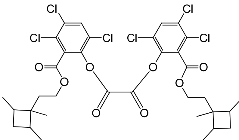
bis(3,4,6-trichloro-2-{[2-(1,2,4-trimethylcyclobutylethoxy)]carbonyl}phenyl) oxalate
