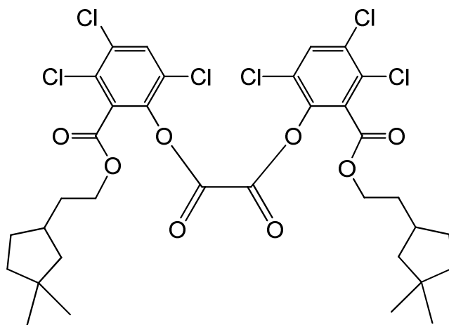
bis(3,4,6-trichloro-2-[[2-(3,3-dimethylcyclopentyl)ethoxy]carbonyl]phenyl) oxalate
