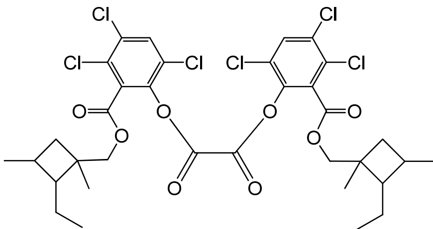
bis(3,4,6-trichloro-2-{[(2-ethyl-1,3-dimethylcyclobutyl)methoxy]carbonyl}phenyl) oxalate
