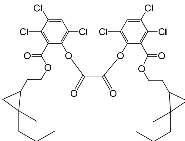
bis(3,4,6-trichloro-2-{[2-(2-methyl-2-propylcyclopropyl)ethoxy]carbonyl}phenyl) oxalate
