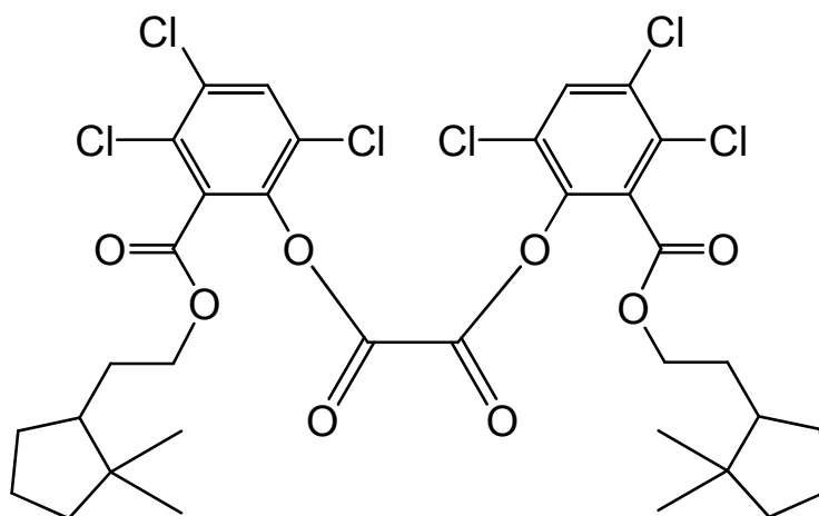
bis(3,4,6-trichloro-2-[[2-(2,2-dimethylcyclopentyl)ethoxy]carbonyl]phenyl) oxalate
