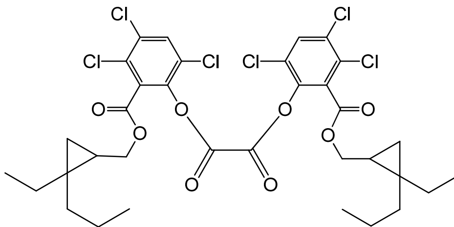
bis(3,4,6-trichloro-2-[(2-ethyl-2-propylcyclopropyl)methoxy]carbonyl)phenyl) oxalate
