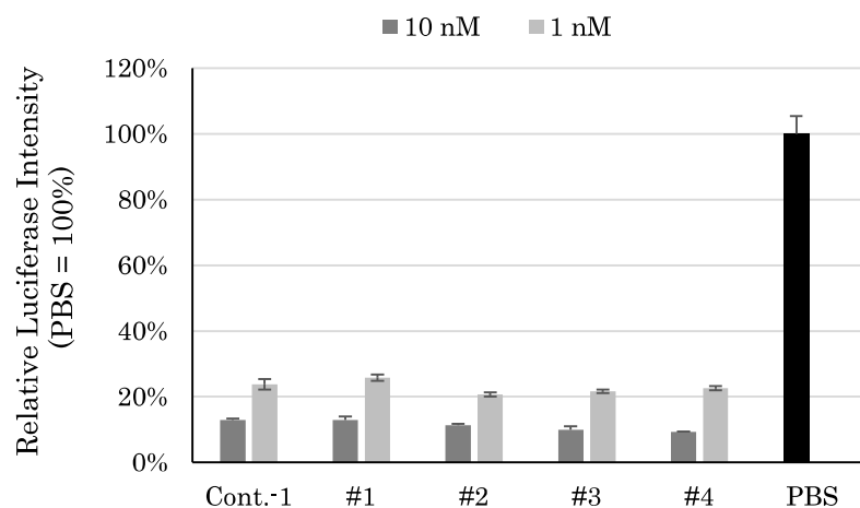
Fig. 1 Dual luciferase reporter assay using modified Luciferase siRNAs in HEK 293 cells
