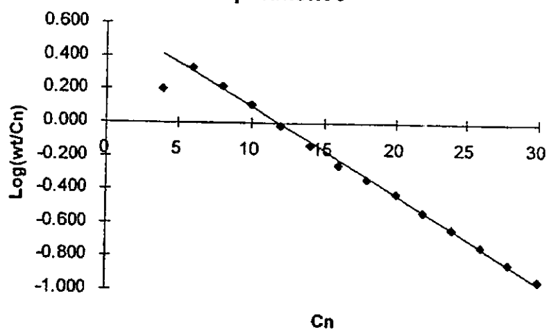
Figure 6: Regression Analysis of Experiment 6
