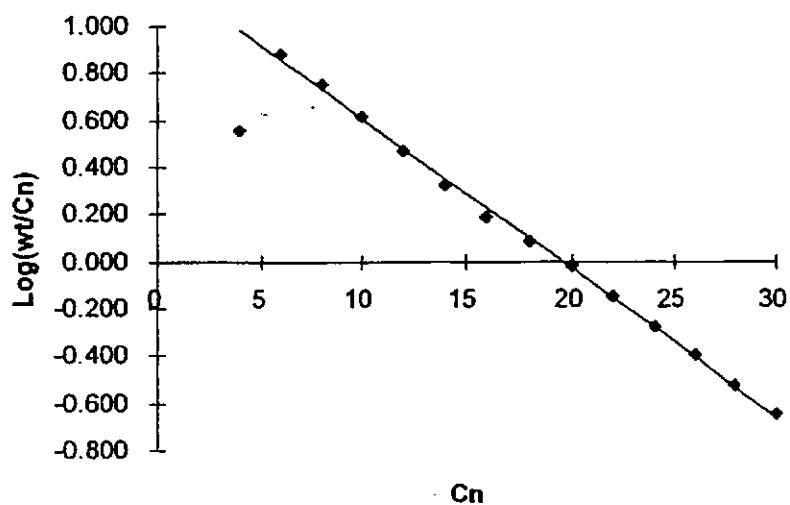
Figure 3: Regression Analysis of Experiment 1
