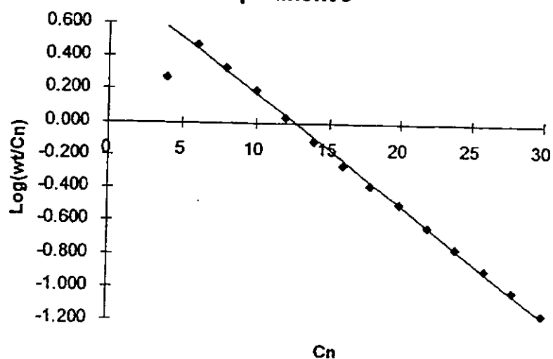
Figure 5: Regression Analysis of Experiment 5
