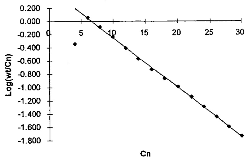
Figure 4: Regression Analysis of Experiment 4
