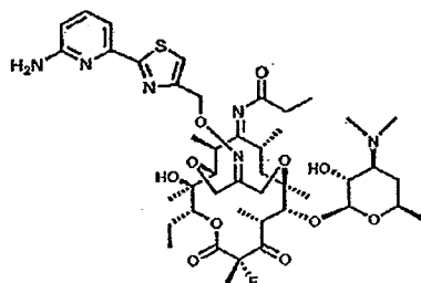
Compound 3
