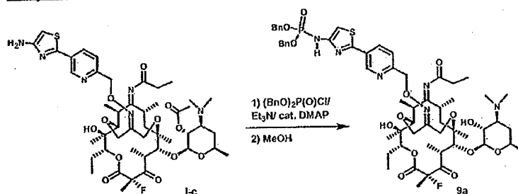
Compound 9
