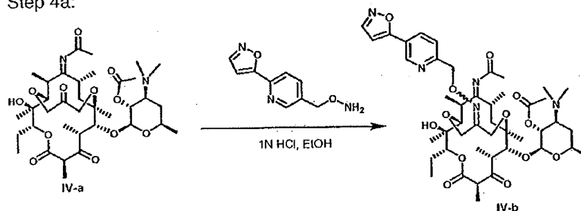
Compound 4
