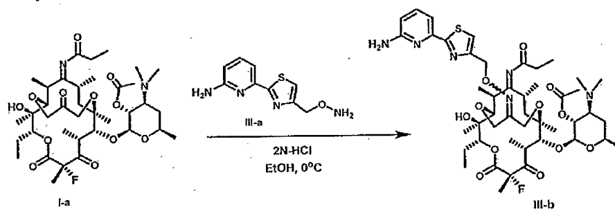
Compound 3
