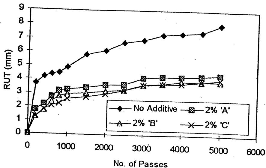
Fig. 3A Comparison of Wheel Tracking Test Results for Mix with Cariphalte and 2% Additive
