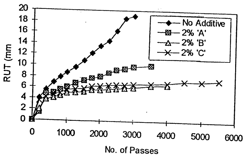
Fig. 3B Comparison of Wheel Tracking Test Results for Mix with 60/70 and 2% Additive
