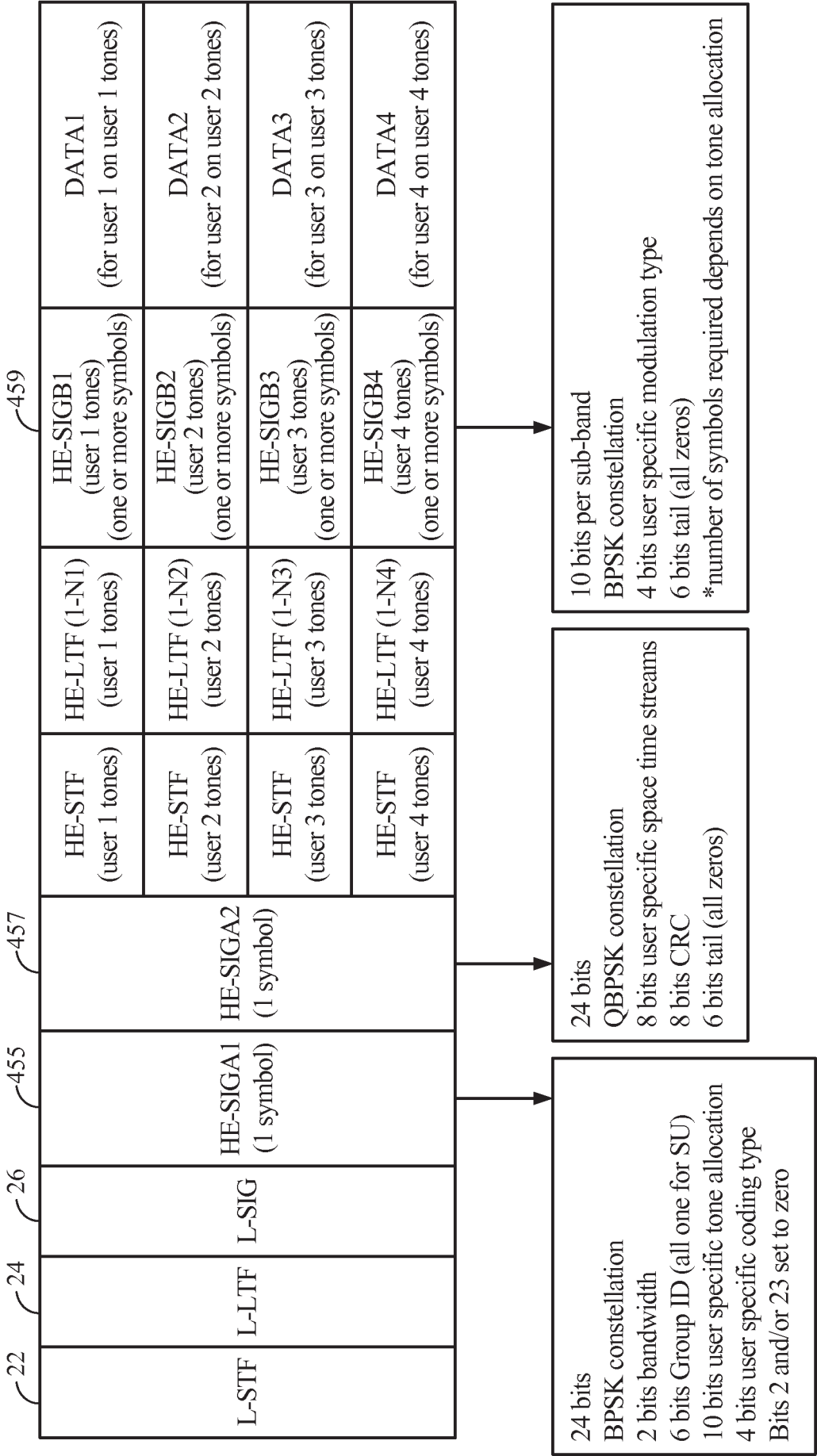
HE downlink packet implementation 4:
