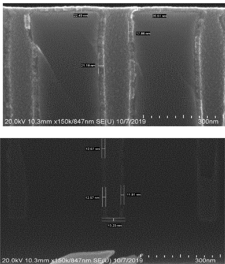
ZOOM of VIA TOP &amp; BOTTOM
