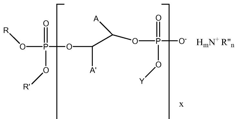
Formula (1a)
