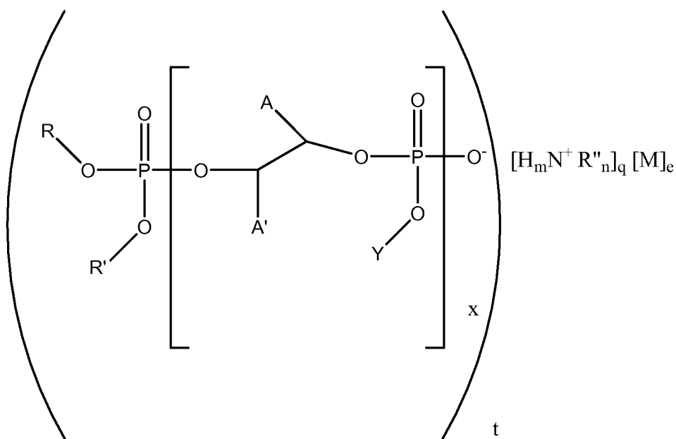
Formula (1)
