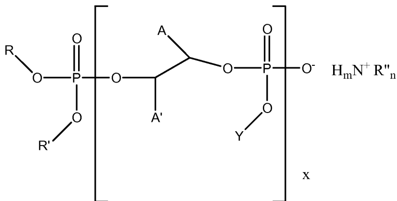
Formula (1a)
