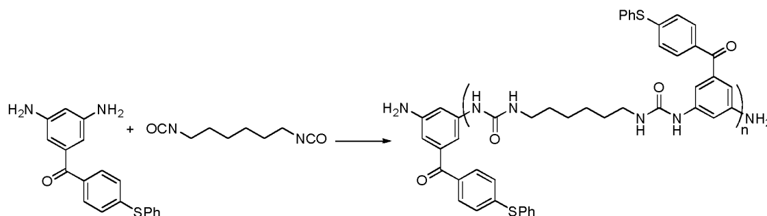
Scheme 3: Synthesis of polymeric polyurethane-based photoinitiators as described in J. Wei, 20 H. Wang, X. Jiang, J. Yin, Macromolecules , 40 (2007), 2344-2351).
