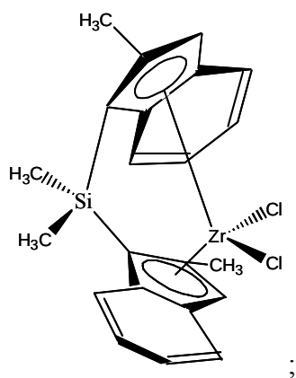
1,2-ethanediylbis(9-fluorenyl)zirconium dichloride,
