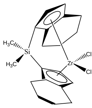
dimethylsilylbis(2-methyl-1-indenyl)zirconium dichloride,
