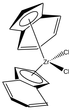
methyl(octyl)silylbis(9-fluorenyl)zirconium dichloride,
