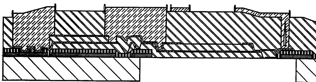
Side view including sacrificial layers
