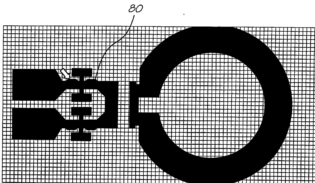
Top view of actuator layer (mask 4)
