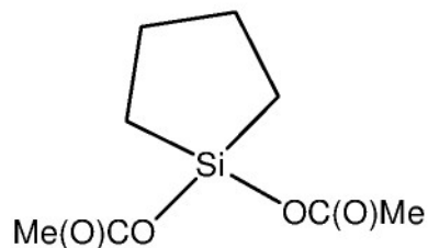
1,1-diacetoxy-1-silacyclopentane
