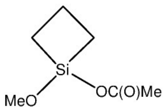
1-methoxy-1-acetoxy-1-silacyclobutane
