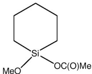
1-methoxy-1-acetoxy-1-silacyclohexane
