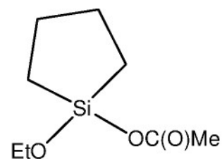
1-ethoxy-1-acetoxy-1-silacyclopentane
