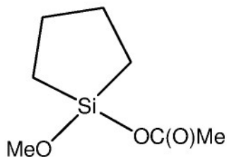
1-methoxy-1-acetoxy-1-silacyclopentane
