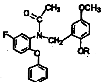
DAA1106 (2) : \text{R}=\text{CH}_3 [^{11}\text{C}] DAA1106 ( [^{11}\text{C}] 2) : \text{R}=\text{}^{11}\text{CH}_3
