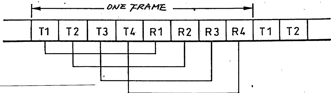
FIG. 2B TDMA SYSTEM
