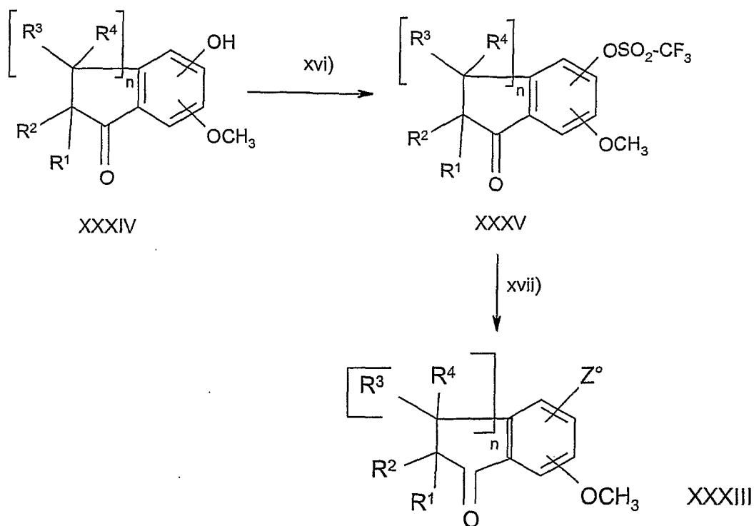
Reaction scheme 6
