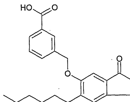
example 44
