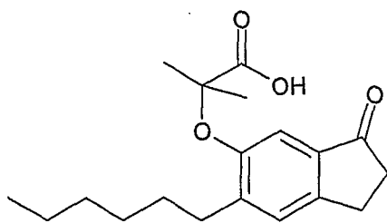
example 8
