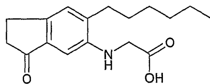
example 38
