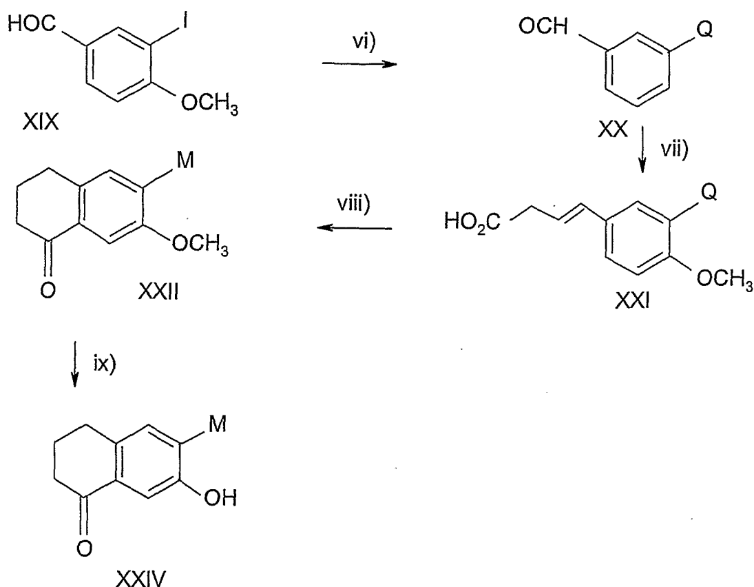
Reaction scheme 3
