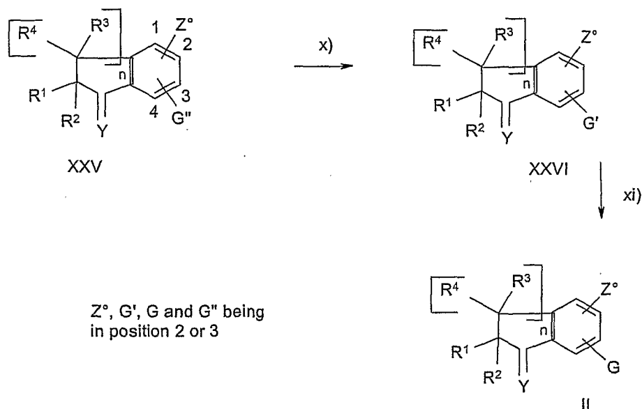
Reaction scheme 4
