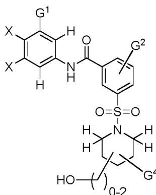
(IVc)
