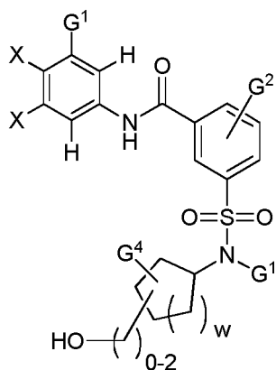
(VIb)
