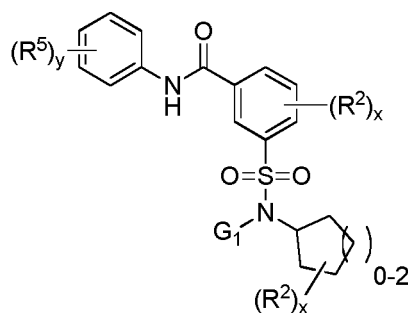
(IIc)
