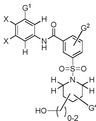
(IVc)
