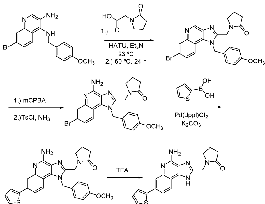
Scheme 8
