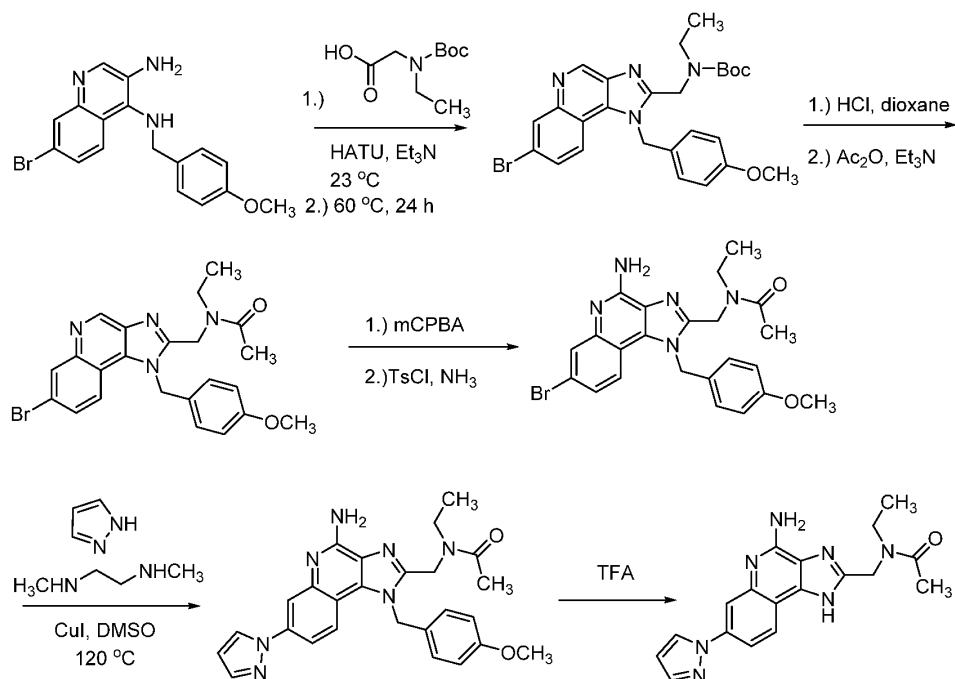
Scheme 3
