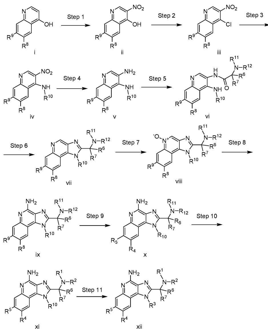
Scheme 1
