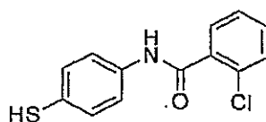
2-chloro-N-(4-mercaptophenyl)benzamide
