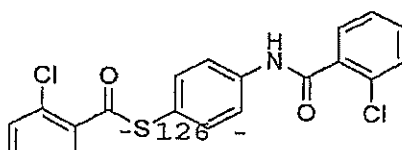
2-chloro-N-(4-mercaptophenyl)benzamide
