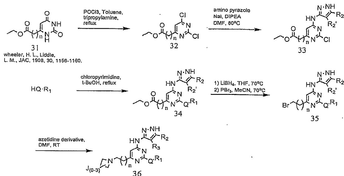
Scheme IX
