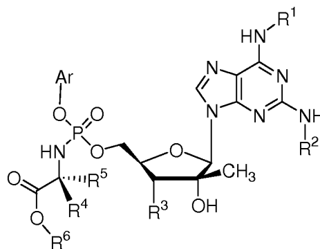
(XLV)
