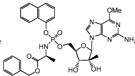
Compound I
