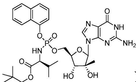
Compound B
