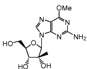
Compound E
