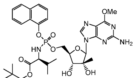
Compound C
