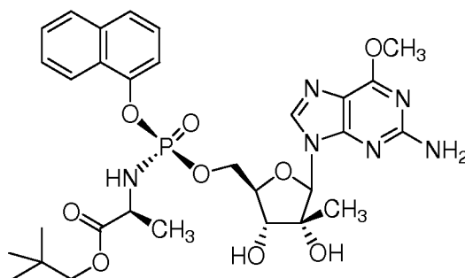
(S)-P
