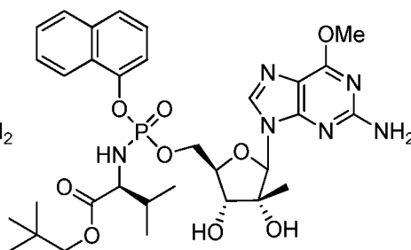
Compound C
