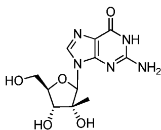
Compound D
