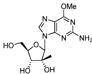
Compound E
