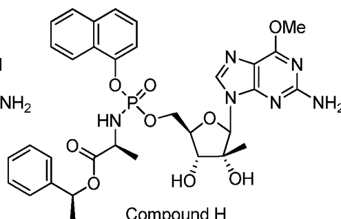
Compound H
