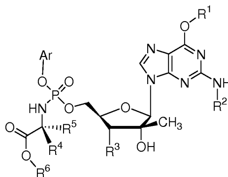
(XLVIII)
