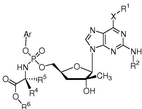
(XLVII)
