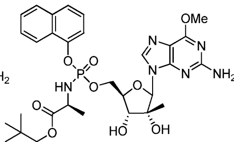
Compound F
