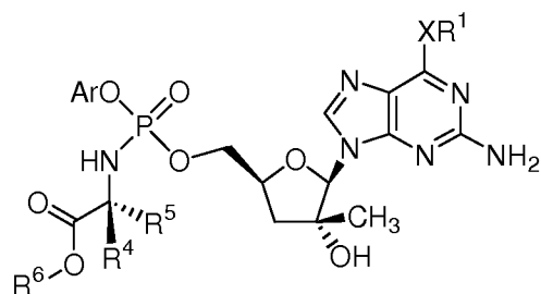
(lb)
