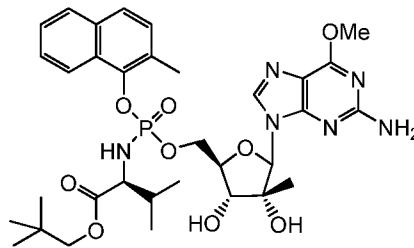
Compound L
