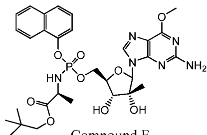
Compound F
