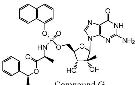
Compound G
