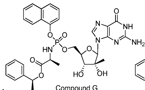
Compound G
