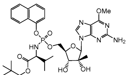
Compound C
