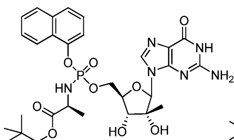
Compound A
