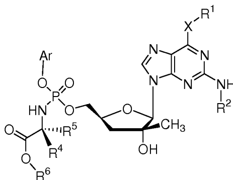
(XLVII)
