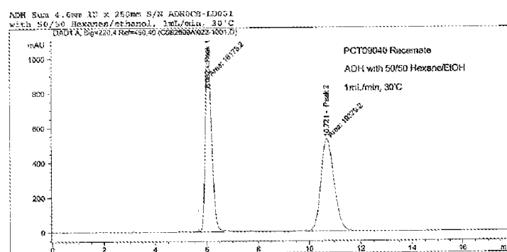
Figure 1. Separation of Diastereomers by Chiral Chromatography.
