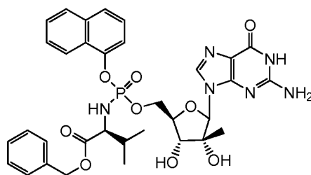
Compound M
