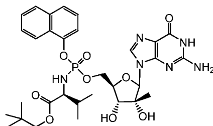
Compound B
