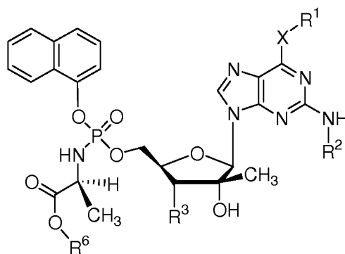
(XL)
