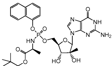
Compound A
