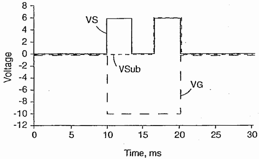
Fig. 5 Prior Art
