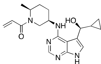
1-((2 S ,5 R )-5-((5-(( S )-cyclopropyl(hydroxy)methyl)-7 H -pyrrolo[2,3- d ]pyrimidin-4-yl)amino)-2-methylpiperidin-1-yl)prop-2-en-1-one
