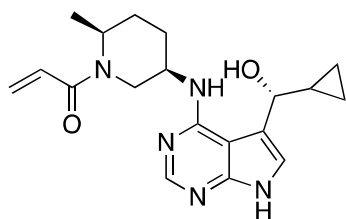
1-((2 S ,5 R )-5-((5-(( R )-cyclopropyl(hydroxy)methyl)-7 H -pyrrolo[2,3- d ]pyrimidin-4-yl)amino)-2-methylpiperidin-1-yl)prop-2-en-1-one
