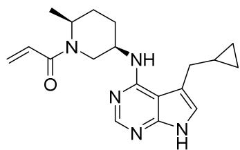
1-((2 S ,5 R )-5-((5-(cyclopropylmethyl)-7 H -pyrrolo[2,3- d ]pyrimidin-4-yl)amino)-2-methylpiperidin-1-yl)prop-2-en-1-one ,
