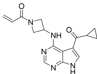
1-(3-((5-(cyclopropanecarbonyl)-7 H -pyrrolo[2,3- d ]pyrimidin-4-yl)amino)azetidin-1-yl)prop-2-en-1-one ,
