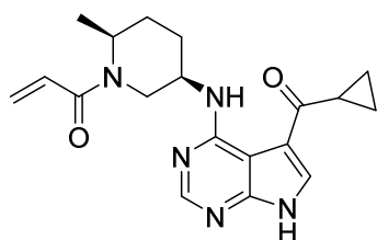
1-((2 S ,5 R )-5-((5-(cyclopropanecarbonyl)-7 H -pyrrolo[2,3- d ]pyrimidin-4-yl)amino)-2-methylpiperidin-1-yl)prop-2-en-1-one
