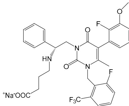
Elagolix
