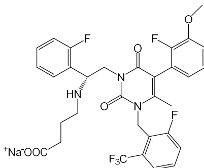
Formula II
