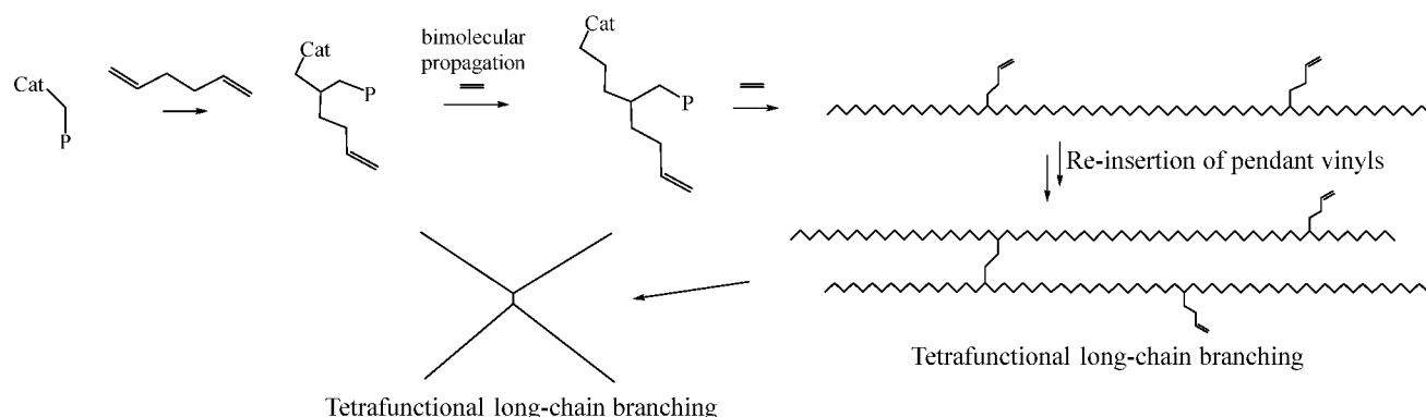
Scheme 2: Long-Chain Branching via Diene Incorporation
