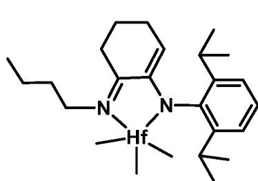
Catalyst 1: Dual-chain catalyst
