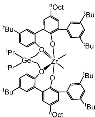
Catalyst 4 Single-Chain Catalyst
