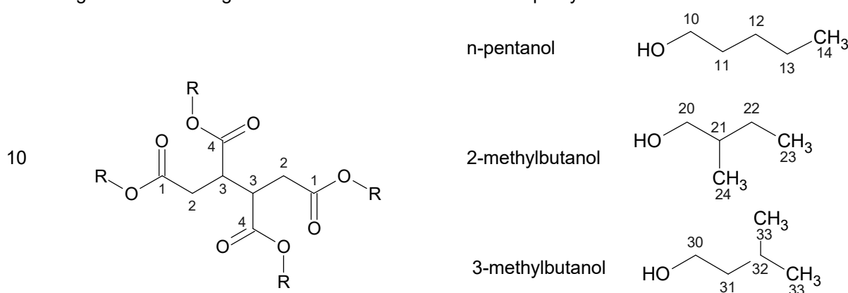
Figure 1: Numbering of the carbon atoms in the different pentyl radicals
