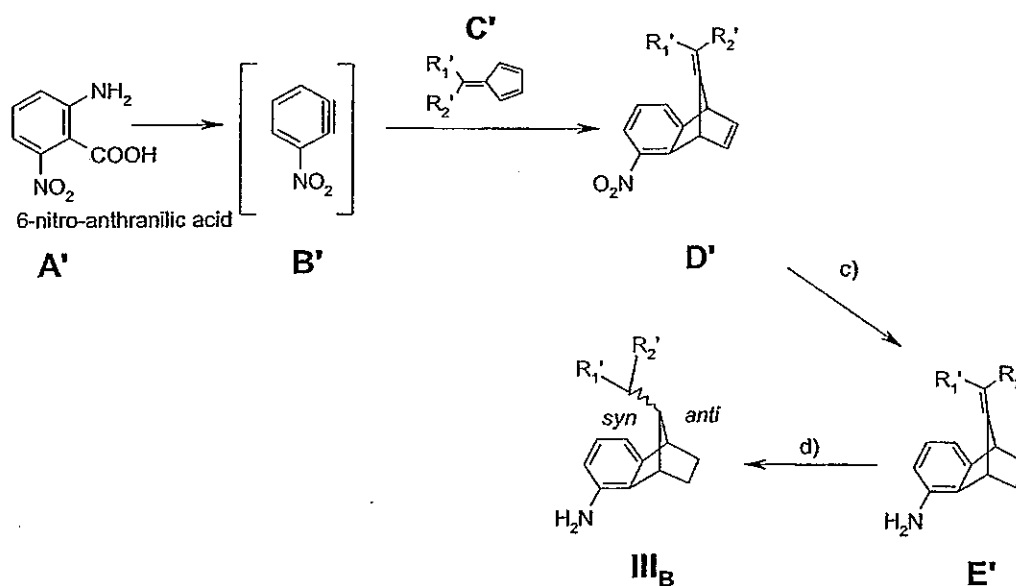
Scheme 1: Synthesis of III B using 6-nitroanthranilic acid
