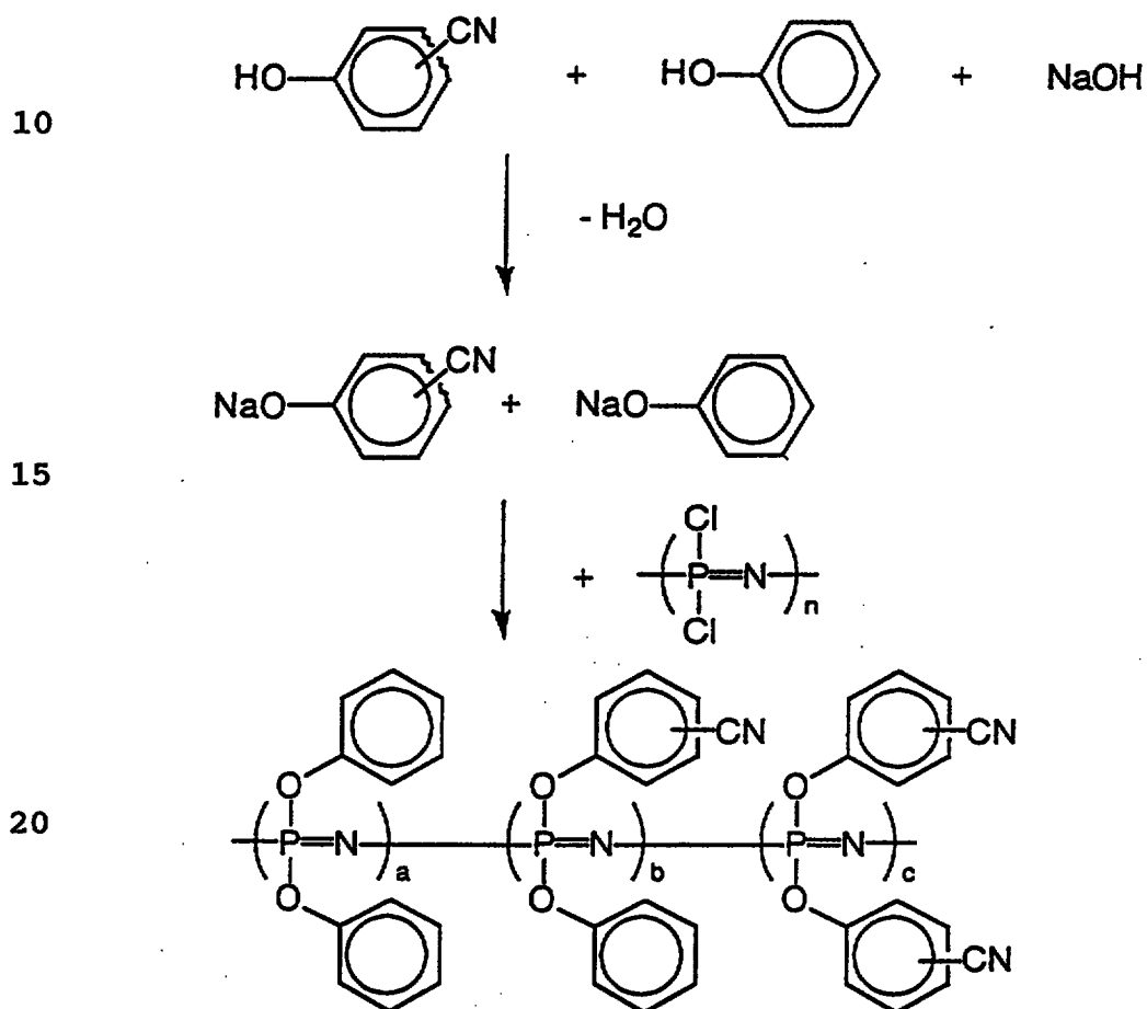
Reaction Scheme-3
