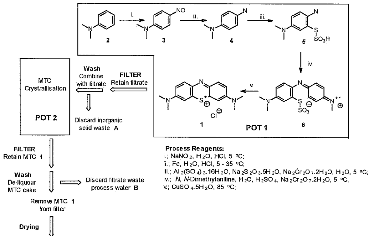
Scheme 2b: Two reactor MTC process
