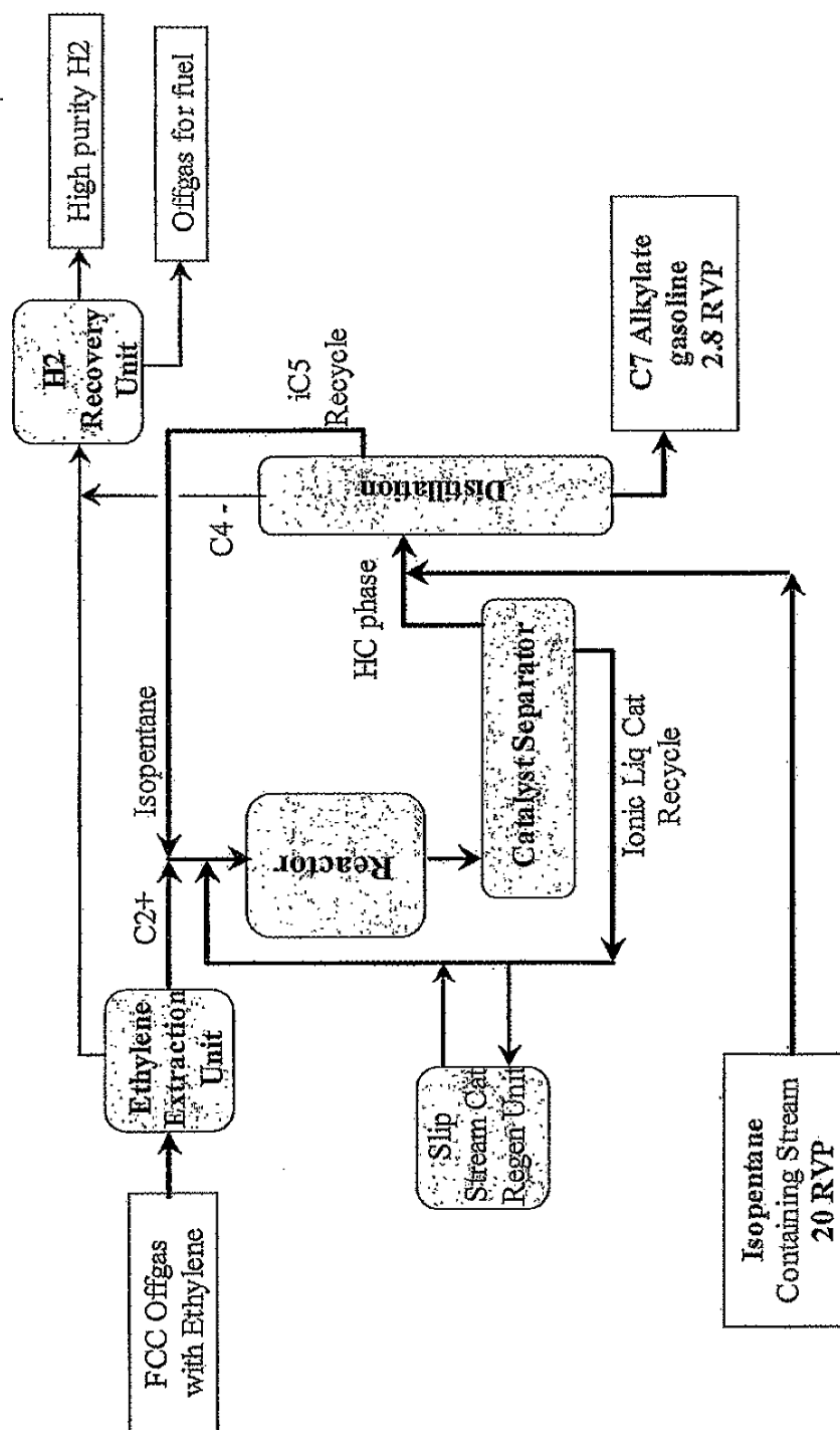
Figure 1 Isopentane and Ethylene Alkylation Process Scheme
