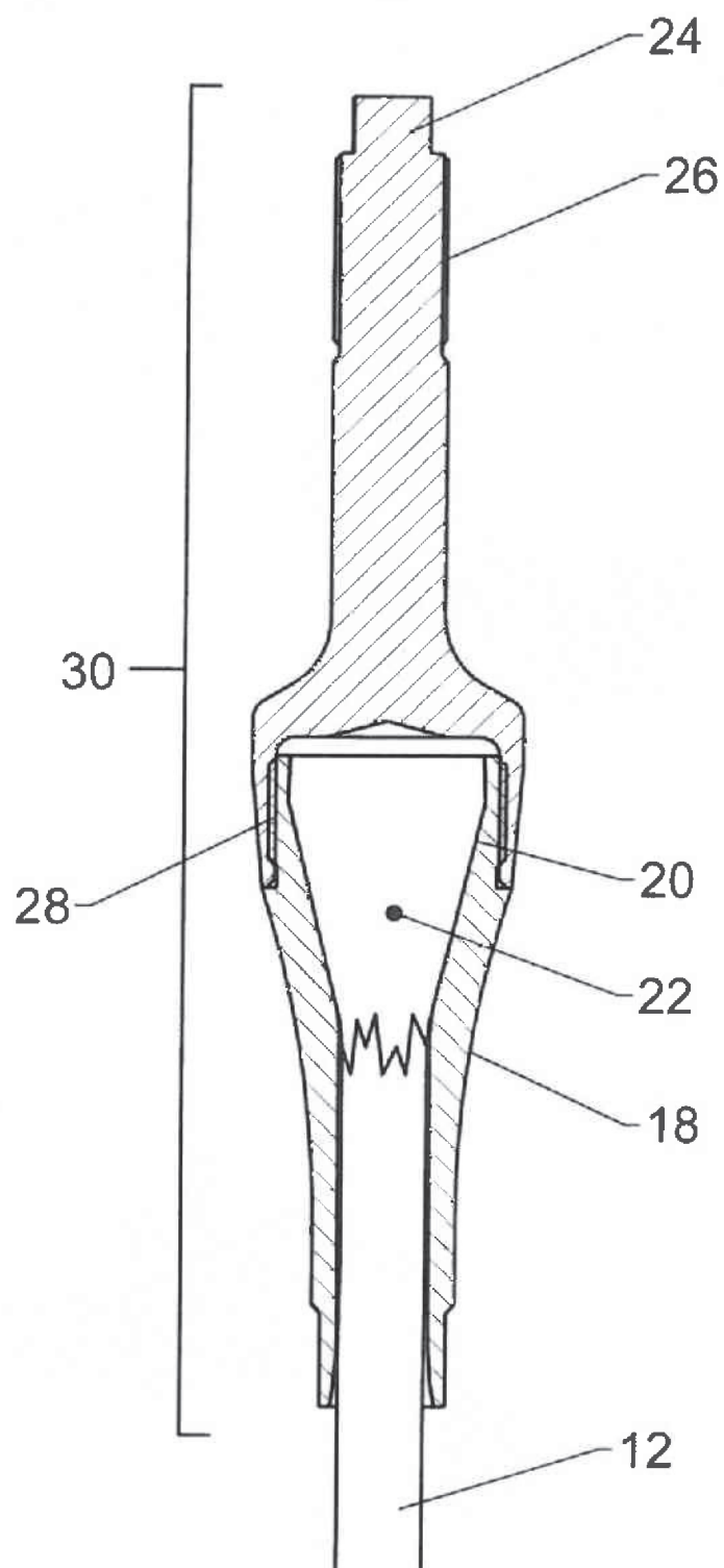
FIG. 2 (PRIOR ART)
