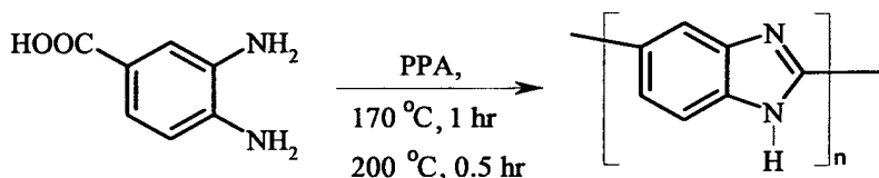
3,4-Diaminobenzoic acid
