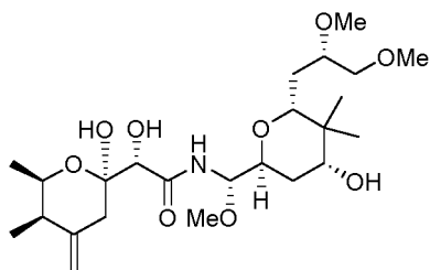
Pseudopederin
