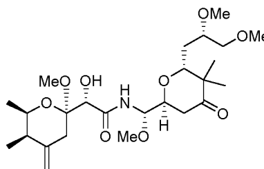
Pederone
