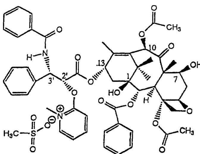
Paclitaxel-2'-methylpyridinium mesylate
