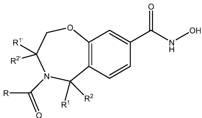
(IA-1c).
