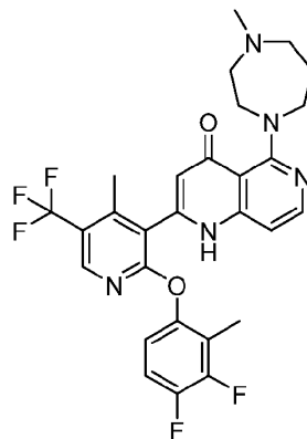
2-[2-(3,4-difluoro-2-methyl-phenoxy)-4-methyl-5-(trifluoromethyl)-3-pyridyl]-5-(4-methyl-1,4-diazepan-1-yl)-1H-1,6-naphthyridin-4-one
