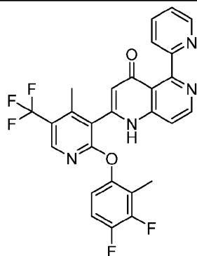
2-[2-(3,4-difluoro-2-methyl-phenoxy)-4-methyl-5-(trifluoromethyl)-3-pyridyl]-5-(2-pyridyl)-1H-1,6-naphthyridin-4-one
