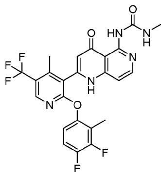
1-[2-[2-(3,4-difluoro-2-methyl-phenoxy)-4-methyl-5-(trifluoromethyl)-3-pyridyl]-4-oxo-1H-1,6-naphthyridin-5-yl]-3-methyl-urea
