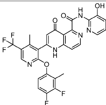
2-[2-(3,4-difluoro-2-methyl-phenoxy)-4-methyl-5-(trifluoromethyl)-3-pyridyl]-N-(3-hydroxy-2-pyridyl)-4-oxo-1H-1,6-naphthyridine-5-carboxamide
