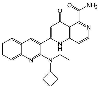
2-[2-[cyclobutyl(ethyl)amino]-3-quinolyl]-4-oxo- 1H-1,6-naphthyridine-5-carboxamide
