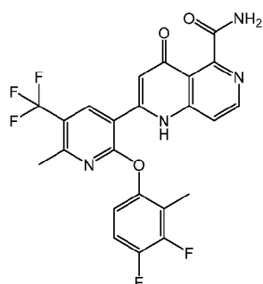
2-[2-(3,4-difluoro-2-methyl-phenoxy)-6-methyl-5-(trifluoromethyl)-3-pyridyl]-4-oxo-1H-1,6-naphthyridine-5-carboxamide
