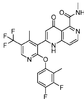
2-[2-(3,4-difluoro-2-methyl-phenoxy)-4-methyl-5-(trifluoromethyl)-3-pyridyl]-N-methyl-4-oxo-1H-1,6-naphthyridine-5-carboxamide
