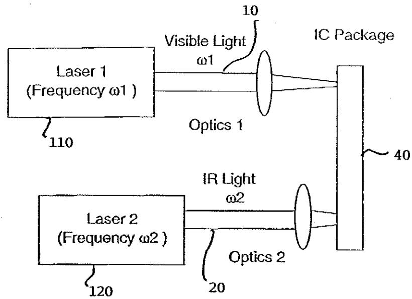
Laser source scheme with two different lasers for different wavelength dual beams
