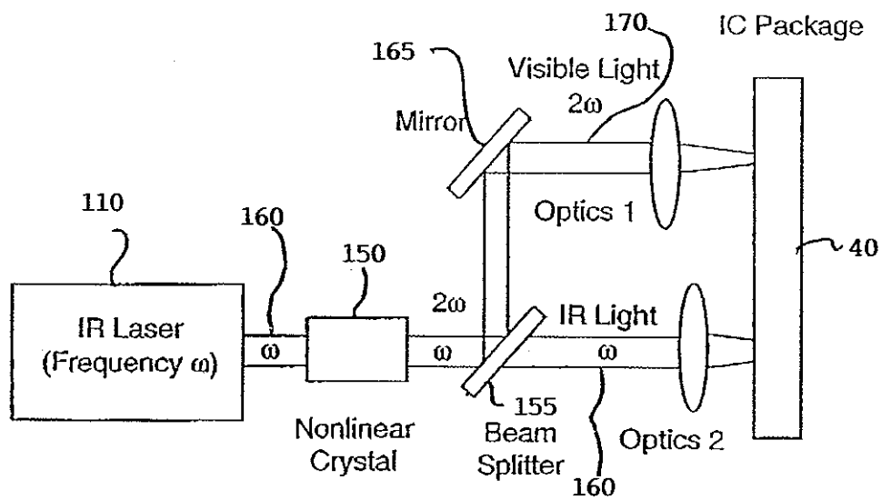
Laser source scheme with one laser for different wavelength dual beams
