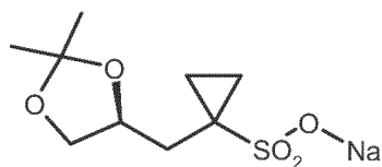
(S)-7
