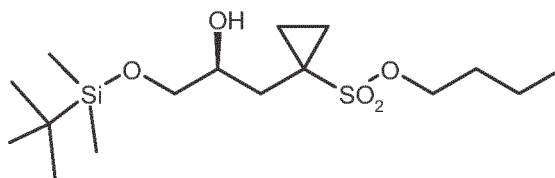
(S)-9a .
