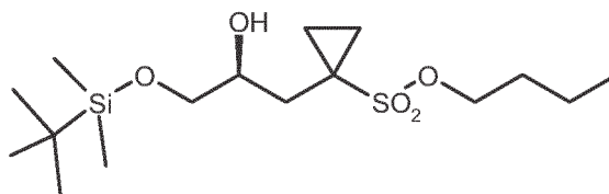
(S)-9a ;
