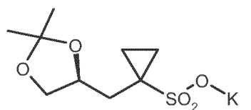
(S)-7' ;
