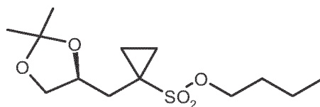
(S)-6 ;
