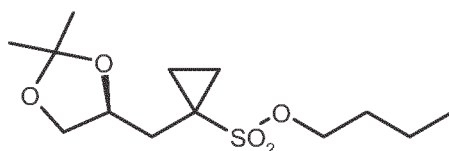
(S)-6
