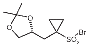
(R)-10-Br
