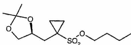
(S)-6
