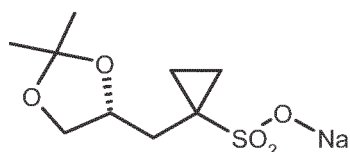
(R)-7
