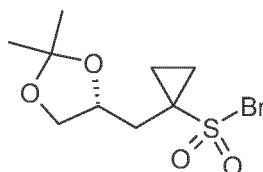
(R)-10-Br
