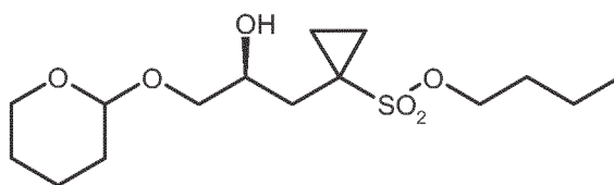
(S)-9b.
