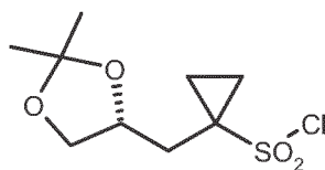
(R)-10
