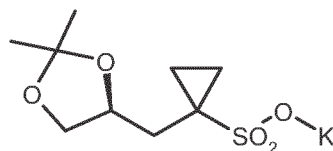
(S)-7'
