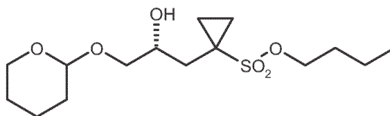
(R)-9b ;
