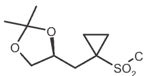
(S)-10
