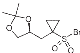
(S)-10-Br
