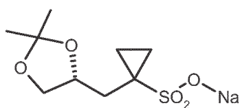
(R)-7
