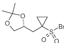
(R)-10-Br
