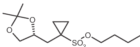
(R)-6
