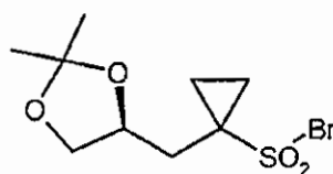
(S)-10-Br
