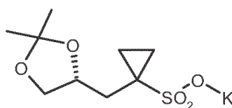
(R)-7'
