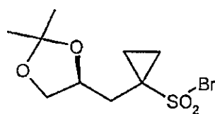
(S)-10-Br
