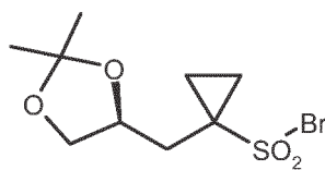
(S)-10-Br
