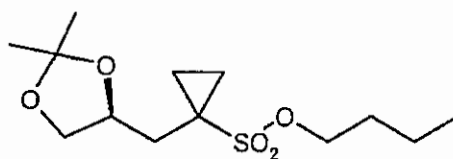
(S)-6
