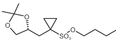
(R)-6
