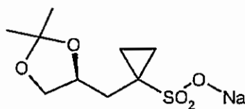
(S)-7
