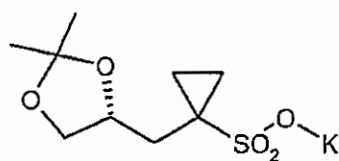
(R)-7' ;
