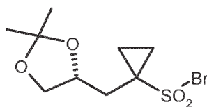
(R)-10-Br
