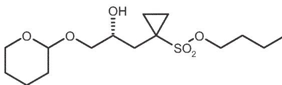
(R)-9b.
