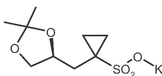
(S)-7'
