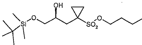
(S)-9a ;
