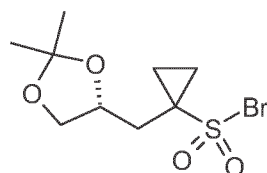
(R)-10-Br
