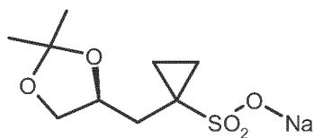
(S)-7
