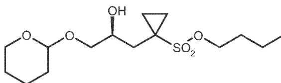
(S)-9b ;
