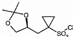
(S)-10
