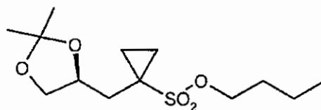
(S)-6 ;
