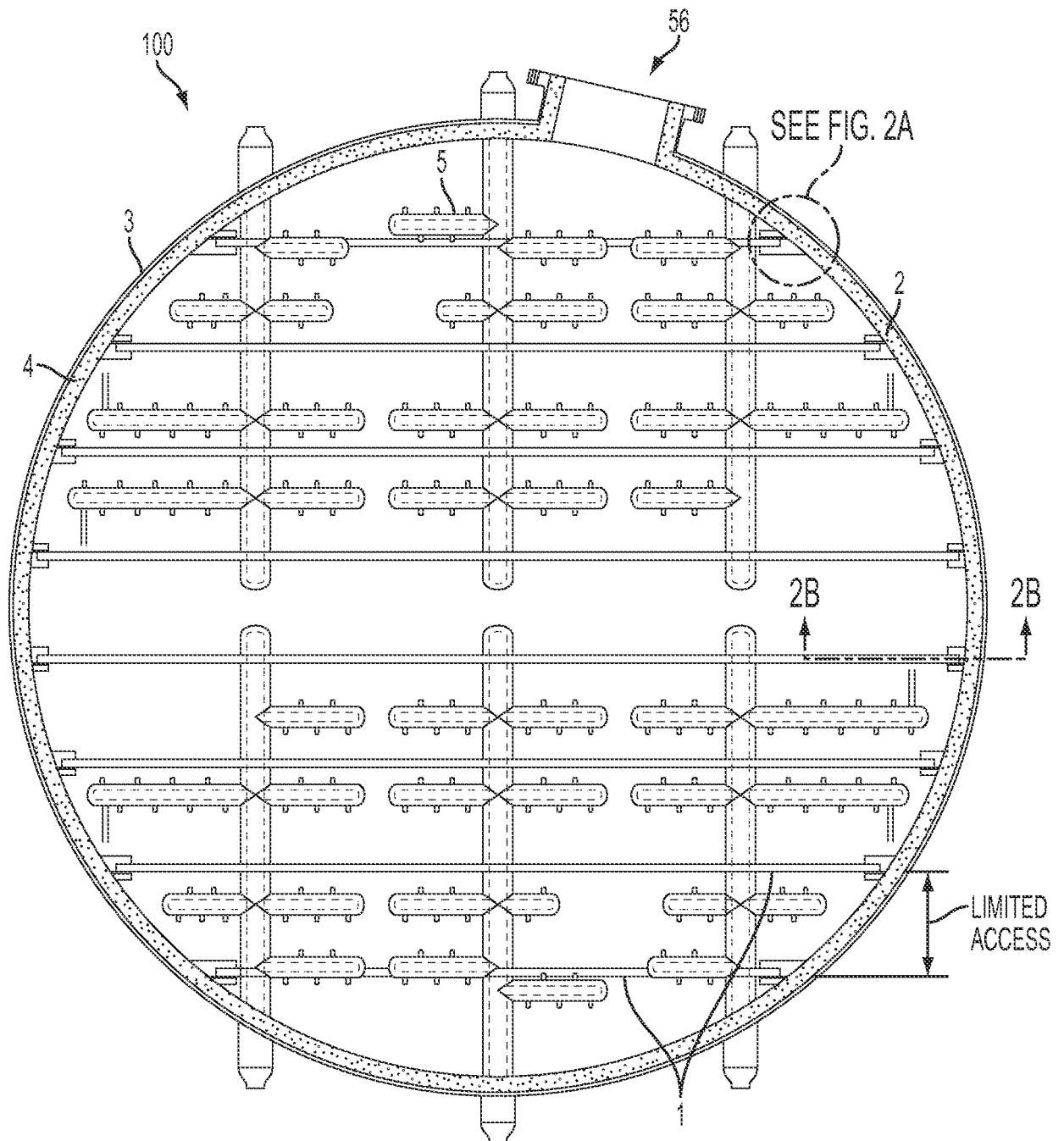
FIG. 1 PRIOR ART
