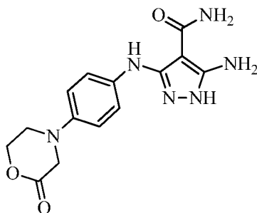
5-amino-3-((4-(2-oxomorpholino)phenyl)amino)-1H-pyrazole-4-carboxamide
