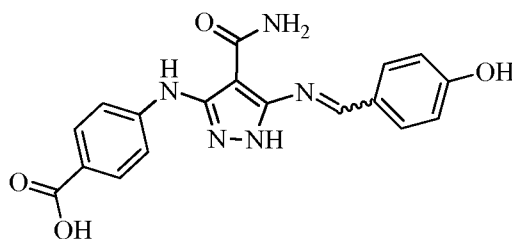
4-((4-carbamoyl-5-((4-hydroxybenzylidene)amino)-1 H -pyrazol-3-yl)amino)benzoic acid
