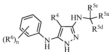
(XV-c)
