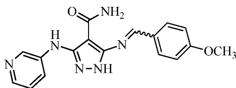
5-((4-methoxybenzylidene)amino)-3-(pyridin-3-ylamino)-1 H -pyrazole-4-carboxamide
