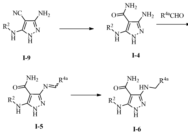
Scheme III
