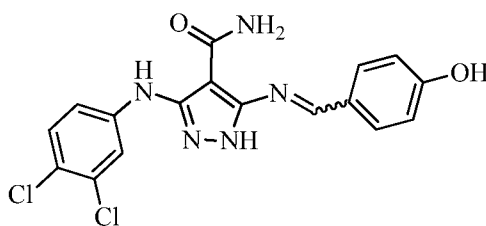
3-((3,4-dichlorophenyl)amino)-5-((4-hydroxybenzylidene)amino)-1 H -pyrazole-4-carboxamide
