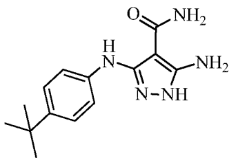
5-amino-3-((4-( tert -butyl)phenyl)amino)-1 H -pyrazole-4-carboxamide
