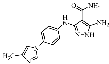
5-amino-3-((4-(4-methyl-1H-imidazol-1-yl)phenyl)amino)-1H-pyrazole-4-carboxamide
