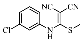
2-(((3-chlorophenyl)amino)(methylthio)methylene)malononitrile
