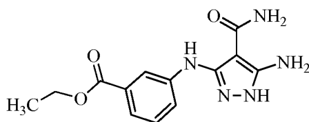
ethyl 3-((5-amino-4-carbamoyl-1H-pyrazol-3-yl)amino)benzoate
