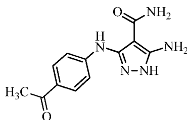
3-((4-acetylphenyl)amino)-5-amino-1 H -pyrazole-4-carboxamide
