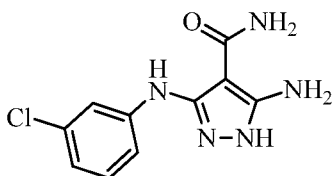
5-amino-3-((3-chlorophenyl)amino)-1H-pyrazole-4-carboxamide
