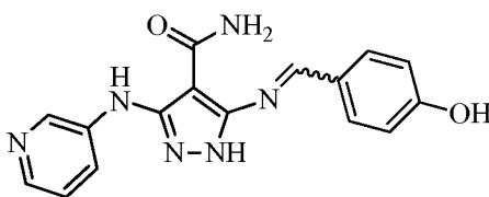
5-((4-hydroxybenzylidene)amino)-3-(pyridin-3-ylamino)-1 H -pyrazole-4-carboxamide
