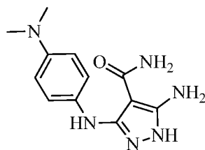
5-amino-3-((4-(dimethylamino)phenyl)amino)-1 H -pyrazole-4-carboxamide
