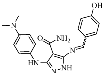
3-((4-(dimethylamino)phenyl)amino)-5-((4-hydroxybenzylidene)amino)-1 H -pyrazole-4-carboxamide
