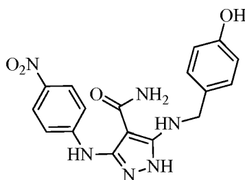
5-((4-hydroxybenzyl)amino)-3-((4-nitrophenyl)amino)-1 H -pyrazole-4-carboxamide
