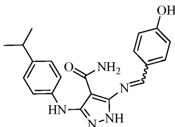
5-((4-hydroxybenzylidene)amino)-3-((4-isopropylphenyl)amino)-1 H -pyrazole-4-carboxamide
