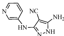
5-amino-3-(pyridin-3-ylamino)-1 H -pyrazole-4-carbonitrile
