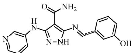
5-((3-hydroxybenzylidene)amino)-3-(pyridin-3-ylamino)-1 H -pyrazole-4-carboxamide
