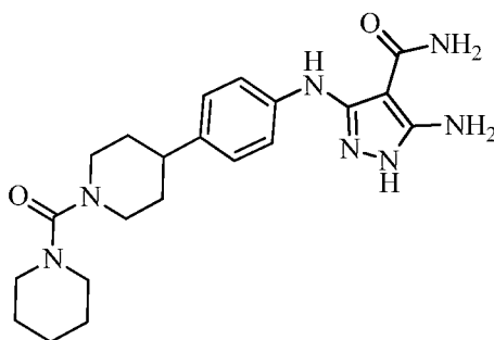
5-amino-3-((4-(1-(piperidine-1-carbonyl)piperidin-4-yl)phenyl)amino)-1 H -pyrazole-4-carboxamide
