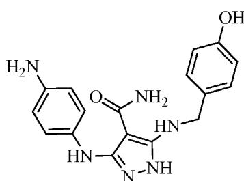
3-((4-aminophenyl)amino)-5-((4-hydroxybenzyl)amino)-1 H -pyrazole-4-carboxamide
