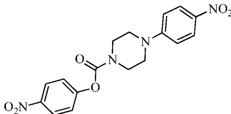
4-nitrophenyl 4-(4-nitrophenyl)piperazine-1-carboxylate
