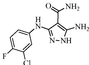
5-amino-3-((3-chloro-4-fluorophenyl)amino)-1H-pyrazole-4-carboxamide
