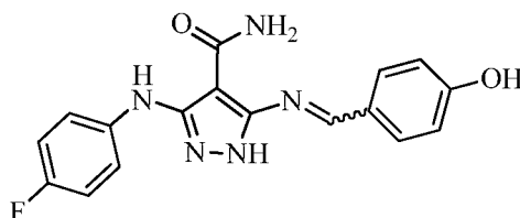
3-((4-fluorophenyl)amino)-5-((4-hydroxybenzylidene)amino)-1 H -pyrazole-4-carboxamide
