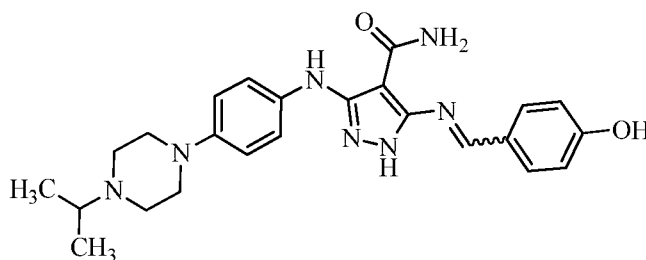
5-((4-(4-isopropylpiperazin-1-yl)phenyl)amino)-3-((4-hydroxybenzyl)amino)-1 H -pyrazole-4-carboxamide
