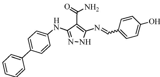
3-([1,1'-biphenyl]-4-ylamino)-5-((4-hydroxybenzylidene)amino)-1 H -pyrazole-4-carboxamide
