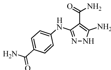
5-amino-3-((4-carbamoylphenyl)amino)-1 H -pyrazole-4-carboxamide
