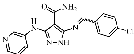
5-((4-chlorobenzylidene)amino)-3-(pyridin-3-ylamino)-1 H -pyrazole-4-carboxamide
