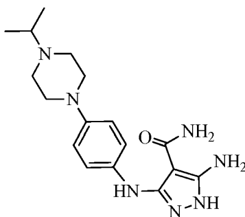
5-amino-3-((4-(4-isopropylpiperazin-1-yl)phenyl)amino)-1 H -pyrazole-4-carboxamide
