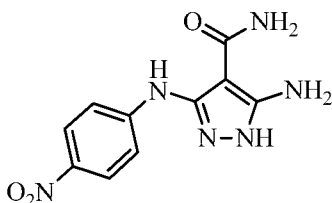
5-amino-3-((4-nitrophenyl)amino)-1H-pyrazole-4-carboxamide
