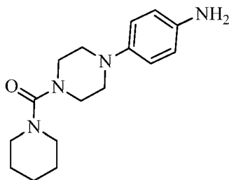
(4-(4-aminophenyl)piperazin-1-yl)(piperidin-1-yl)methanone
