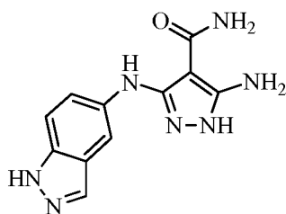
3-((1H-indazol-5-yl)amino)-5-amino-1H-pyrazole-4-carboxamide
