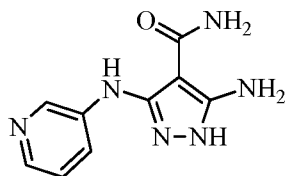
5-amino-3-(pyridin-3-ylamino)-1 H -pyrazole-4-carboxamide
