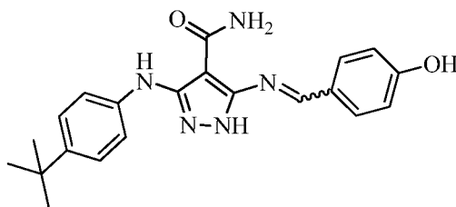
3-((4-( tert -butyl)phenyl)amino)-5-((4-hydroxybenzylidene)amino)-1 H -pyrazole-4-carboxamide
