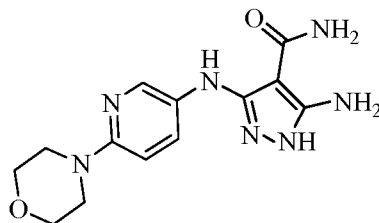
5-amino-3-((6-morpholinopyridin-3-yl)amino)-1H-pyrazole-4-carboxamide
