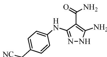
5-amino-3-((4-(cyanomethyl)phenyl)amino)-1 H -pyrazole-4-carboxamide
