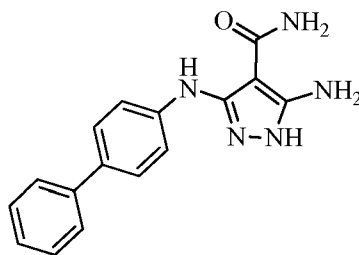
3-([1,1'-biphenyl]-4-ylamino)-5-amino-1 H -pyrazole-4-carboxamide
