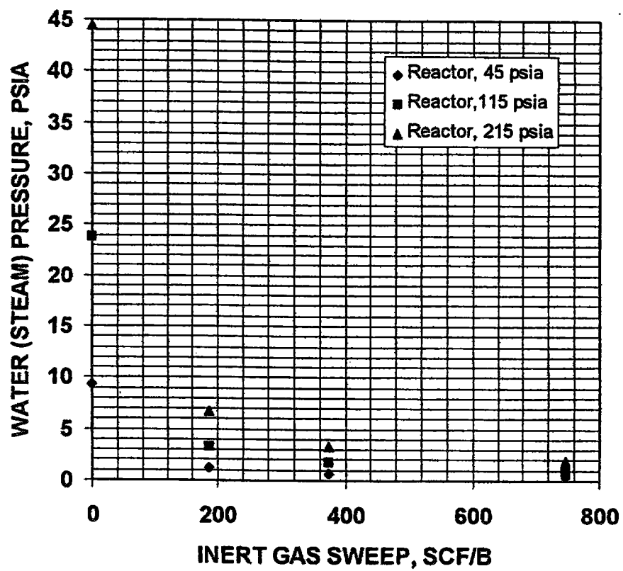
FIG. 1, WATER PRESSURE VS SWEEP RATE
