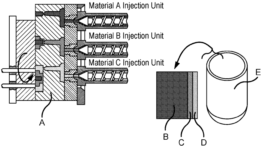
Sequential Injection Overmolding Schematic A - Sequential Injection Overmolding Unit B - Engineering Thermoplastic C - Thermoplastic Elastomer D - Fluoropolymer Resin E - Example Molded Capsule
