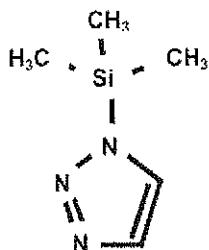
Trimethylsilyl-1,2,3-triazole
