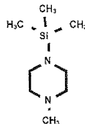
Trimethylsilyl-4-methylpiperazine
