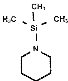
Trimethylsilylpiperidine
