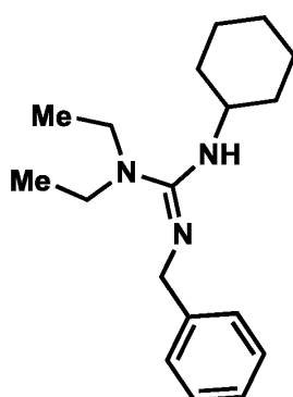
Ligand 1
