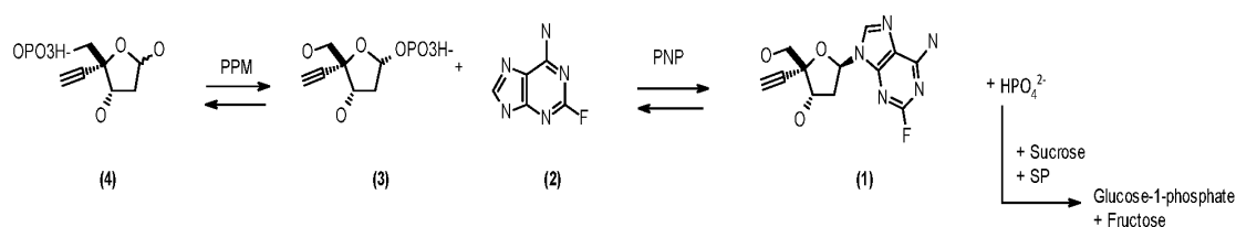
Scheme III. Overall Reaction Scheme to Produce Compound (1)
