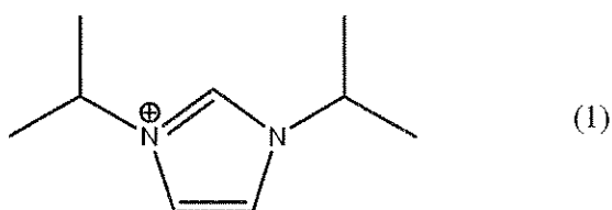
1,3-diisopropylimidazolium cation
