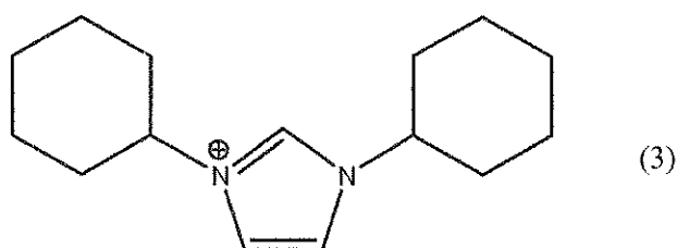
1,3-dicyclohexylimidazolium cation
