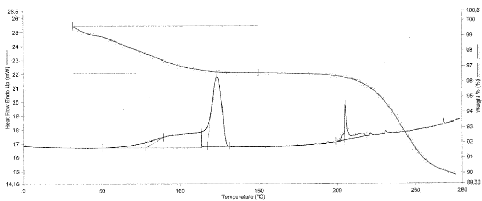
Fig. 29: DSC- and TGA-thermogram of the 1,25-Hydrate, example 6d
