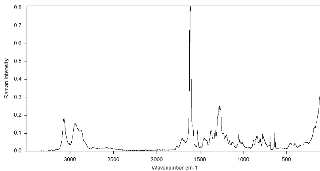
Fig. 18: Raman spectrum of the amorphous form, example 6g
