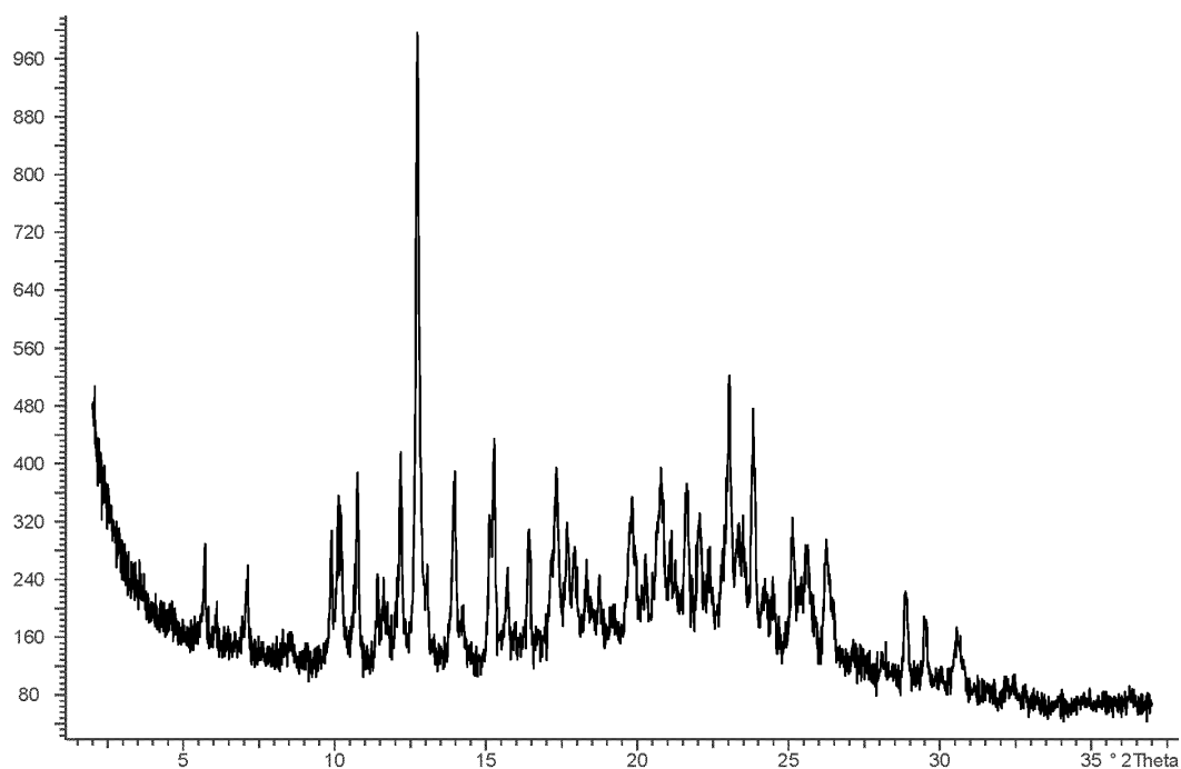
Fig. 40: X-Ray powder diffractogram of example 7 (storage stability): starting material for storage stability, monohydrate II
