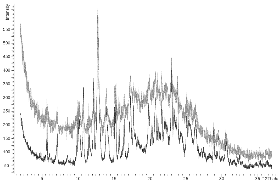
Fig. 42: Overlay of X-ray powder diffractograms of example 8b (micronization): starting material (monohydrate II) (bottom line) and material after micronization (monohydrate II with amorphous amounts, PTFE coated jet mill, 25°C) (top line)
