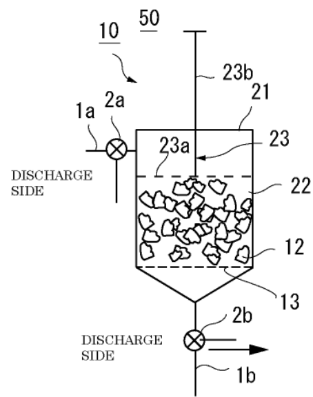
DRAINAGE DISCHARGE
