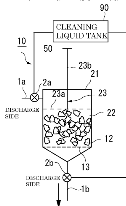
DRAINAGE DISCHARGE
