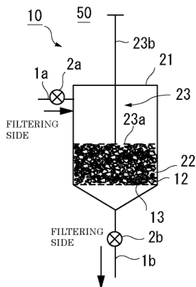
(b) FILTERING
