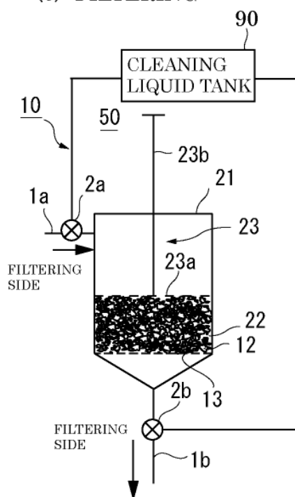
(c) FILTERING
