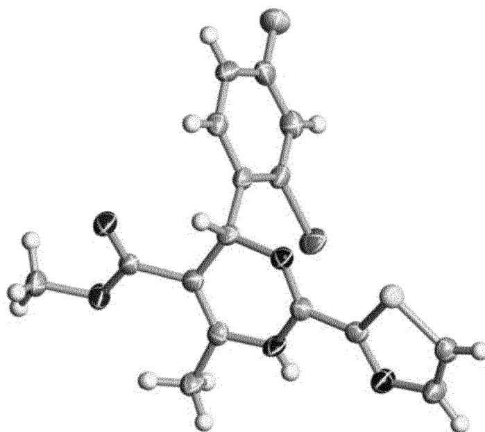
Figure 1: X-ray crystal structure of compound B1
